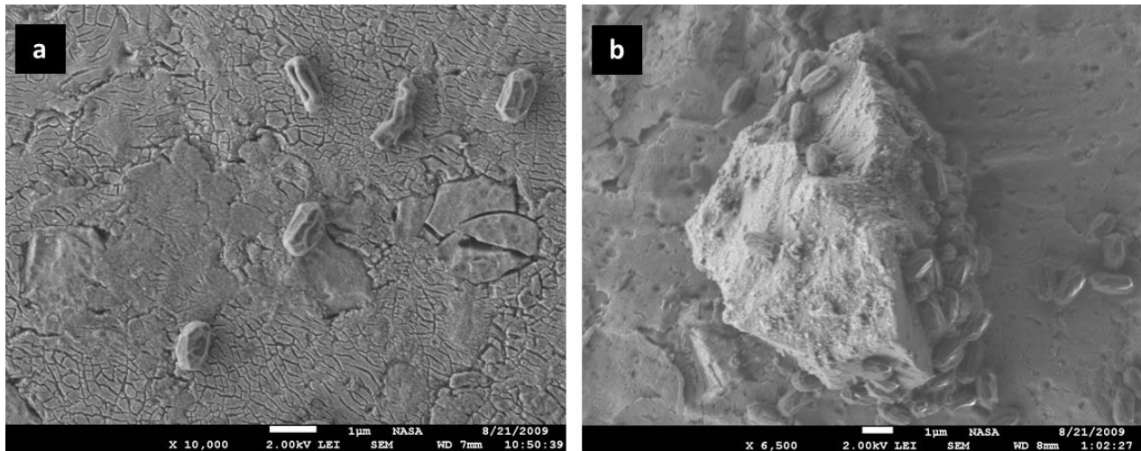
Figure 5.3 Scanning electron microscopy. Monolayers of dehydrated Bacillus subtilis spores (ovoid shaped, 1 µm) are visible on coupons used for experiments. Number of spores per coupon was estimated at 1 \times 10^6 . (A) Typical distribution of spores on dust-free coupon. (B) Example of dust treated coupon where spores can be seen attached to a prominent particle.
