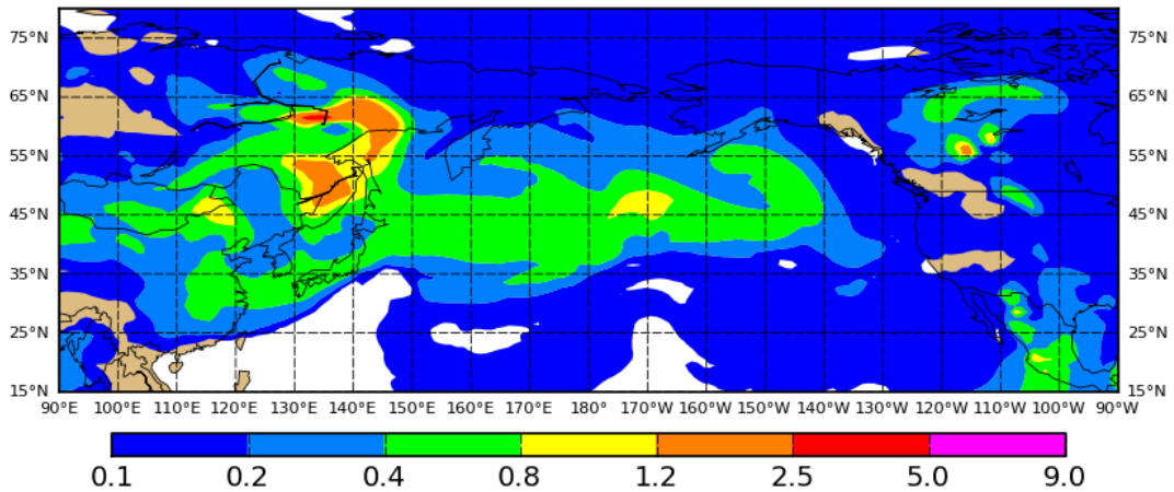
Figure S3.3 Transoceanic aerosol plumes modeled with the Navy Research Laboratory Aerosol Analysis and Prediction System (NAAPS). Total aerosol at optical depth 550 nm includes sulfate, smoke, dust, and sea salt mass concentrations. (a) Selected panel from 15 to 25 April 2011. (b) Selected panel from 7 to 17 May 2011.
