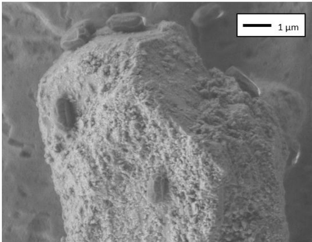
Figure 1.1 Tiny (1 \mu m) ovoid-shaped bacterial spores sampled from the atmosphere are attached to a large dust particle.
