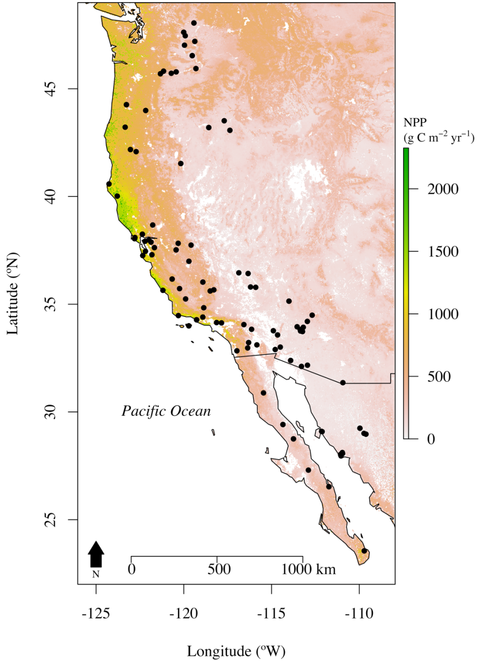
Figure 3.1. Collection localities for Pallid bat, Antrozous pallidus , specimens (black circles). Colors on the map represent mean annual net primary productivity ( \text{g C m}^{-2} \text{ year}^{-1} ), obtained as gridded data from the MODerate Resolution Imaging Spectroradiometer (MODIS) MOD17 land product dataset (see methods).
