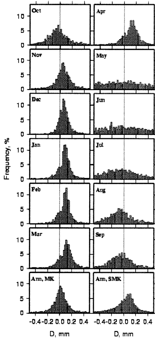
Figure 4.6 Histograms of the differences D_{ij} (MK statistics for individual months: "Oct" to "Sep"; and the MK statistic for annual streamflow: "Ann, MK") and D_{ijk} (for the SMK statistic: "Ann, SMK") used to determine the Mann-Kendall slope estimator B according to Hirsch et al. (1982), i.e. B is the median of the D_{ij} for MK and the D_{ijk} for SMK (see text for details). Results are shown for observed streamflow at the outlet of the Yenisei for the period of 1937 to 1998. Units are \text{mm month}^{-1} .
