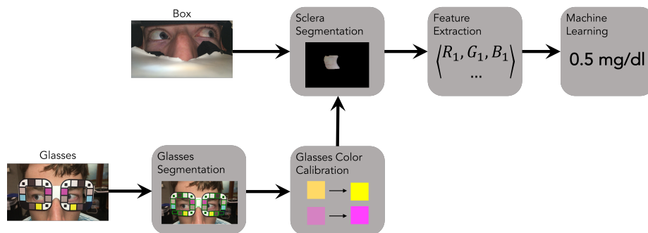
Figure 4.3: The algorithm pipeline for both BiliScreen accessories. Images from both the box and the glasses go through the same sclera segmentation, feature extraction, and machine learning steps (with their own respective models and small parameter changes). Images gathered with the glasses must go through the extra steps of glasses segmentation and color calibration.
