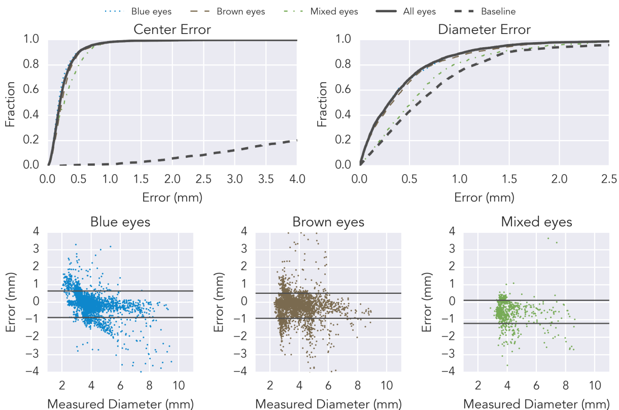
Figure 5.11: The accuracy results for the fully convolutional architecture. (top-left) The CDF of the pupil center prediction error. (top-right) The CDF of the pupil diameter prediction error. (bottom) Bland-Altman plots showing the residuals of the pupil diameter predictions split across the different iris colors: blue, brown, and mixed from left to right. The black lines indicate one standard deviation from the mean.
