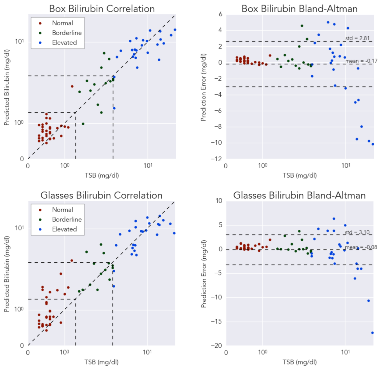
Figure 4.8: The (left) correlation and (right) Bland-Altman plots for BiliScreen’s bilirubin measurements with the (top) box and (bottom) glasses using the optimal sclera and glasses segmentation. Note that the axes of the correlation plot are both in log-scale, as is the x-axis of the Bland-Altman plot.
