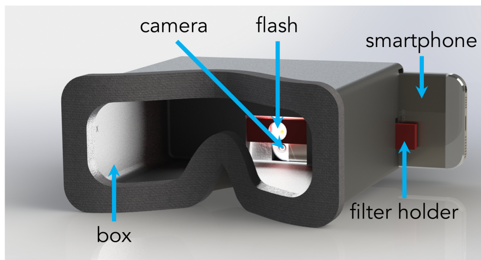
Figure 5.4: A 3D rendering of the PupilScreen box. The smartphone's flash lies in the horizontal center of the box. The box has a hole on the side so that a neutral density filter and a diffuser can be aligned with the flash using a sliding stick.
