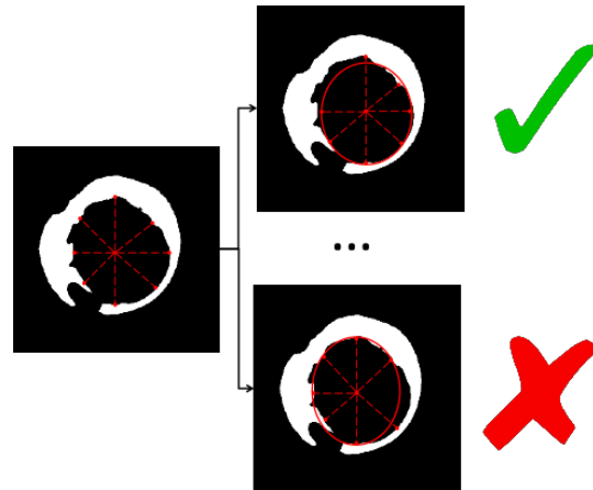
Figure 3.3: A variation of the Starburst technique by Li et al. [141] is used to estimate the innermost ellipse from a binary mask. After candidate points are selected from the inside, contiguous subsets of points are tested with least-squares ellipse fitting until the most circular is found.
