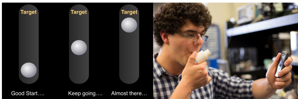
Figure 6.2: (left) As a person pushes more air out of their lungs, the ball in the SpiroSmart visualization rises to the top and encourages the user to continue the maneuver. (right) The SpiroSmart vortex whistle can be used to control the diameter of the user's mouth, acting as a flow-to-pitch transducer.
