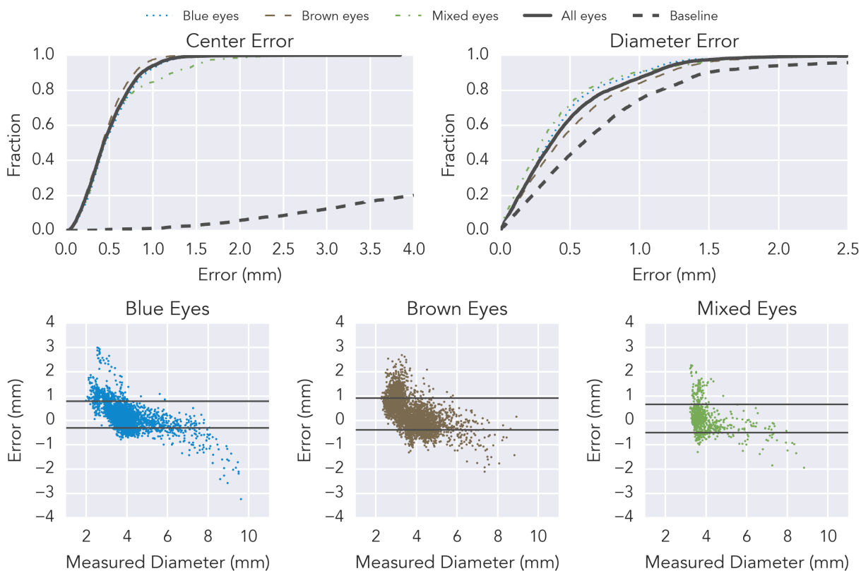
Figure 5.10: The accuracy results for the sequential network architecture. (top-left) The CDF of the pupil center prediction error. (top-right) The CDF of the pupil diameter prediction error. (bottom) Bland-Altman plots showing the residuals of the pupil diameter predictions split across the different iris colors: blue, brown, and mixed from left to right. The black lines indicate one standard deviation from the mean.
