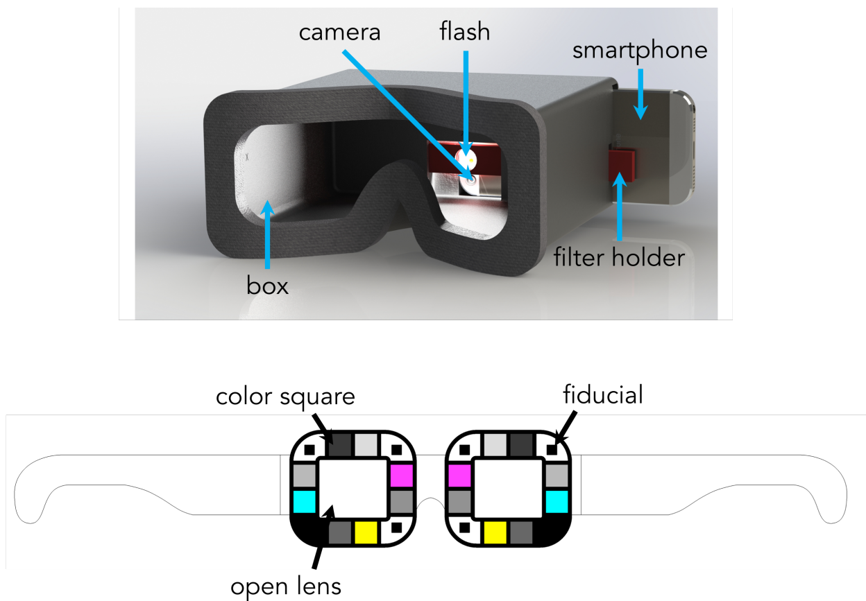
Figure 4.2: (top) A 3D rendering of the BiliScreen box. The smartphone's flash lies in the horizontal center of the box. The flash is covered with a neutral density filter and a diffuser to make the light more comfortable. (bottom) A rendering of the BiliScreen glasses.
