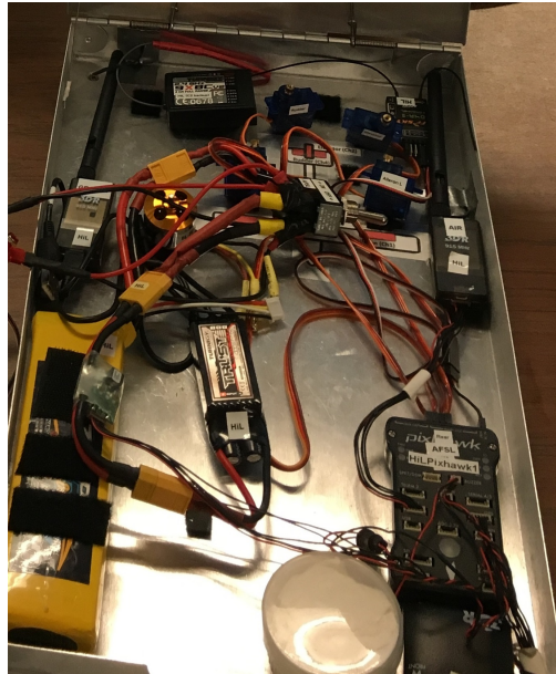
Figure 3.5: Secondary GPS HiL unit.
