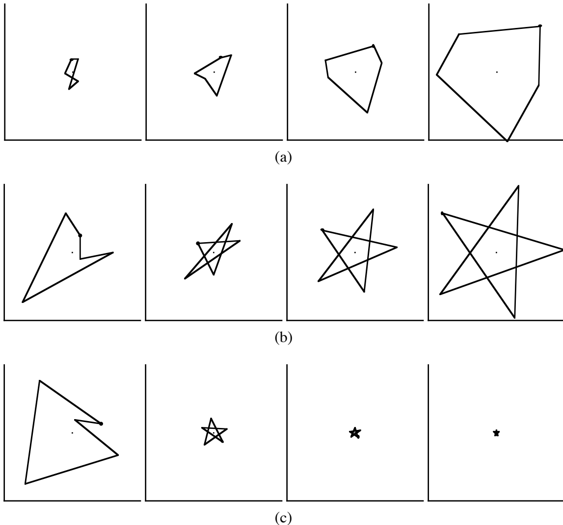
Figure N6.1. Iterations of the smoothing operation S(b) , with b = (1, -i/2, 0, 0, i/2) . The eigenvalues are \lambda_1 = 1.951056516 = \rho_1 ; \lambda_2 = 1.587785252 = \rho_2 ; \lambda_3 = 0.4122147477 = \rho_3 ; \lambda_4 = 0.0489434837 = \rho_4 , and \phi_d = 0 for all d . The starting pentagon in (a) has nontrivial regular (5/d) -components for all d ; the polygon in (b) is missing the (5/1) -component, while the one in (c) is missing both (5/1) - and (5/2) -components.
