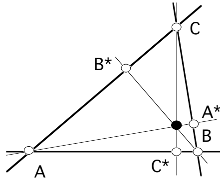
Figure 2.3. Notation for the proof of the existence of the orthocenter, the point of concurrence of the three altitudes.
