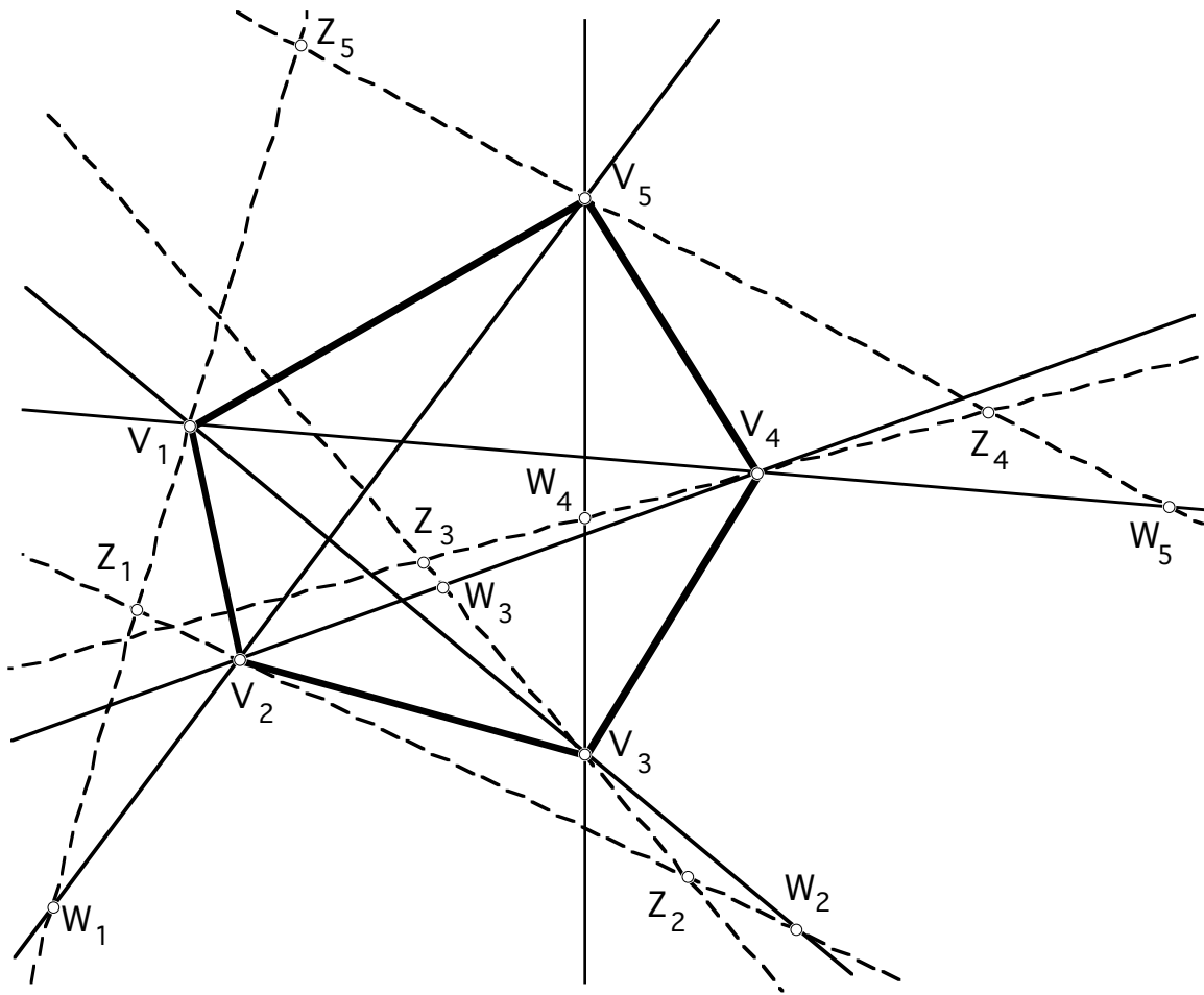
Figure 8.3. An illustration for n = 5 of Theorem 8.4.
