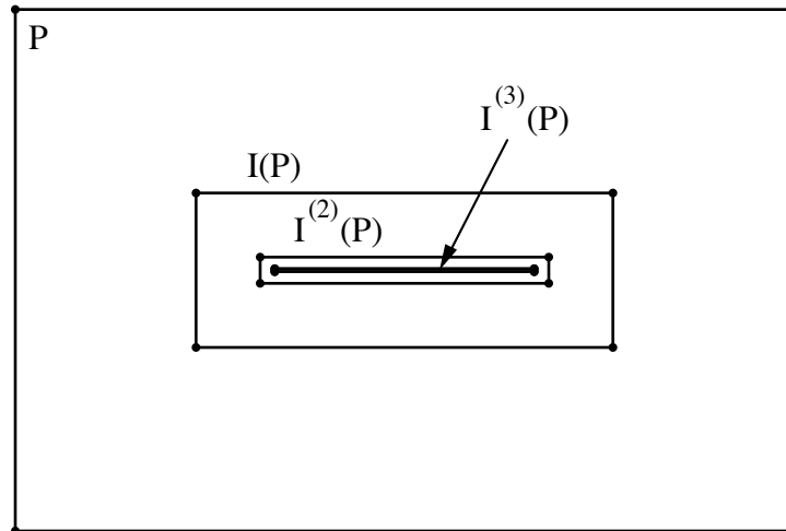
Figure N8.3. Iterations of the incenter transformation applied to a rectangle lead to rectangles which converge to a segment. All rectangles in the sequence have same difference of length of their sides.
