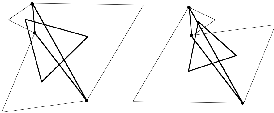
Figure 1.2. "Napoleon's theorem" starts with an arbitrary triangle and leads to two equilateral triangles.
