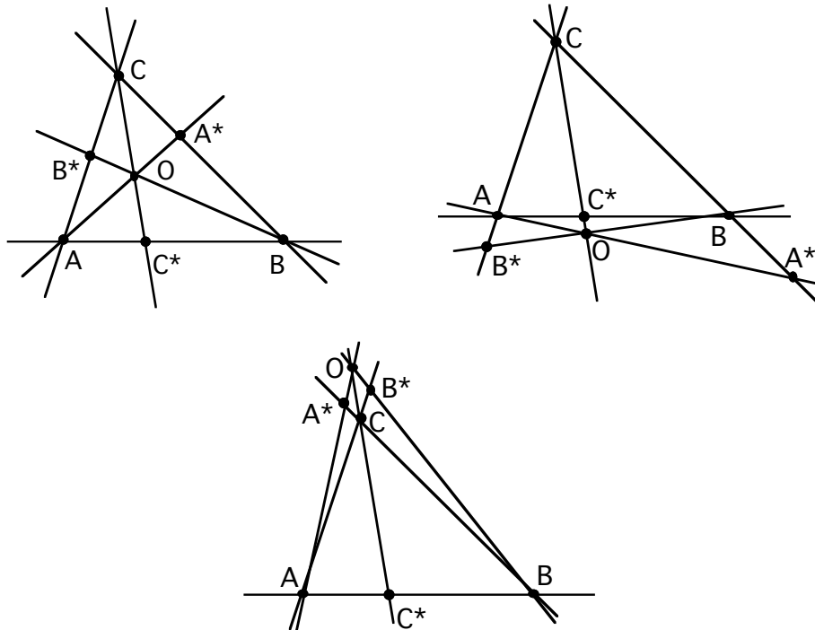
Figure 2.2. The three distinct positions of the point O of Ceva's theorem.
