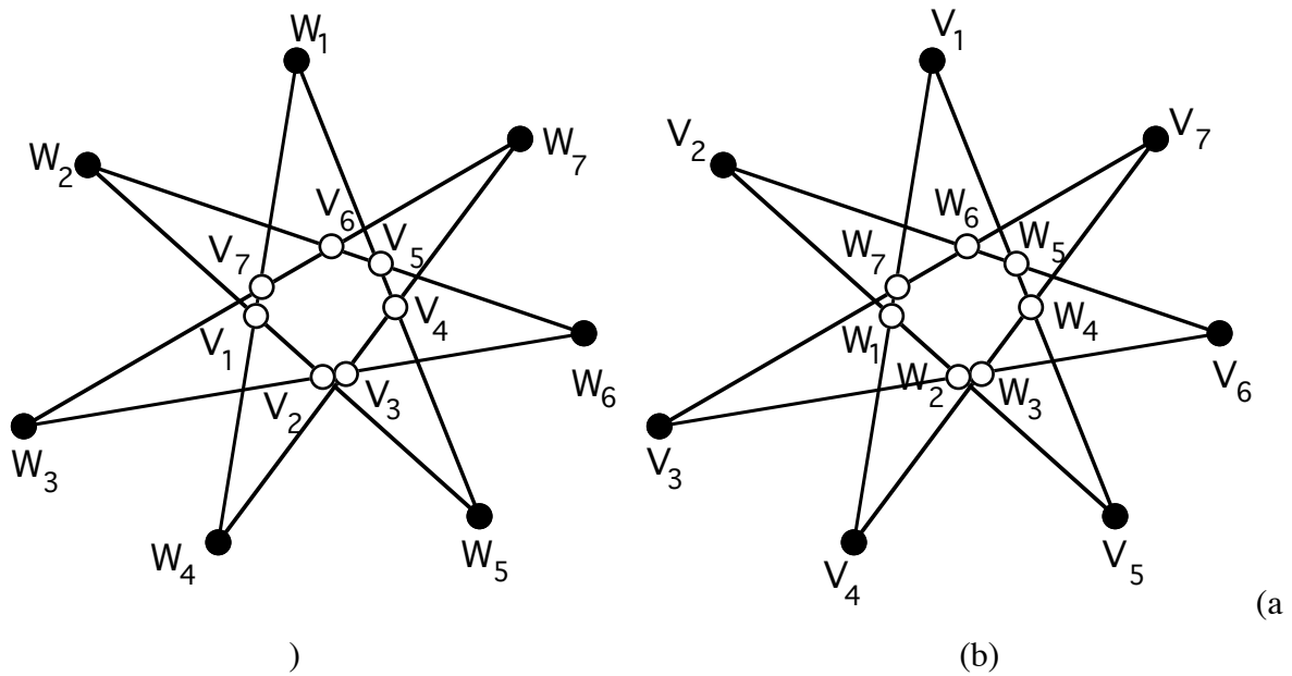
Figure 6.5. (a) Illustration of Hoehn's First Theorem for n = 7 , j = 3 . (b) Illustration of Hoehn's Second Theorem, with n = 7 , k = 3 .
