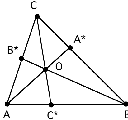
Figure 2.1. An illustration of Ceva's theorem: \frac{AC^*}{C^*B} \cdot \frac{BA^*}{A^*C} \cdot \frac{CB^*}{B^*A} = 1 if and only if the lines AA^*, BB^*, CC^* are concurrent.
