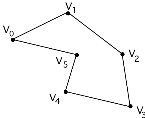
Figure N1.1. Notation for polygons and rooted polygons.
