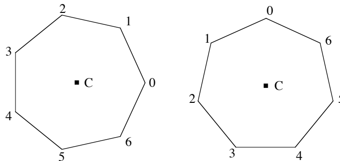
Figure N1.6. The two polygons that form an orthogonal basis of the space \mathbf{W}^O(5/1) .
