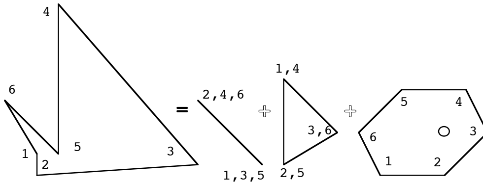
Figure N2.3. The decomposition of a hexagon into a vertex sum of three affinely regular hexagons, illustrating Corollary 3.3. For clarity, the origin has been moved away from the center of the hexagon that is being decomposed.
