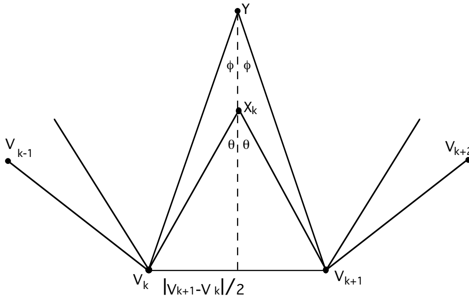
Figure N5.4. An illustration of the calculations in the proof of Theorem N5.3. The V 's are vertices of the regular (n/d_0) -gon R(n,d_0) , with center at Y . The point X_k is the center of the regular (n/d_j) -gon P_k which shares the edge [V_k, V_{k+1}] with R(n,d_0) . X_k is a vertex of \mathcal{T}_{n,d_j}(R(n,d_0)) .
