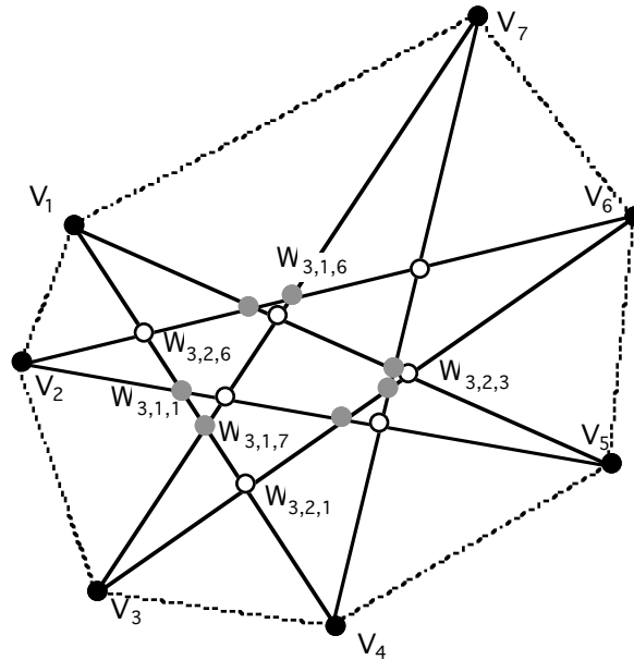
Figure 6.7. An illustration of the notation used for the result in (3) above.
