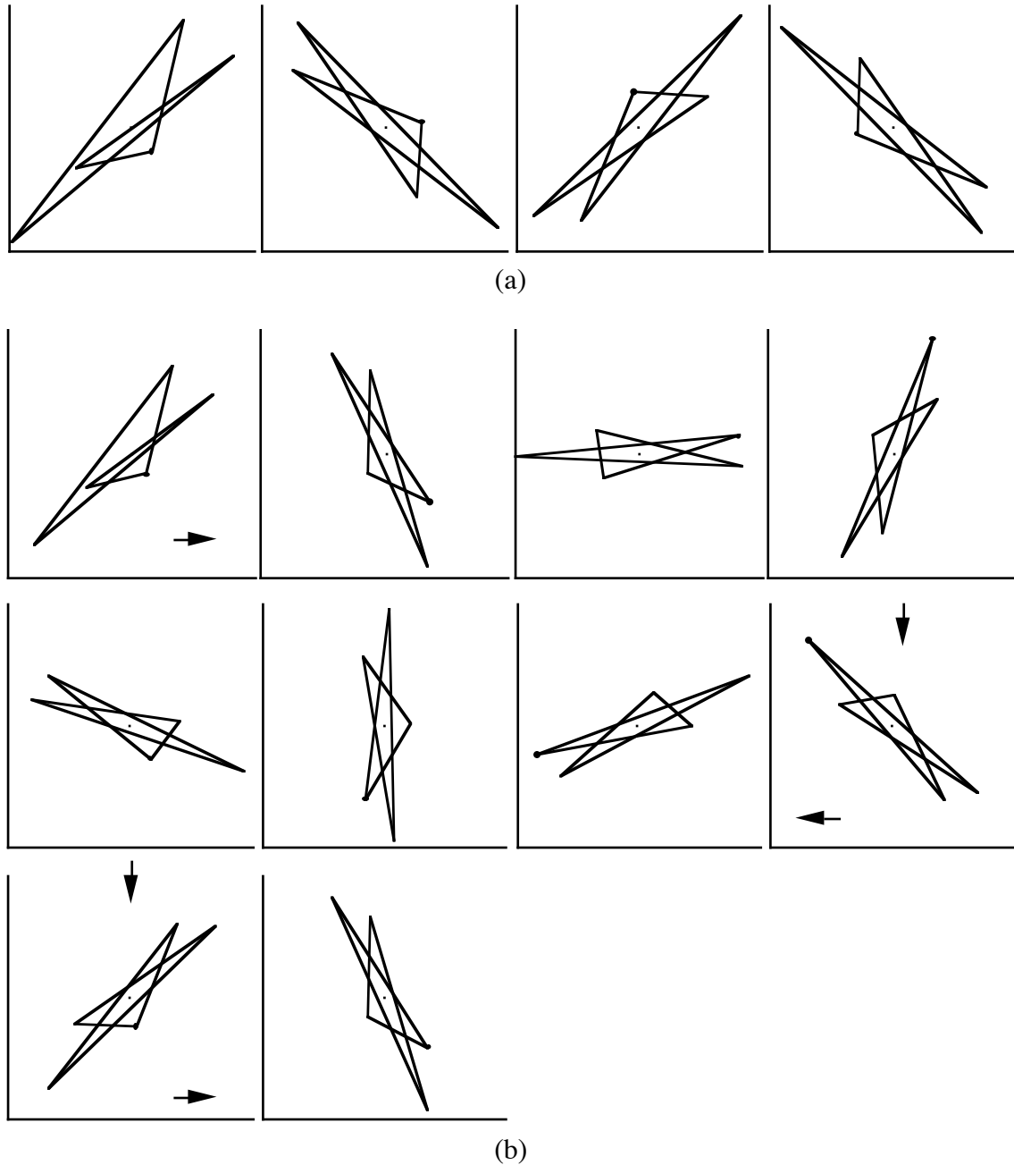
Figure N6.5. Two examples of smoothing operations periodic after the first iteration. The one in (a) has \lambda = (2, 2, i, i, 0) , while the one in (b) has \lambda = (2, 2, i, (1+i)/\sqrt{2}, 0) . The polygon is the same in both cases; it has trivial (5/1) -component, and all other components nontrivial. In both cases the (5/4) -component is annihilated in the first iteration, and the sequence of iterates is periodic. However, all these polygons (beyond the starting one) are congruent in (a), and the period is 4, while in (b) the period is 8 and the polygons within each period are noncongruent.
