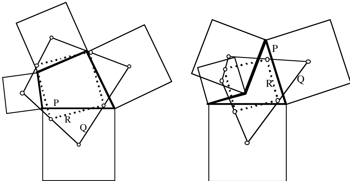
Figure N2.8. Starting from an arbitrary quadrangle P , the centers of the squares constructed on the edges of P are vertices of a quadrangle with the property that the midpoints of its edges are vertices of a square.
