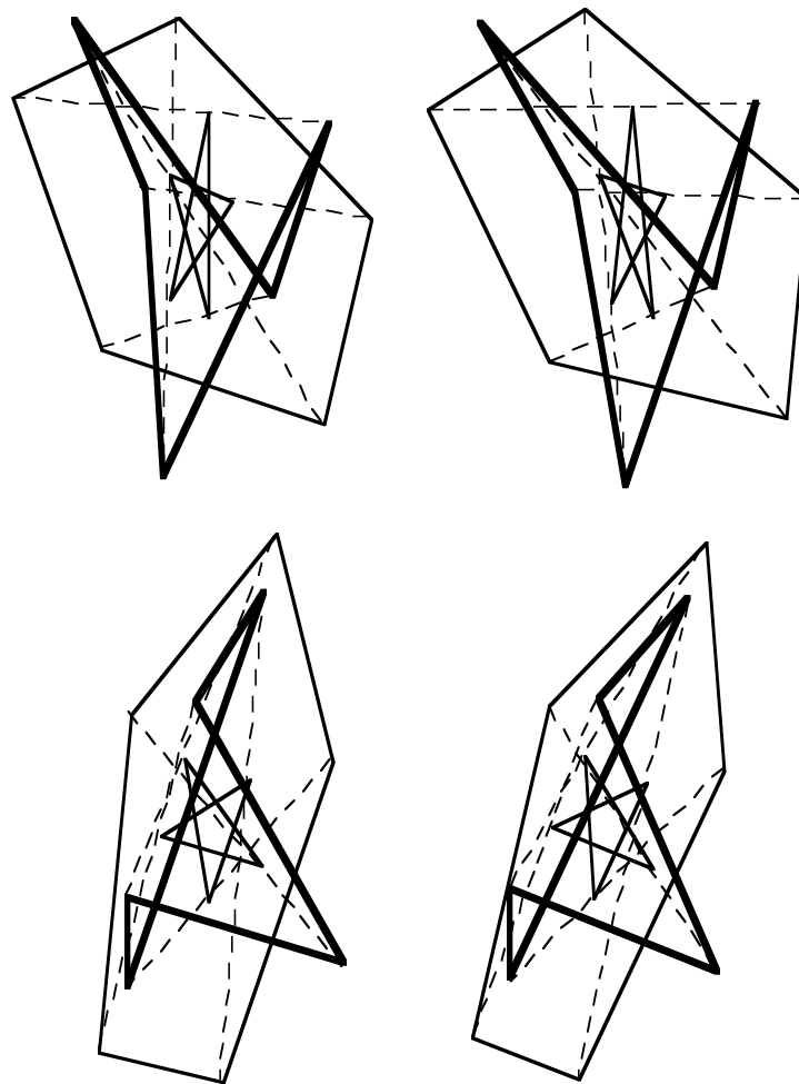
Figure N7.2. Two examples (each in stereoscopic pairs) of the two affine-regular pentagons associated with each pentagon in \mathbf{E}^3 by the method of Douglas and Schoenberg. The original pentagon in each example is shown in heavy lines, the affine-regular ones in thin lines. The collinearities mentioned in the text are indicated by the dashed lines.
