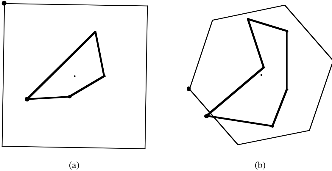
Figure N3.3. Examples of the action of some strictly regularizing vectors. In (a) the strictly (4/1)-regularizing vector is (1-i, -1-i, -1+i, 1+i)/2 , and in (b) the strictly (6/1)-regularizing vector is (3-i\sqrt{3}, -2i\sqrt{3}, -3-i\sqrt{3}, -3+i\sqrt{3}, 2i\sqrt{3}, 3+i\sqrt{3})/12 .
