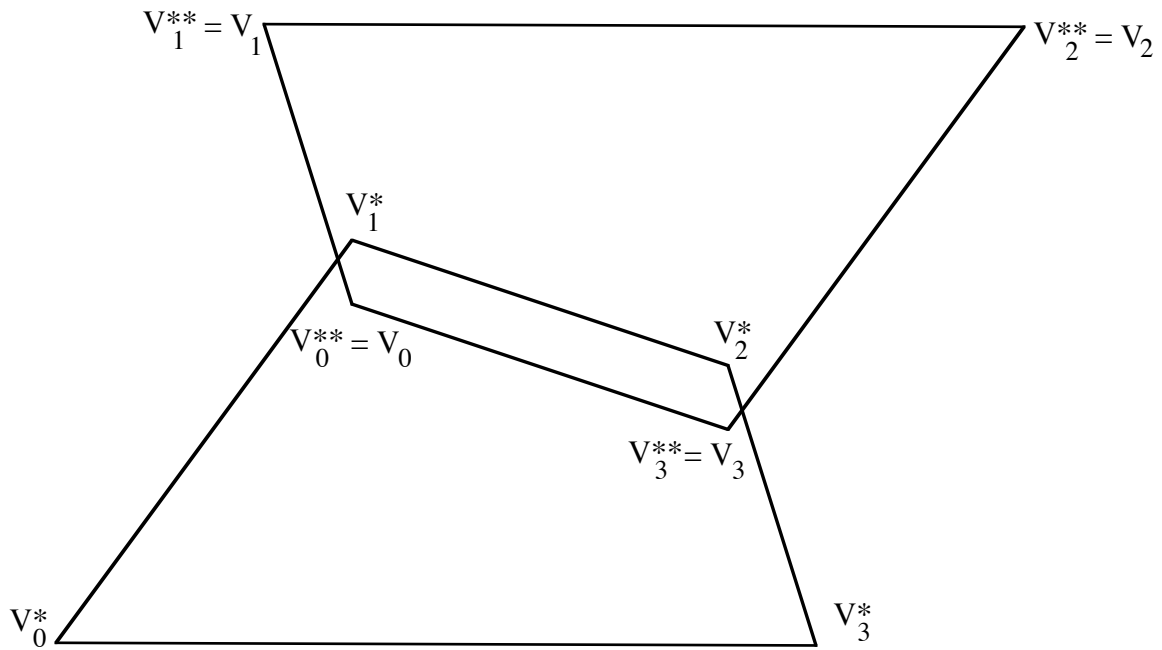
Figure N8.6. An example of a quadrangle P which is congruent to O(P) . The vertices have coordinates (0.3194, 2.5694), (3.5227548996, 2.55560034), (2.2778, 0.8611), (0.6944, 1.3889) . The maximal distance between vertices of P and the corresponding vertices of O(P) is less than 1.5 \cdot 10^{-10} . This was the limit of my patience in minimizing this distance, but there is no doubt that it can be reduced to 0 by suitably adjusting any one of the vertices of P .
