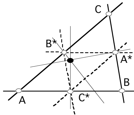
Figure 2.4. Notation for the proof of the existence of the circumcenter of \triangle ABC , which coincides with the orthocenter of \triangle A^*B^*C^* .
