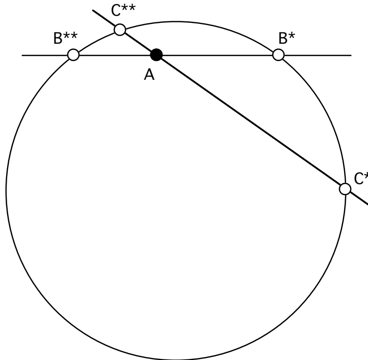
Figure 9.2. An illustration of the "power of a point with respect to a circle" theorem. The point A common to the two transversals may just as well be on the circle, or outside of it.
