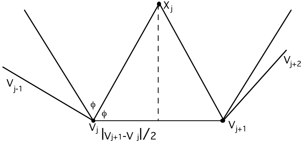
Figure N5.3. The calculation of the smoothing vector b corresponding to the operation \mathcal{T} (n,d) . Here \phi = \pi(n - 2d)/2n is half the angle at the vertex of a regular (n/d) -gon and |X_j V_j|/|V_{j+1} V_j| = 1/(2 \cos \phi) .
