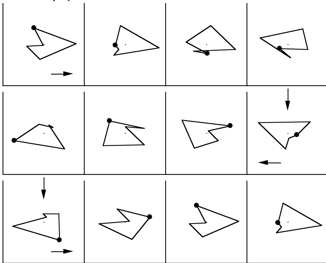
Figure N6.13. The operation determined by the smoothing vector b = (0, 0.7236067977, -0.2763932022, 0, -0.4472135955) is periodic with period 10 for every pentagon.
