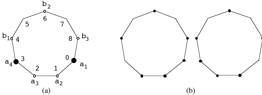
Figure 5.1. (a) An AB-diagram for n = 9 , with A = (0,1,2,3) and B = (4,6,8) . Here s = 3 and r = 2 . Because the two sets of points marked in (b) are directly congruent, the sets A and B satisfy the condition of the Transversality Theorem.
