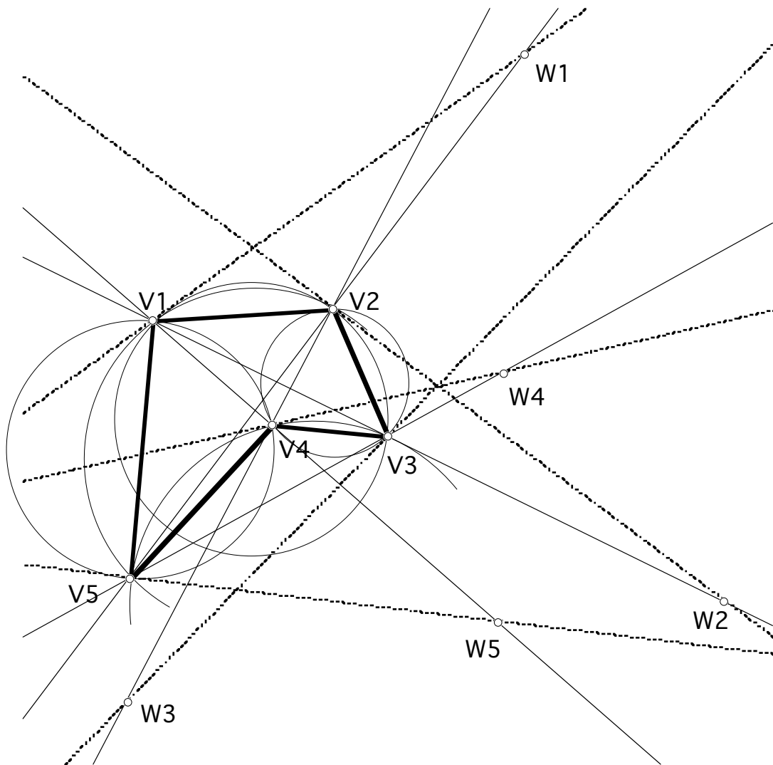
Figure 8.1. An illustration of Theorem 8.1, for n = 5 .
