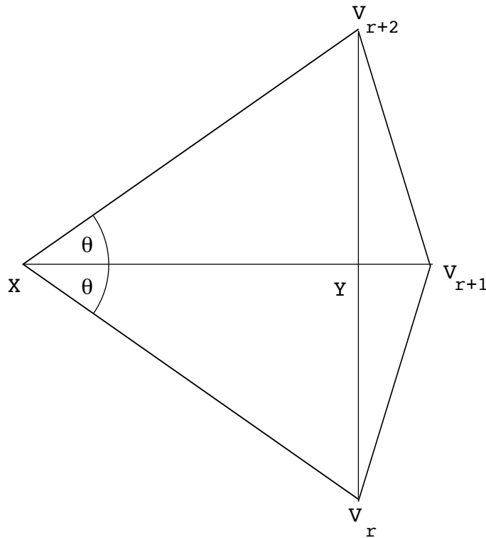
Figure N3.4. V_r, V_{r+1}, V_{r+2} are three consecutive vertices of an (n/d) -gon centered at X , and \theta = 2\pi d/n . This diagram is used in establishing equation (2) and thereby constructing an (n/d) -centralizing vector.
