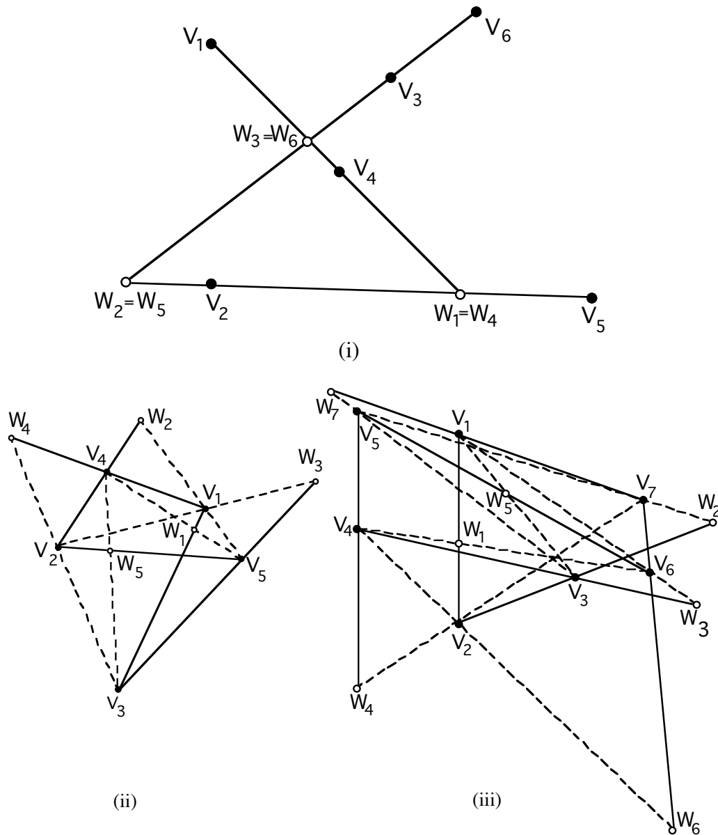
Figure 4.3. Three examples illustrating the Selftransversality Theorem. The product of the appropriate ratios is 1 in (i), and -1 in (ii) and (iii). To avoid clutter, all lines have been clipped as much as possible.
