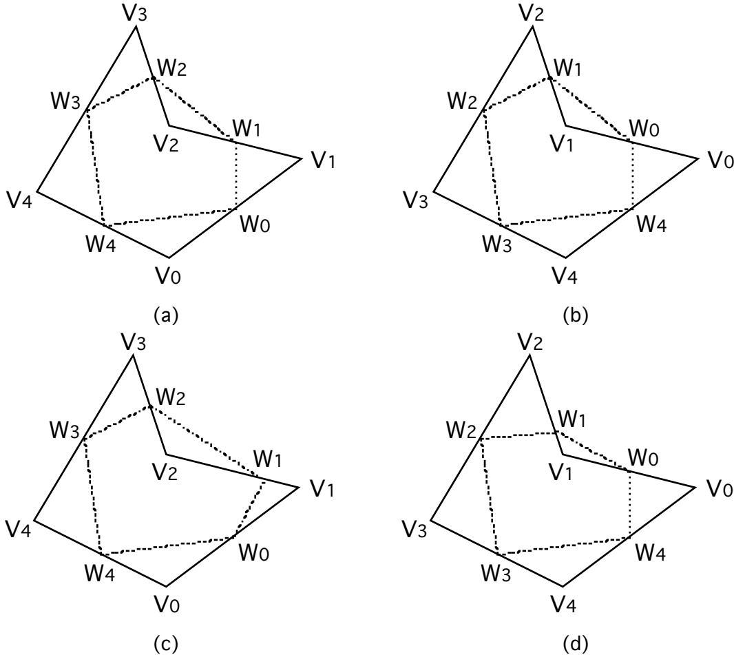
Figure N3.1. The rooted polygon Q = (W_0, W_1, W_2, W_3, W_4) is the image of the rooted polygon P = (V_0, V_1, V_2, V_3, V_4) under a linear transformation. The transformation in parts (a) and (b) is the smoothing transformation S(b) determined by the smoothing vector b = (1/2, 1/2, 0, 0, 0) ; these terms are explained in the text. The polygons P and Q in part (b) arise from polygons with the same name in part (a) by the transformation \zeta which advances the root vertex to the second vertex of the original polygon. Since S(b) is a smoothing operation, its action on the (unrooted) polygons is the same in parts (a) and (b). In contrast, the transformation used in (c) and (d) is not a smoothing transformation, since its matrix differs from that of S(b) by having the first row (4/3, 1/4, 0, 0, 0) , making it a noncirculant matrix. The transformation is not determined on the unrooted polygons.
