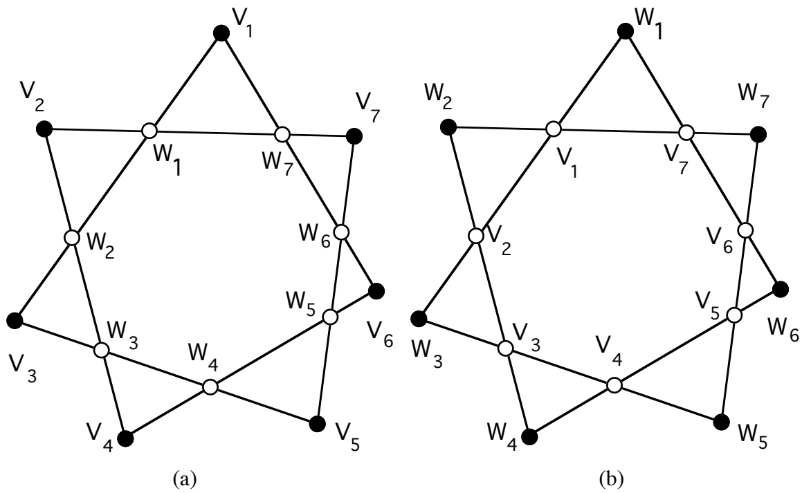
Figure 6.3. (a) Illustration of Hoehn's First Theorem for n = 7, j = 1 . (b) Illustration of Hoehn's Second Theorem, with n = 7, k = 1 .
