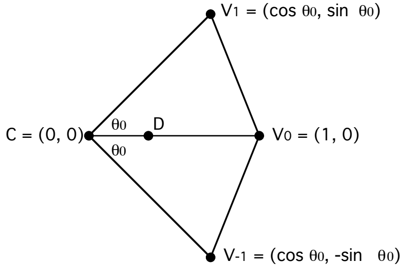
Figure N4.1. An illustration of the calculation of the coefficient of homothety \lambda(n,d,d_0) using three adjacent vertices of the regular (n/d_0) -gon; here \theta_0 = 2\pi d_0/n . The point D = (V_{-1} - 2 \cos \theta V_0 + V_1)/(2 - 2 \cos \theta) , with \theta_0 = 2\pi d/n , is the vertex of the affine-regular (n/d_0) -gon Q that corresponds under S(b_{n,d}) to the vertex V_0 of the standard regular (n/d_0) -gon R_{n,d} ; hence \lambda(n,d,d_0) = |C,V_0|/|C,D| , as used in the proof.
