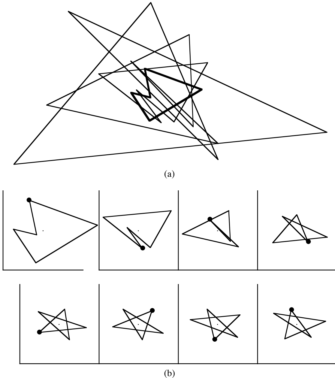
Figure N6.10. The action of the tangent map, determined for pentagons by b = (-1, 1, 0, 0, 0) , on a pentagon with both affine components nontrivial. (a) shows the first three iterates, and (b) shows the first seven iterates of the scaled transformation, for which the smoothing vector is (-1, 1, 0, 0, 0)/1.9021130\dots . Since the ratio \rho_1/\rho_2 = 0.61803399\dots is not very small, the (5/1) -component is eliminated only gradually. The sequence of scaled iterates is co-convergent with the affine (5/2) -component, which affinely rotates through an angle of 162^\circ at each step, and is therefore periodic with period 10.
