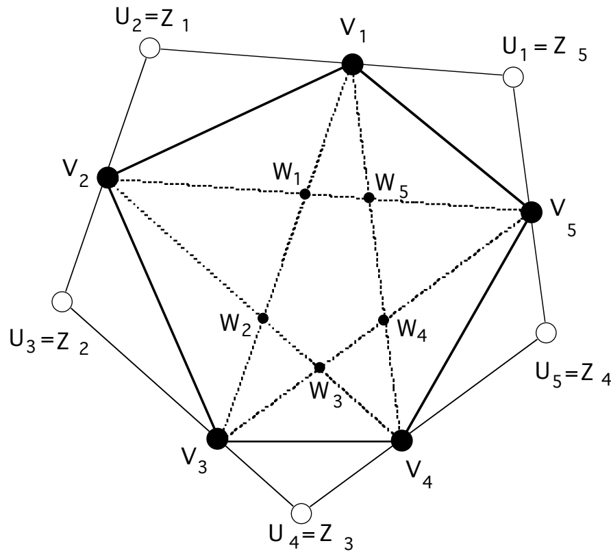
Figure 6.6. The illustration of the result attributed to Pratt and Kasapi by Chou [1988].
