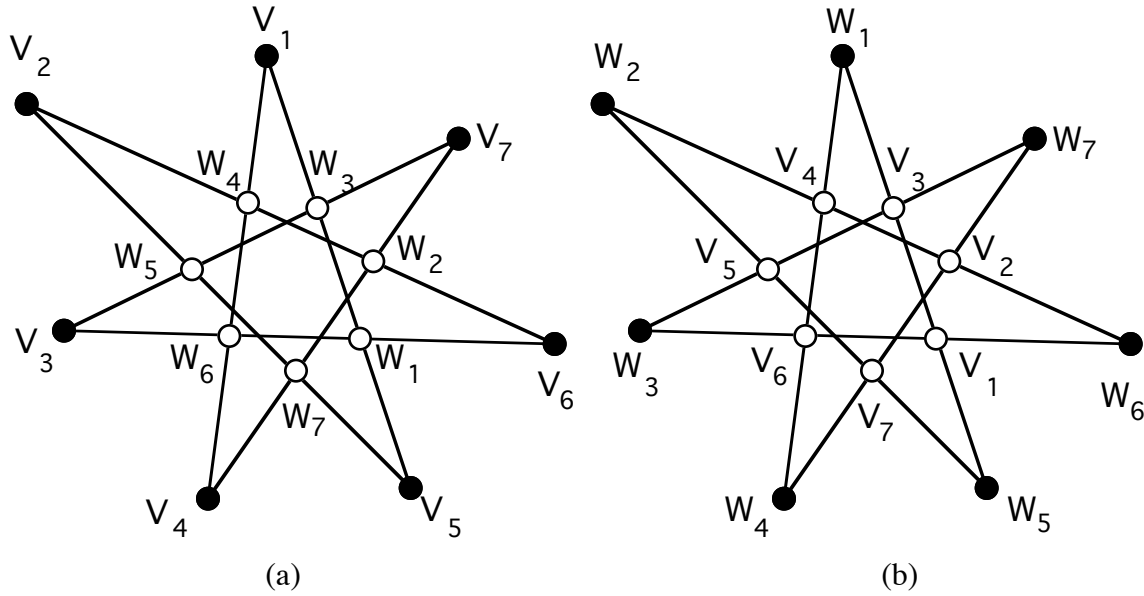
Figure 6.4. (a) Illustration of Hoehn's First Theorem for n = 7 , j = 2 . (b) Illustration of Hoehn's Second Theorem, with n = 7 , k = 2 .
