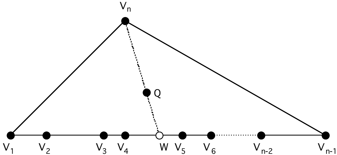
Figure 7.1. An example of an n -acron used in the proof of the Complete Ceva Theorem.
