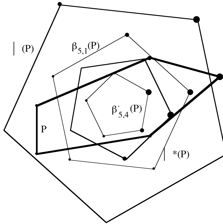
Figure N2.7. An illustration of the relationship between the regular components of an affinely regular polygon, and its Napoleon-Barlotti polygons.
