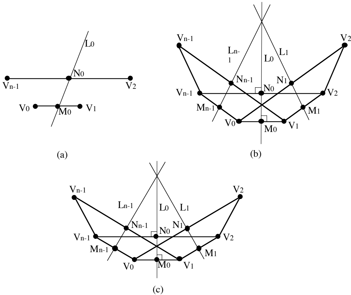
Figure N2.4. Illustration of the arguments used in the proof of Theorem N2.2.
