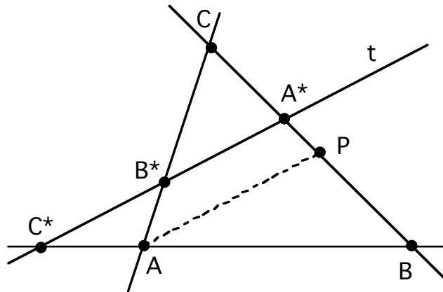
Figure 2.6. An illustration of the theorem of Menelaus and its proof.
