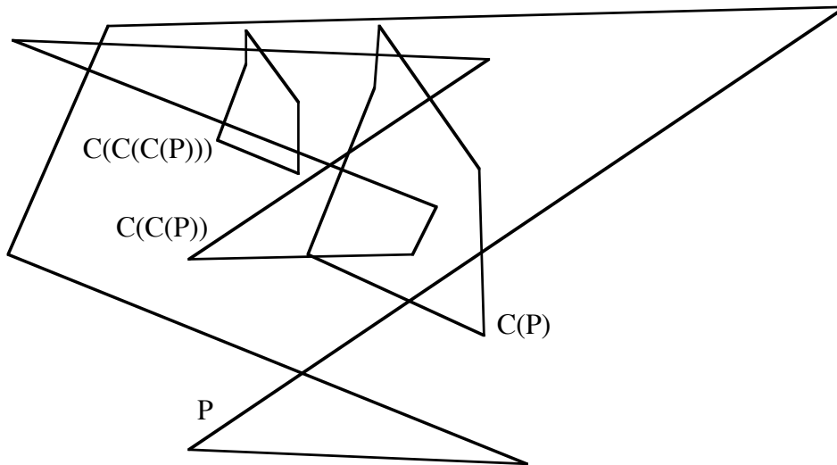
Figure N8.10. An illustration of the homothety between C(P) and C(C(C(P))) for a pentagon P . In general, a pentagon P is not homothetic to C(C(P)) .
