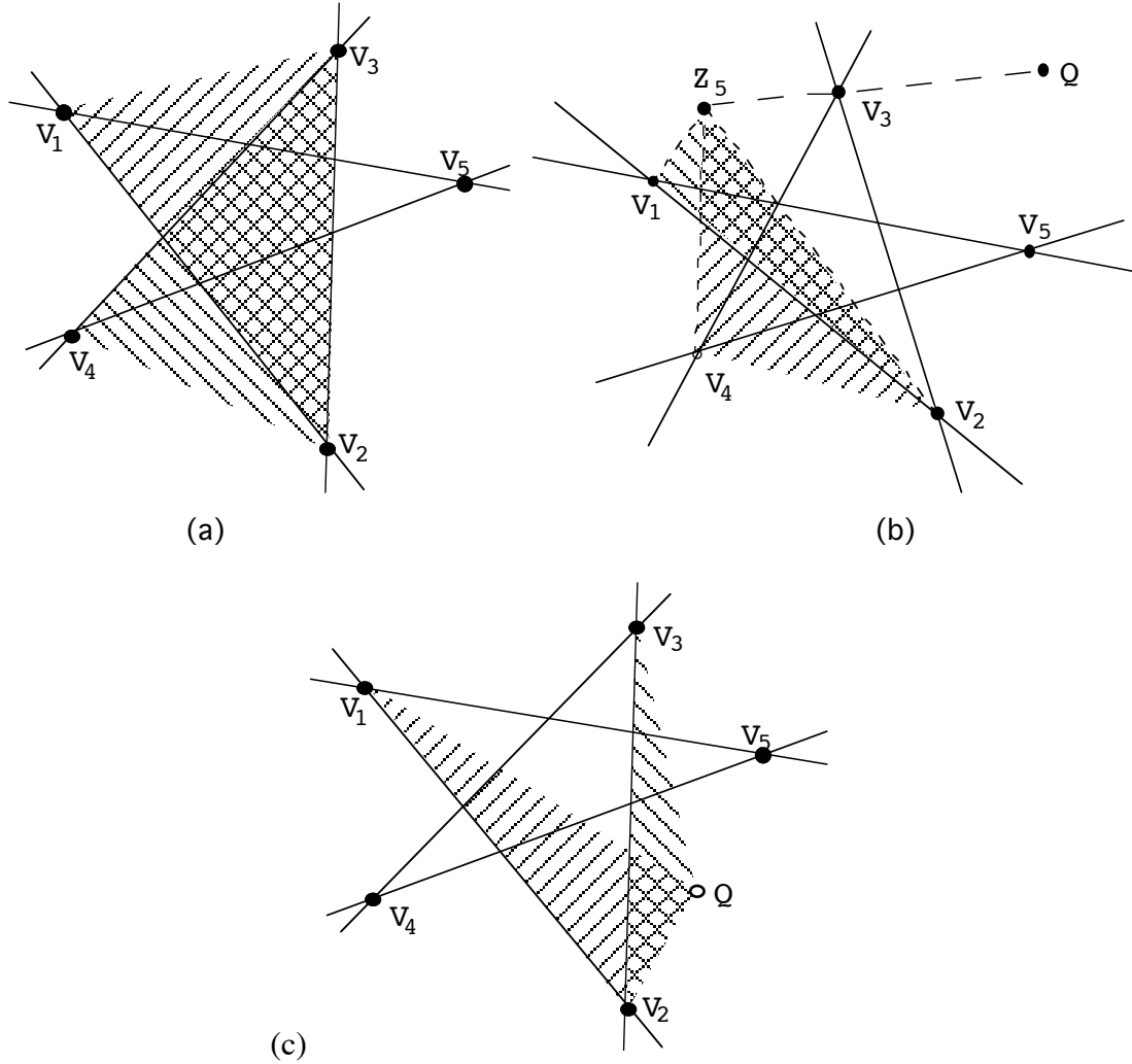
Figure 5.2. Three illustrations of the Transversality Theorem.
