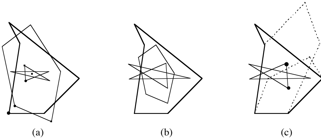
Figure N4.2. Comparison, as explained in the text, of (a) the affine-regular components of a pentagon, to (b) the affine-regular polygons, homothetic to these components, which result by applying the smoothing operations determined by the vectors b_{n,d} . The alternative interpretation of the latter, explained in Theorem N4.3, is indicated by the dotted lines in (c). In order to avoid clutter, only two of the affine-regular (5/1) -gons are shown in (c), and their centers — which are vertices of the resulting affinely regular (5/2) -gon — are indicated by the solid dots.
