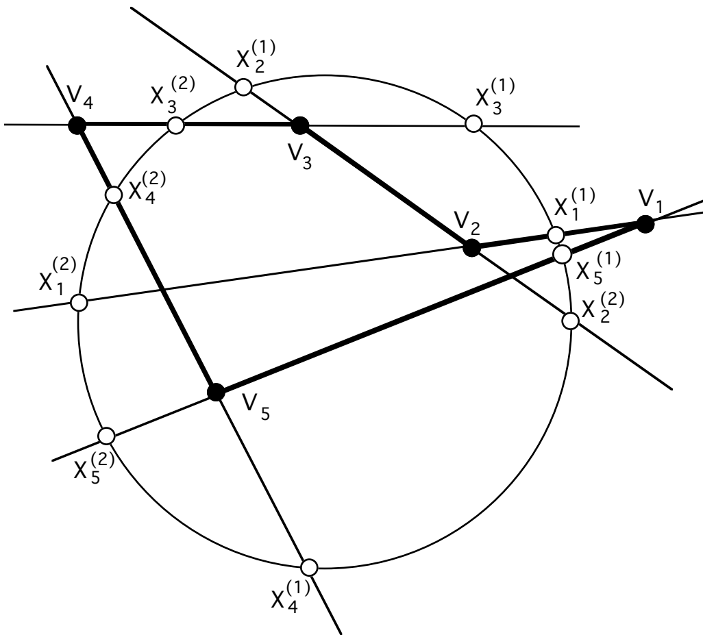
Figure 9.1. An illustration of Theorem 9.1 in case n = 5 .
