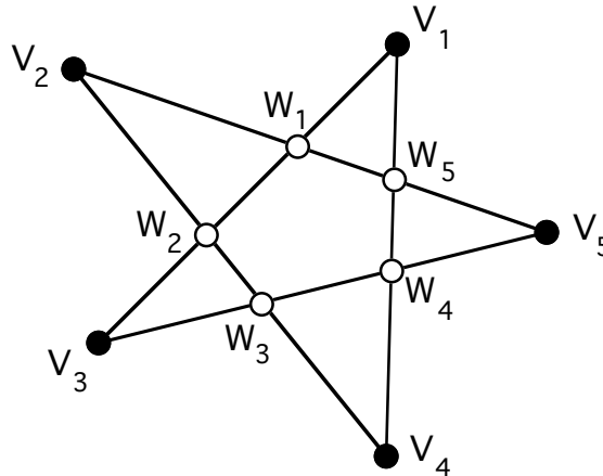
Figure 6.2. An illustration of Hoehn's theorems.
