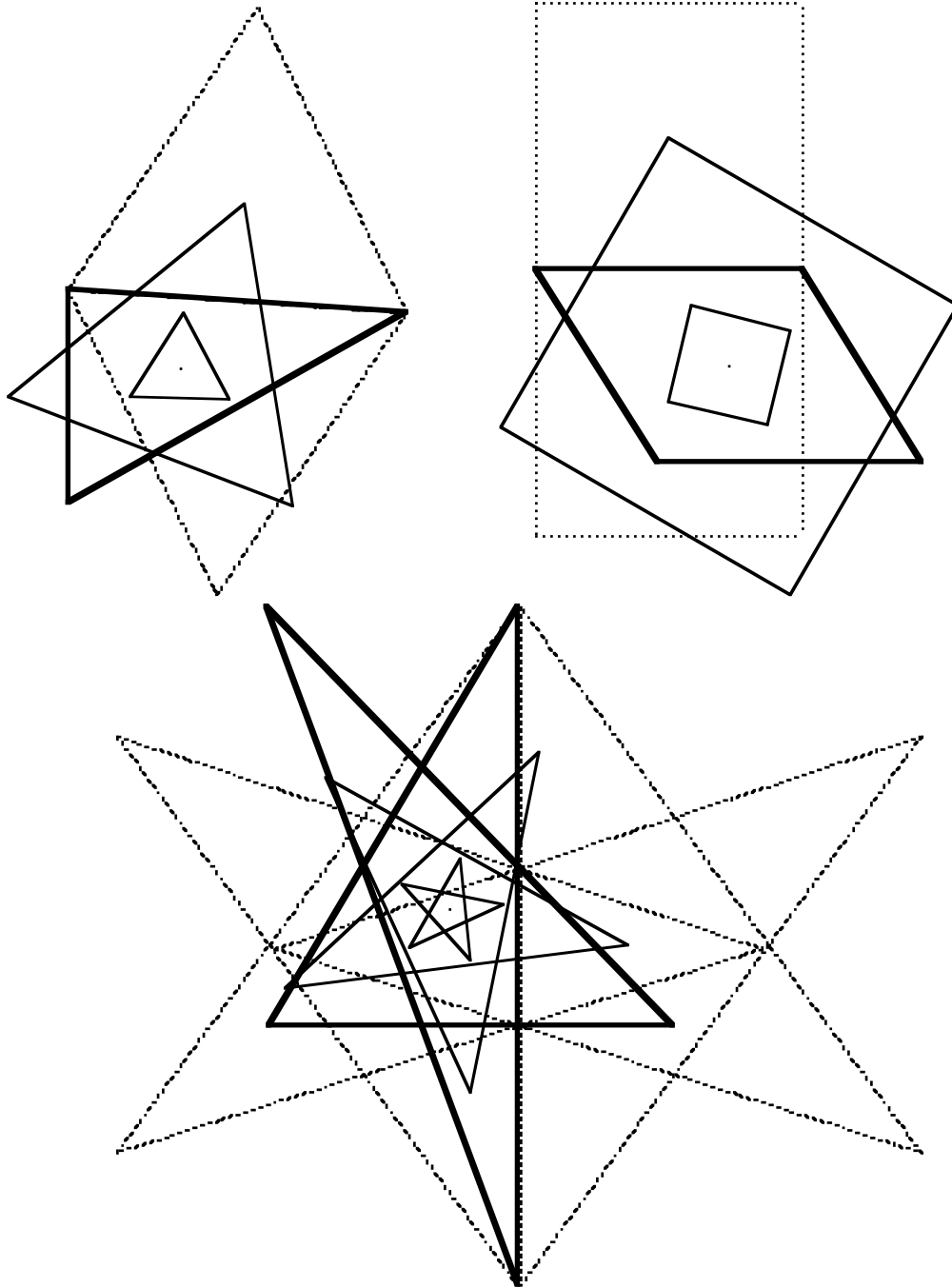
Figure N2.6. Three illustrations of the Napoleon-Barlotti theorem. The given affinely regular polygon P is shown by heavy lines, and the polygons \mathcal{B}(P) and \mathcal{B}^*(P) are shown by thin lines. The dotted lines indicate the regular polygons constructed on the edges of P ; to avoid clutter, only one such polygon is shown in each case.
