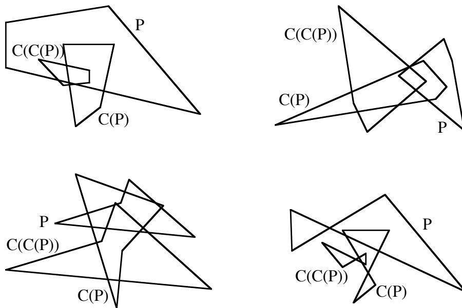
Figure N8.8. Illustrations of the homothety between a quadrangle P and its image C(C(P)) .
