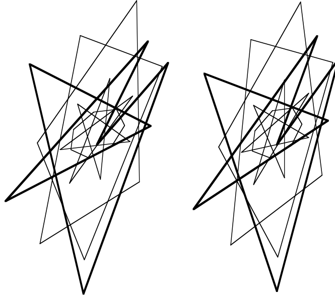
Figure N7.3. A heptagon, and the three affine-regular heptagons associated with it by the construction of Schoenberg.
