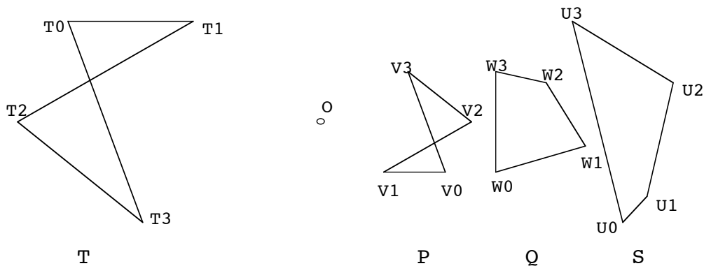
Figure N1.2. Illustrations of the vertex sum and scalar multiplication of rooted polygons. Here \mathbf{S} = \mathbf{P} \oplus \mathbf{Q} , and \mathbf{T} = -2\mathbf{P} .
