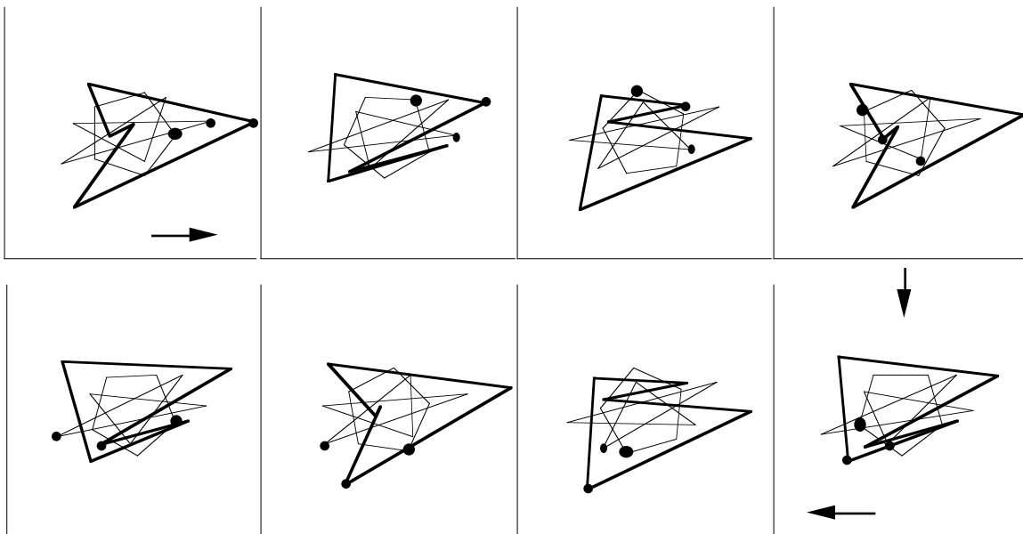
Figure N6.11. Iteration of the map S(b) with b = (1 + \tau, 1, \tau, 0, 0) where \tau = (1 + \sqrt{5})/2 = 1.618033989\dots is the golden section, scaled appropriately, acting on a pentagon P . For the rescaled smoothing vector \rho_1 = \rho_2 = 1 therefore both affine components of P retain their size. The affine rotations are \phi_1 = 49.61382244\dots^\circ and \phi_2 = -22.38617756\dots^\circ ; they appear to be incommensurable with 360^\circ and with each other, hence all iterated pentagons have affinely unrelated shapes.
