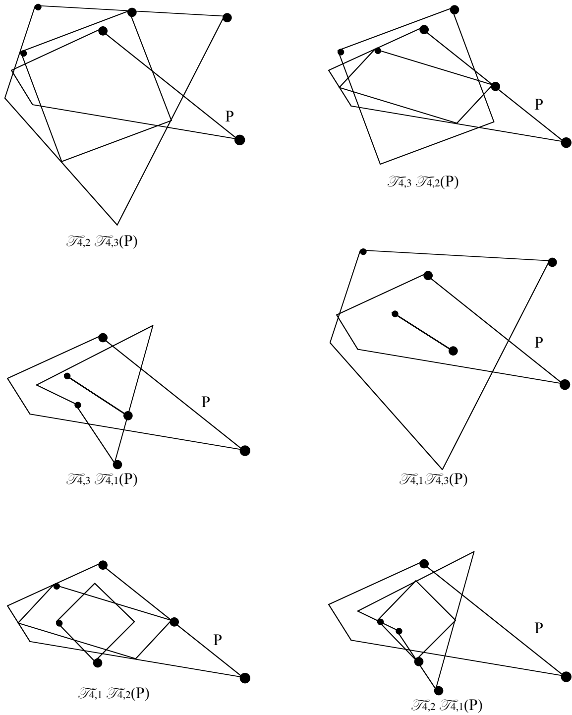
Figure N5.2. Six essentially different instances of Napoleon's theorem, applied to a quadrangle P . To avoid clutter, the regular polygons R(4,1) and R(4,3) used in the construction are not shown. The orientation of each quadrangle is indicated by the transition from the large dot to the mid-sized dot. The three constructions in each column give the three symmetric components of the quadrangle P .
