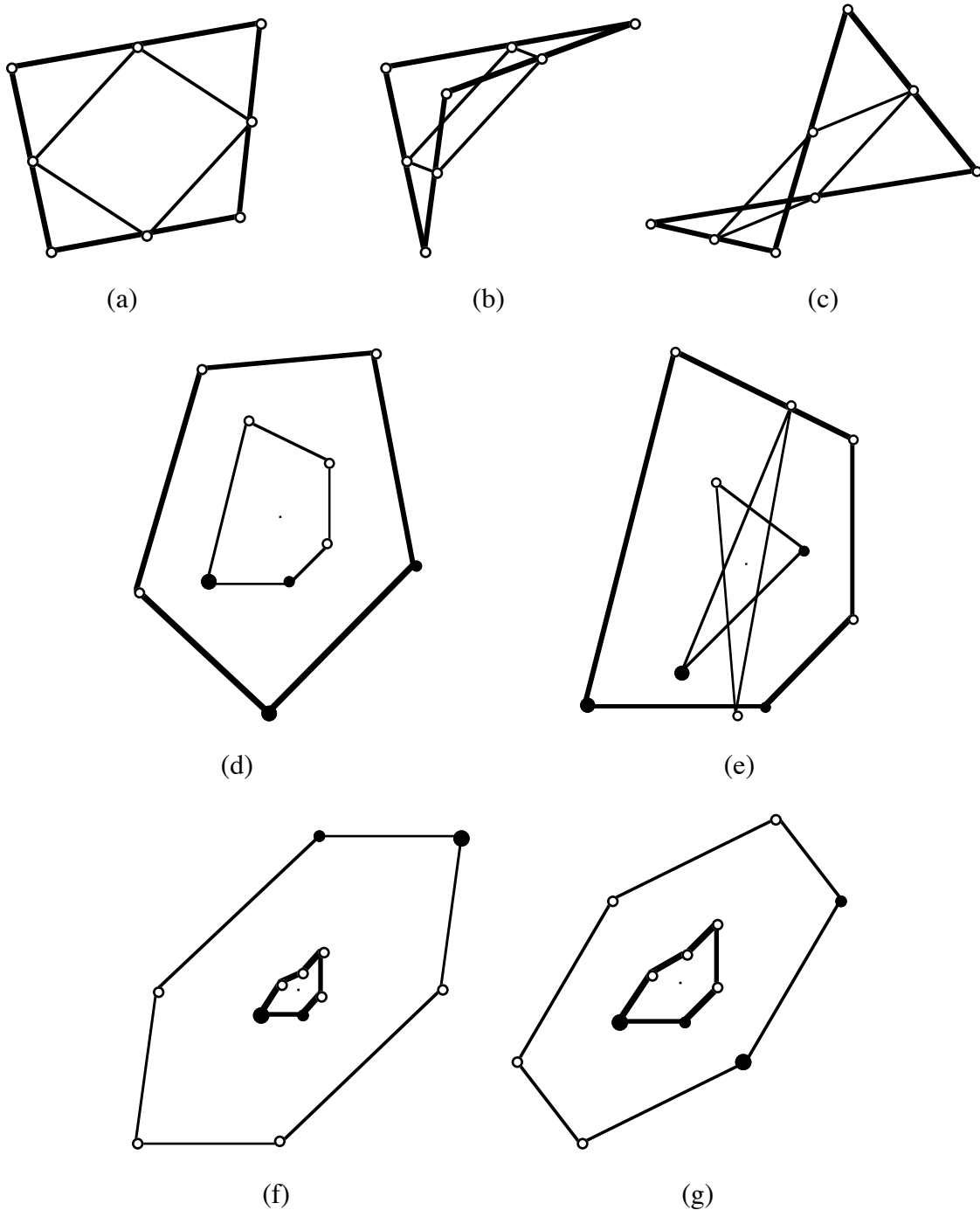
Figure N3.2. Examples of the action of some regularizing vectors. (a), (b), (c) show results of applying the (4/1) -regularizing vector b = (1/2, 1/2, 0, 0) . (d) illustrates the (5/1) -regularizing vector b = (1, 1.61803\dots, 1, 0, 0) , and (e) the (5/2) -regularizing vector b = (1, -0.618934\dots, 1, 0, 0) . (f) and (g) show the action of the (6/1) -regularizing vectors b = (-1, 0, 2, 3, 2, 0) and b = (1, 2, 2, 1, 0, 0) . The starting polygons are shown in heavy lines.
