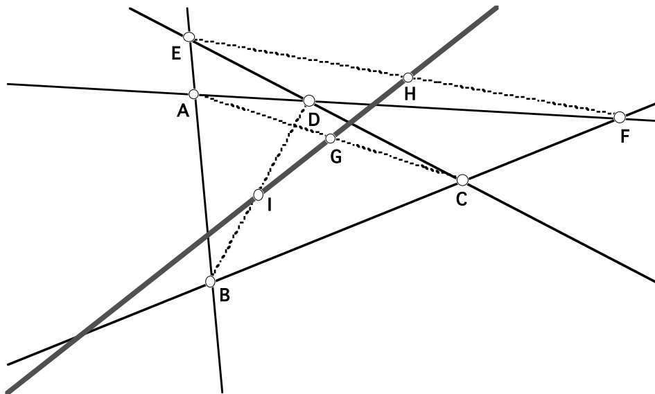
Figure 1.3. The Newton-Gauss line of a quadrilateral. Starting with four lines in general position, three "diagonals" are determined; their midpoints are collinear, on the Newton-Gauss line.
