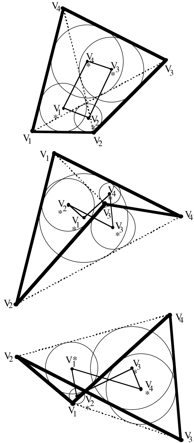
Figure N8.1. Examples of the incircle construction. In each, the quadrangle P is shown with heavy lines, its diagonals with dotted lines, and the derived quadrangle with thin lines. The four circles inscribed into the triangles T_j are also shown.
