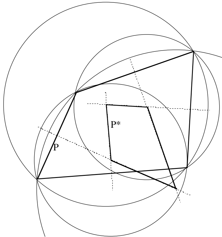
Figure N8.7. An illustration of the circumcenter map leading from a polygon P to the polygon P^* = C(P) .
