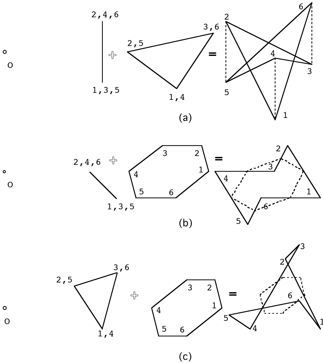
Figure N4.5. Examples of hexagons for which one affine-regular component is missing. The missing component is (6/1) in (a), (6/2) in (b), and (6/3) in (c).
