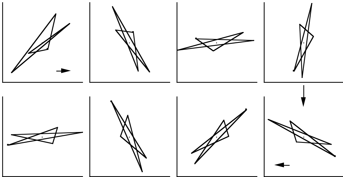
Figure N6.7. The same polygon as in two preceding figures is transformed by the smoothing operation with eigenvalues vector \lambda = (1, 0, (3+4i)/5, i, 0) . Here not both rotations (through \phi_2 = 53.13010235^\circ and \phi_3 = 90^\circ ) are commensurable with 360^\circ , and neither is their difference; therefore there is no periodicity, and even no repetition of the shape. All polygons are different.
