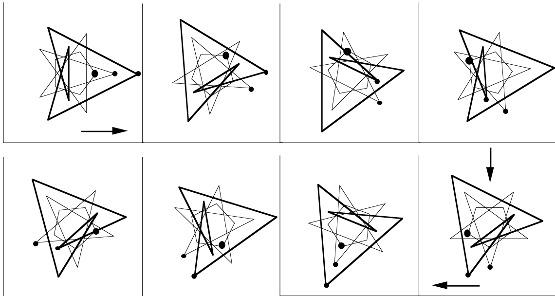
Figure 6.12. Iteration of the same map S(b) as in Figure 6.11 applied to a pentagon P which is the vertex sum of a regular (5/1) -gon and a regular (5/2) -gon. The rooted iterated polygons in are rotationally equivalent after five steps, and the unrooted polygons are all rotationally equivalent.
