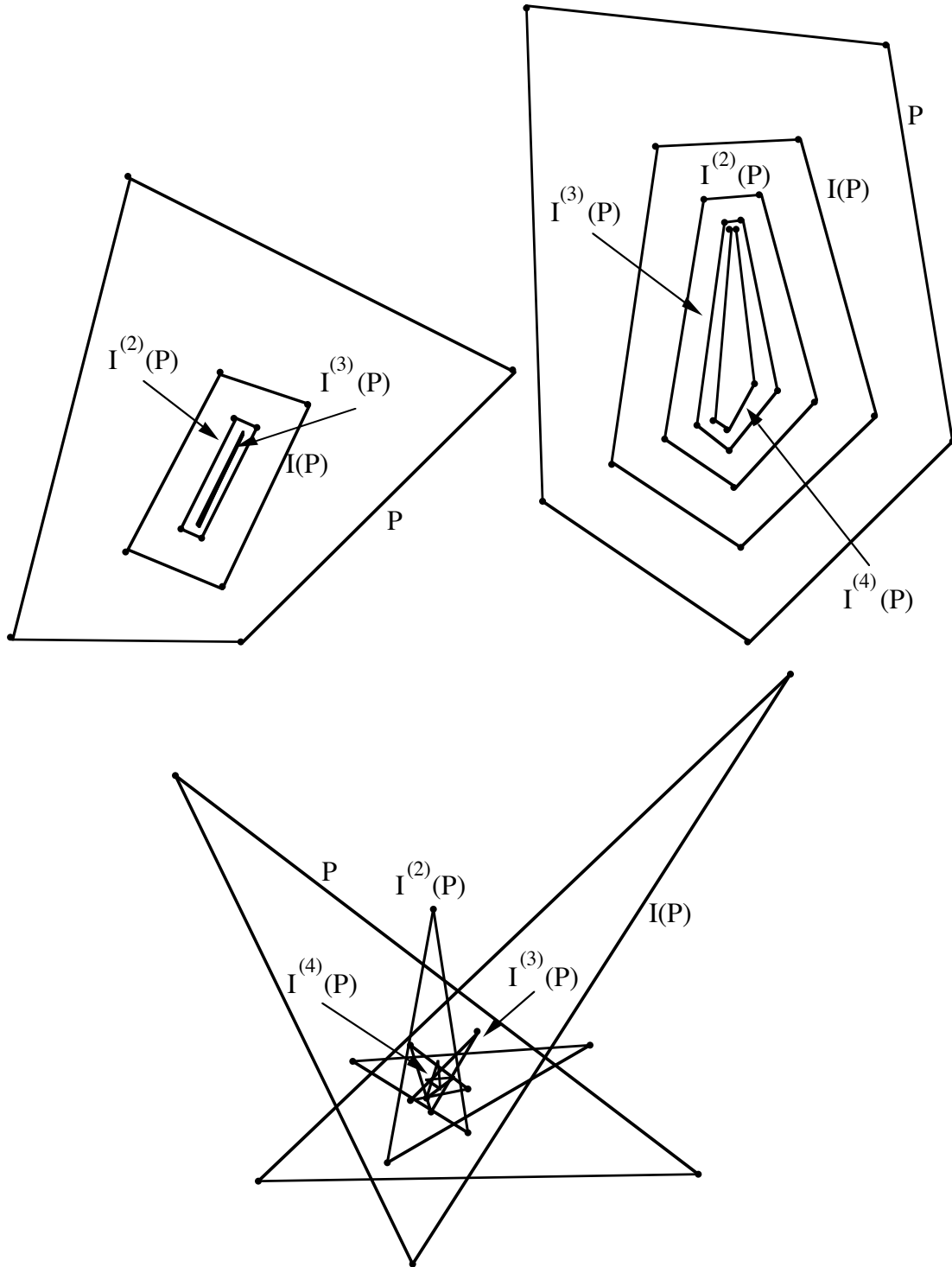
Figure N8.2. Iterations of the incircle map seem to lead to limits which are either segments or points.
