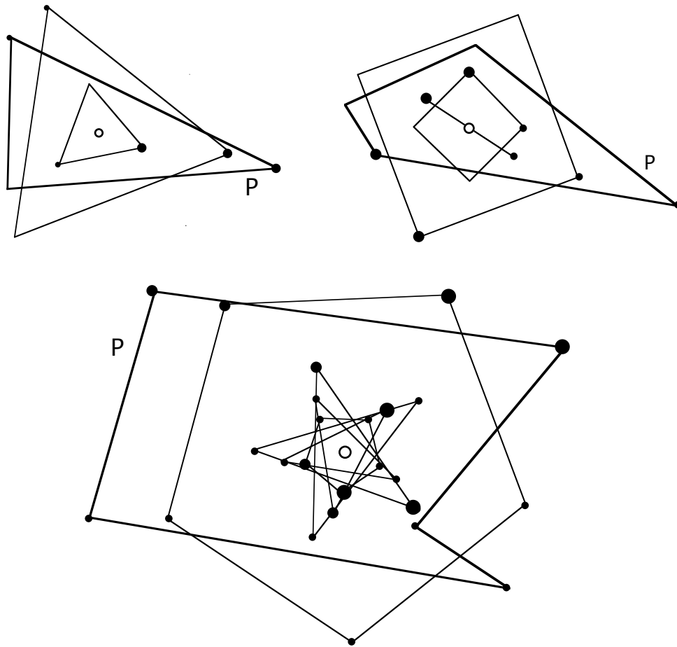
Figure N1.7. The regular components of an n -gon P . The dots of various sizes indicate not only the orientation of the polygons, but also the vertices of the regular components which add up to the vertex of P represented by the same kind of dot. The hollow dot indicates the origin.
