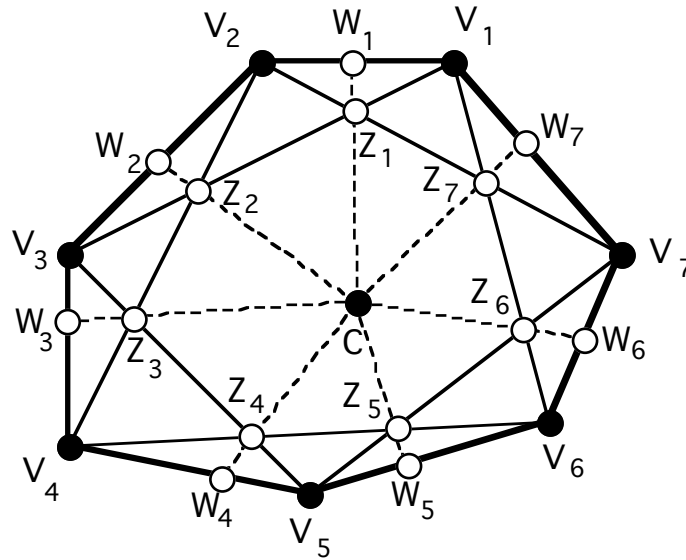
Figure 7.23. An illustration of the case (b) of the Ceva variant theorem, with n = 7 and k = 1 .
