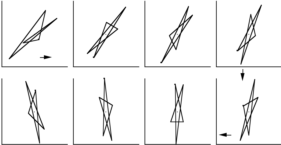
Figure N6.6. The same polygon as in Figure N6.5 is transformed by the smoothing operation with eigenvalues vector \lambda = (1, 0, 3+4i, 4-3i, 0)/5 . Since the rotations of the (5/2) - and (5/3) -components differ by 90^\circ , the shape of the pentagon is repeated after four iterations (beyond the first one), but this congruent pentagon is rotated through an angle that is incommensurable with 360^\circ . Hence the transformation is nonperiodic, although only four shapes appear.
