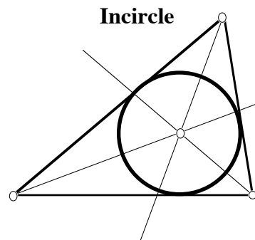
Figure 1.1. The four traditional "remarkable points" of a triangle, and the two circles and one line to which they lead.
