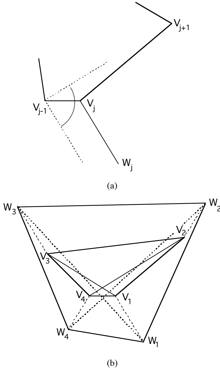
Figure N5.1. (a) A smoothing operation defined by a linear operation described in the text. (b) When applied to an arbitrary quadrangle, this linear operation produces a quadrangle in which the diagonals are perpendicular and have the same length.
