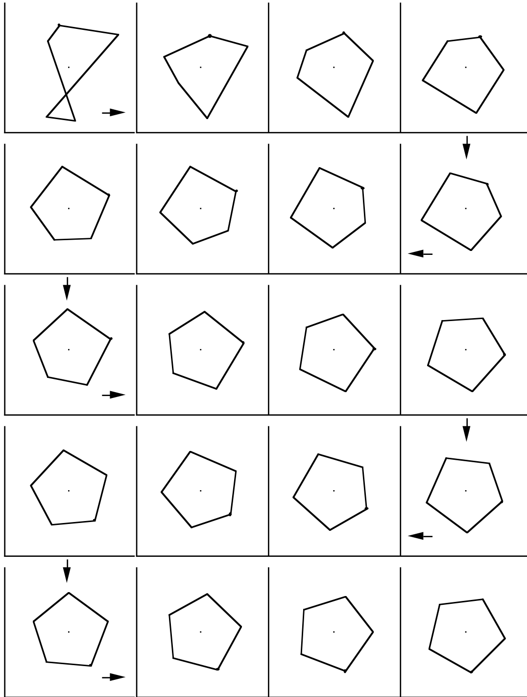
Figure N6.3. The iteration of the smoothing operation S(b) with b = (0.5062325629, -0.5062325629i, 0, 0, 0) , a rescale of (1, -i, 0, 0, 0) , applied to a pentagon in which all regular components are nontrivial. Here \lambda_1 = 0.9876883407 - 0.1564344651i , \rho_1 = 1 , \phi_1 = -9^\circ ; \lambda_2 = 0.8037885977 + 0.4095507465i , \rho_2 = 0.9021130327 , \phi_2 = 27^\circ ; \lambda_3 = 0.2086765282 + 0.4095507465i , \rho_3 = 0.4596495485 , \phi_3 = 63^\circ ; \lambda_4 = 0.0247767852 - 0.1564344651i , \rho_4 = 0.1583844403 , \phi_4 = -81^\circ . The iterates are co-convergent with a sequence of regular (5/1) -gons, which rotate -9^\circ with each iteration.
