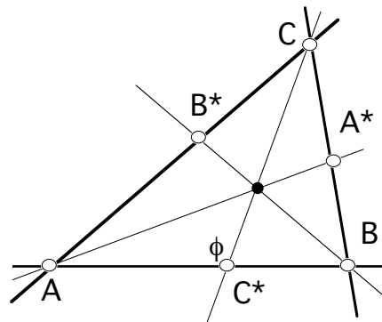
Figure 2.5. Notation for the proof of existence of the incenter, the point of concurrence of the three angle-bisectors.
