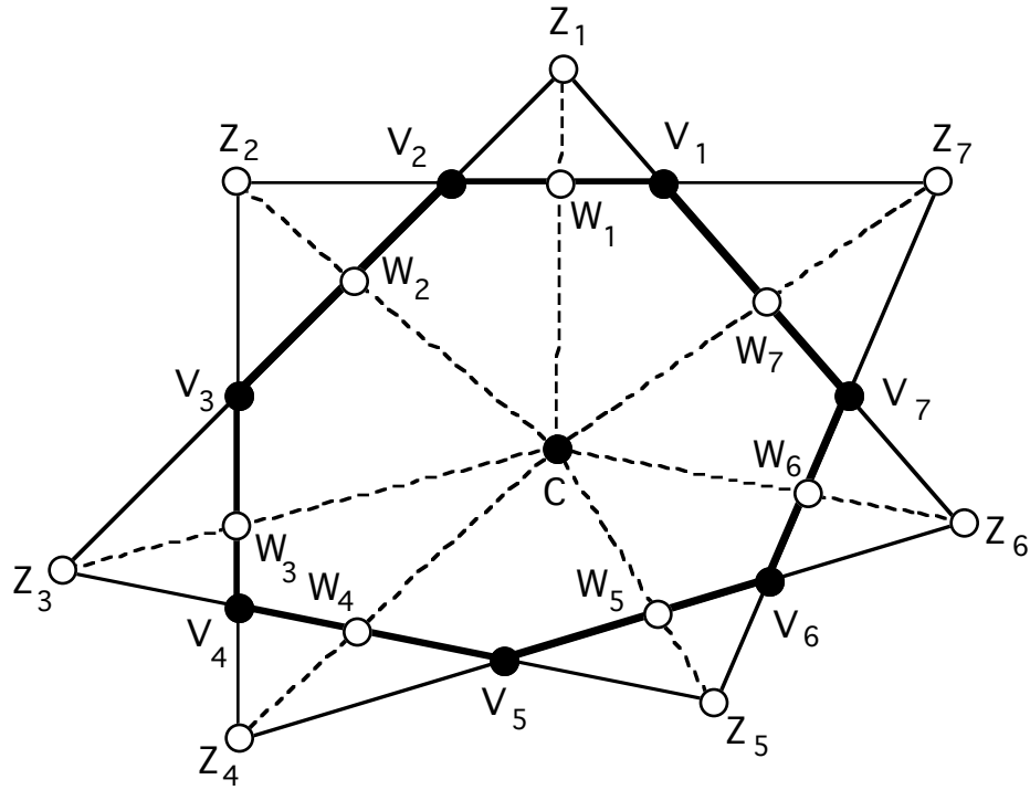
Figure 7.2. An illustration of the case (a) of the Ceva variant theorem, with n = 7 and k = 1 .
