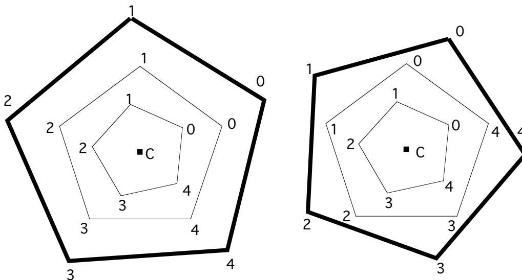
Figure N1.5. The sum of two rooted regular \{5/1\} -gons is itself a rooted regular \{5/1\} -gon. Note that the resulting polygon depends on the choice of roots.
