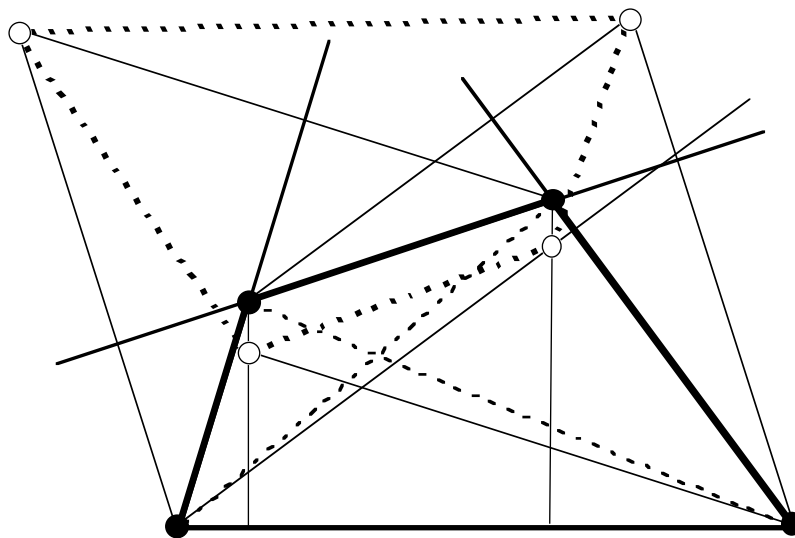
Figure N8.4. Construction of the polygon O(P) (heavy dotted line) from the quadrangle P (heavy lines). Only two altitudes (thin solid lines) are shown for each of the four triangles, each of which is determined by two adjacent sides of the quadrangle and one diagonal (dotted lines).
