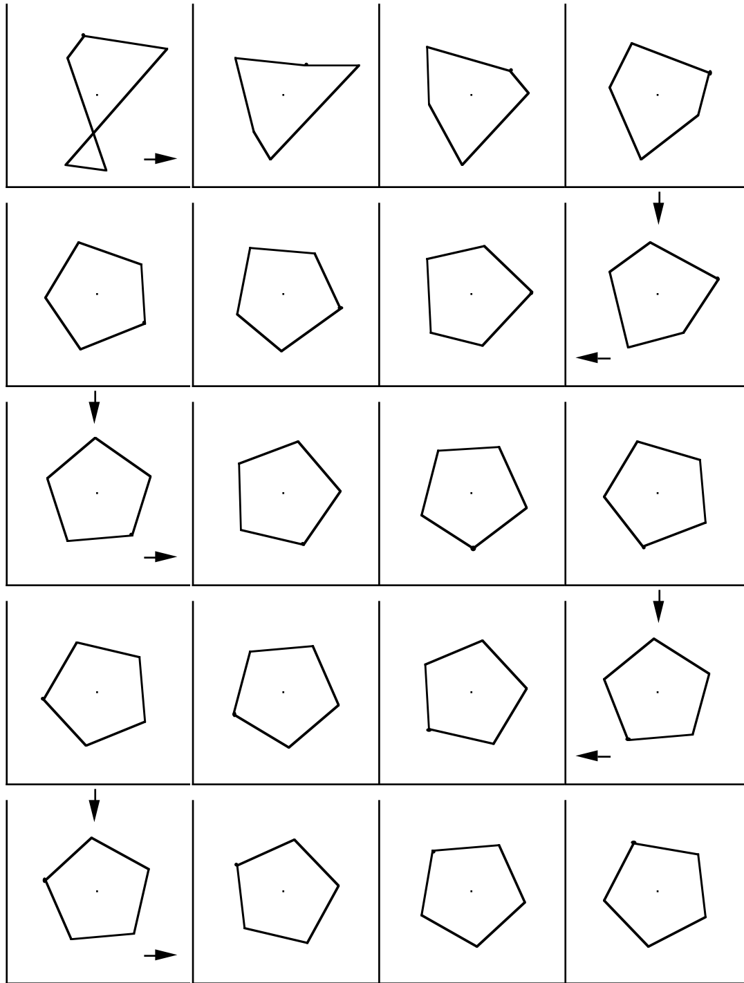
Figure N6.4. The iteration of the smoothing operation S(b) with b = (0.538901508, -0.269450754 i, 0, 0.269450754 i, 0) , a rescale of (1, -0.5 i, 0, 0.5 i, 0) , applied to a pentagon in which all regular components are nontrivial. Here \lambda_1 = 0.9535435829 - 0.3012551013 i , \rho_1 = 1 , \phi_1 = -17.53300301^\circ ; \lambda_2 = 0.441017792 + 0.3012551013 i , \rho_2 = 0.5340892518 , \phi_2 = 34.33661506^\circ ; \lambda_3 = 0.636785224 + 0.3012551013 i , \rho_3 = 0.704450181 , \phi_3 = 25.31824382^\circ ; \lambda_4 = 0.1242594332 - 0.3012551013 i , \rho_4 = 0.3258758088 , \phi_4 = -67.58520093^\circ . The iterates are co-convergent with a sequence of regular (5/1) -gons, which rotate -17.53300301^\circ with each iteration.
