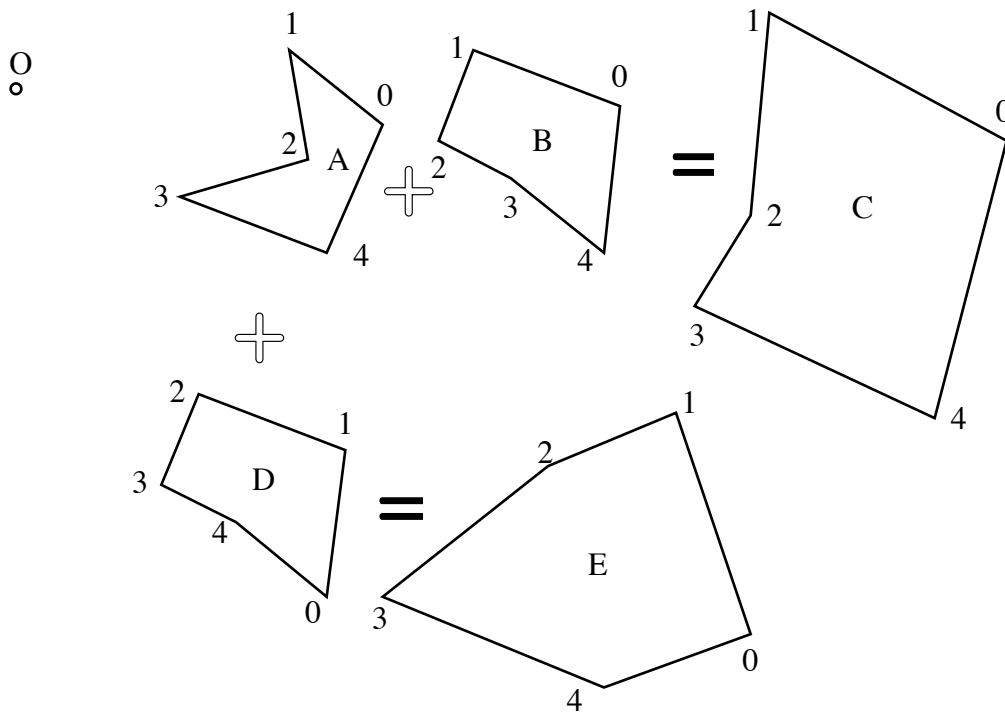
Figure N1.3. Different choices of roots lead to different vertex sums.
