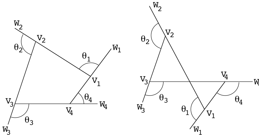
Figure N8.9. The definition of the deflections \theta_j at the vertices V_j of a quadrangle. Since the angles are to be measured in the counterclockwise direction, in the illustration at right the angles \theta_1 and \theta_4 are negative.
