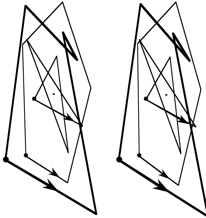
Figure N7.1. A stereoscopic pair of images, showing the decomposition of a nonplanar pentagon in \mathbf{E}^3 (shown by heavy lines) into two affine-regular pentagons. The arrowed edge of the pentagon is in the plane of the paper, the arrowed edge of the (5/1) -gon points out of this plane upwards, and the one of the pentagram points downwards.
