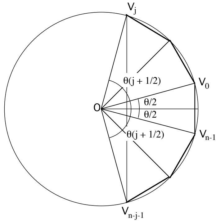
Figure N3.6. Illustration of the arguments in the proof of Corollary N3.8.
