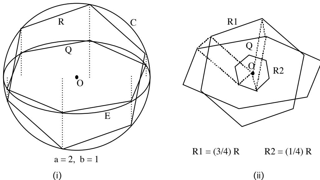
Figure N2.2. The construction, explained in the text, of two regular polygons whose vertex sum is the given affinely regular polygon.
