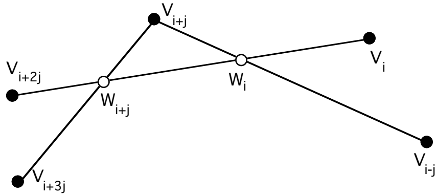
Figure 6.2. The notation used in the transformation of a typical ratio in the circular product appearing in Hoehn's First Theorem.
