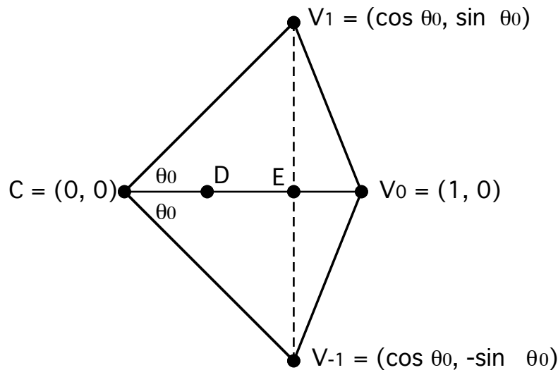
Figure N4.4 The calculation of the coefficients needed to show relation (3) can be accomplished easily using the point E = (\cos \theta_0, 0) ; here \theta_0 = 2\pi d_0/n is the central angle of the standard regular (n/d_0) -gon R_{n,d} . The center of the affine-regular (n/d) -gon is at D , and this is the vertex of P^{(d)} resulting from V_0 . The ratio CV_0/EV_0 = 1/(1 - \cos \theta_0) , and similarly DV_0/EV_0 = 1/(1 - \cos \theta) , with \theta = 2\pi d/n . Then the desired ratio CD/CV_0 has the same value as \lambda(n,d,d_0) from Theorem N4.2.
