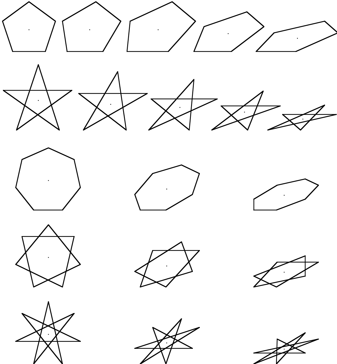
Figure N2.1. Examples of affinely regular pentagons and heptagons. In each row, the first polygon is regular. The first polygon in each row is regular and those following are affine images of it. They therefore belong to \mathcal{A}(5/1) , \mathcal{A}(5/2) , \mathcal{A}(7) , \mathcal{A}(7/2) and \mathcal{A}(7/3) , respectively.
