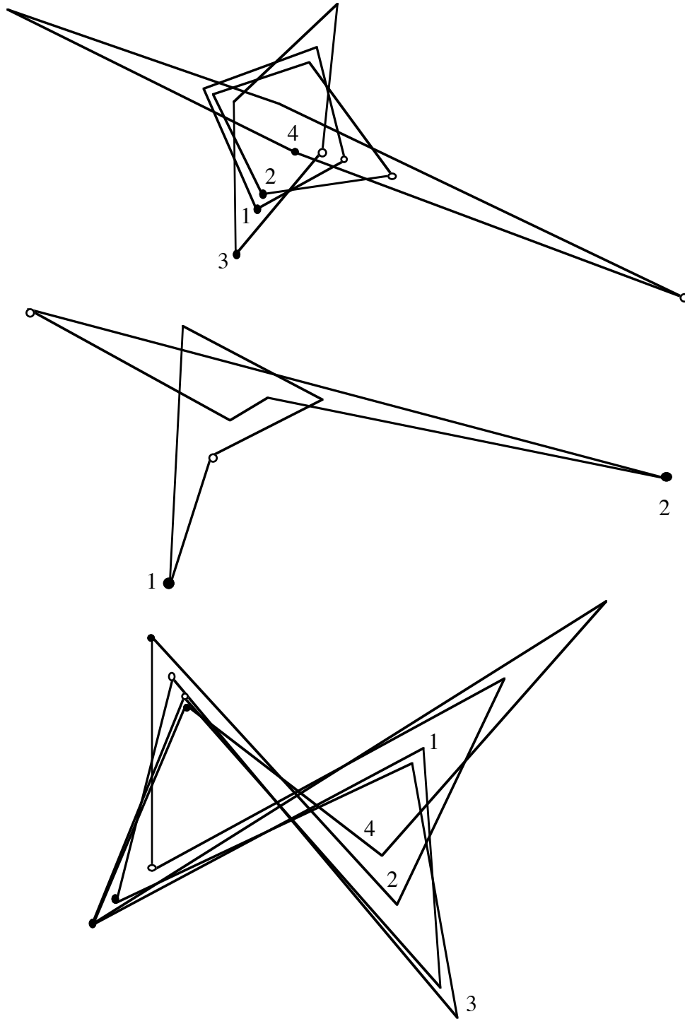
Figure N8.5. Three examples of iterations of the operation O . The starting quadrangle is labeled 1, and the other numerals indicate the iterates. Examples like these led to the idea of affine equivalence of the quadrangles P and O(P) .
