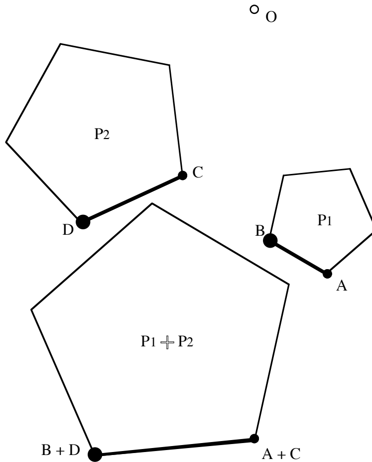
Figure N2.5. An illustration of Lemma N2.1.
