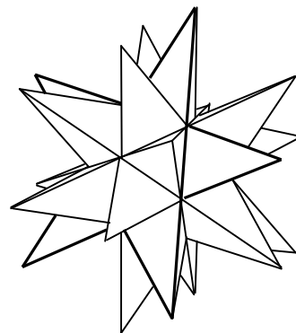
Great stellated dodecahedron \{5/2,3\}
