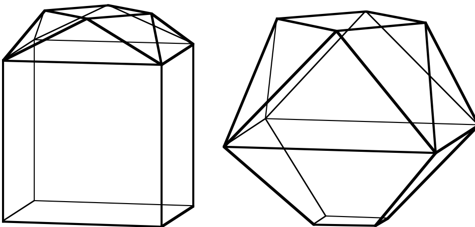
Figure 2. A convex polyhedron, and its canonical representative obtained by the Hart algorithm [34].
