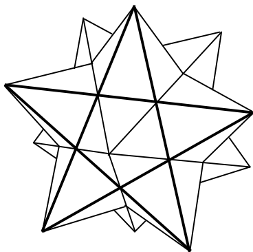
Small stellated dodecahedron \{5/2,5\}
