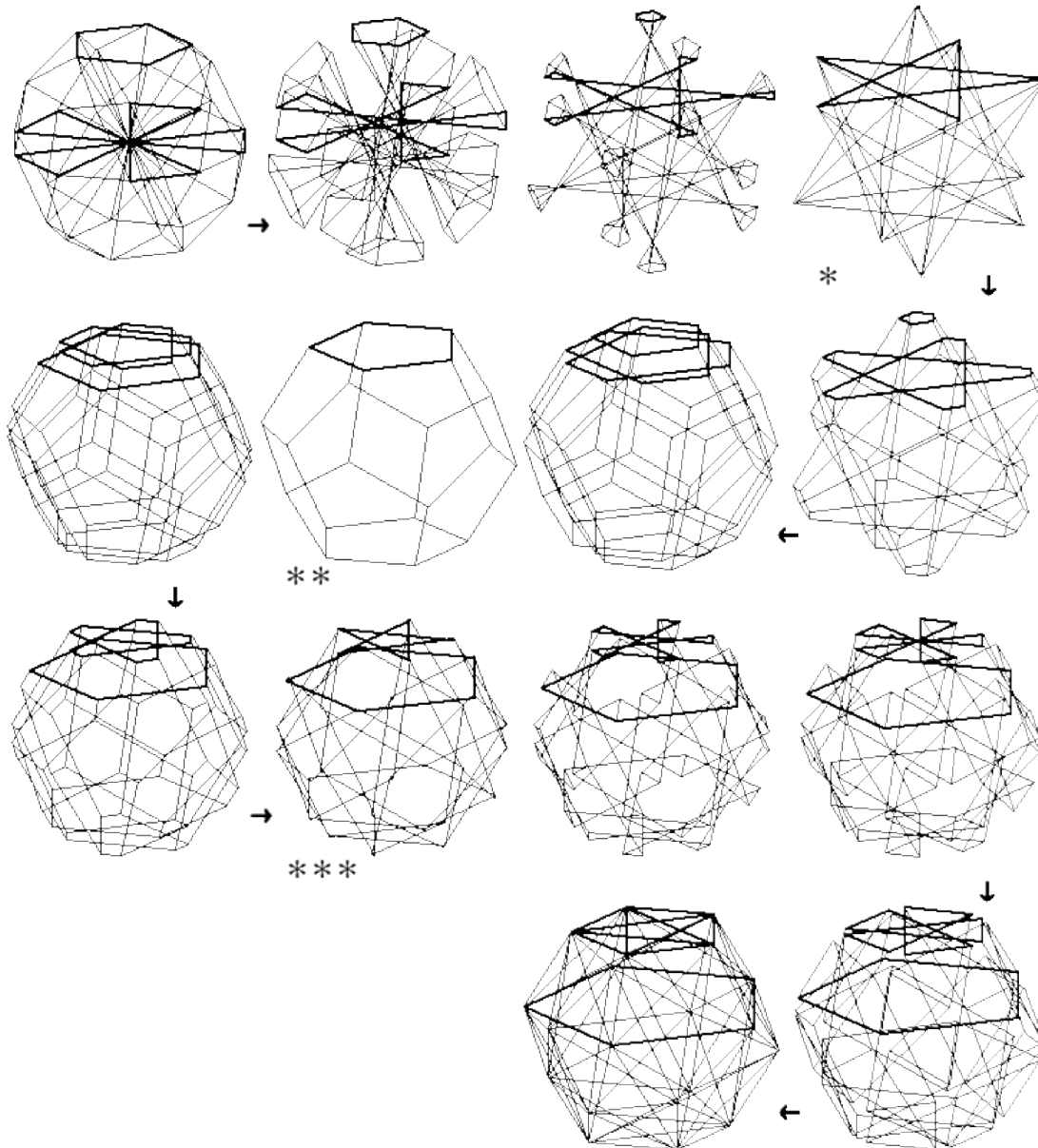
Figure 13. A representation of a part of the continuous family of realizations of an abstract isogonal icositetrahedron (5.10.10) , with 12 pentagonal and 12 decagonal faces. Each of the 60 vertices is incident with one pentagon and two decagons. The polyhedron is orientable, of genus 4. The realization marked by two asterisks is a "new" uniform polyhedron with symbol (5.10/2.10/2) . The realizations marked by asterisks are isomeghetic (represented by the same point set) as well known polyhedra: one asterisk and two asterisks indicate polyhedra isomeghetic with regular polyhedra (small stellated dodecahedron \{5/2, 5\} and dodecahedron \{5, 3\} , respectively). The polyhedron marked by three asterisks is isomeghetic with the uniform dodecadodecahedron (5.5/2.5.5/2) . The polyhedra between those with one and two asterisks are isomeghetic with truncations of the small stellated dodecahedron.
