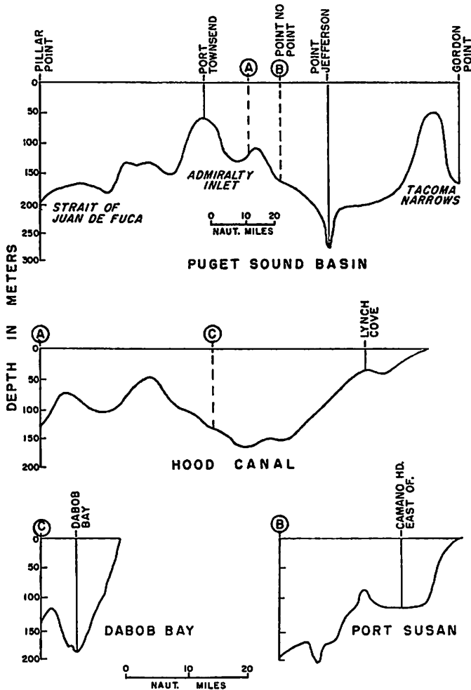
Figure 2. Schematic longitudinal section of the Puget Sound basin and selected appendages.
