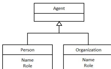
Figure 6: Agent Entities
