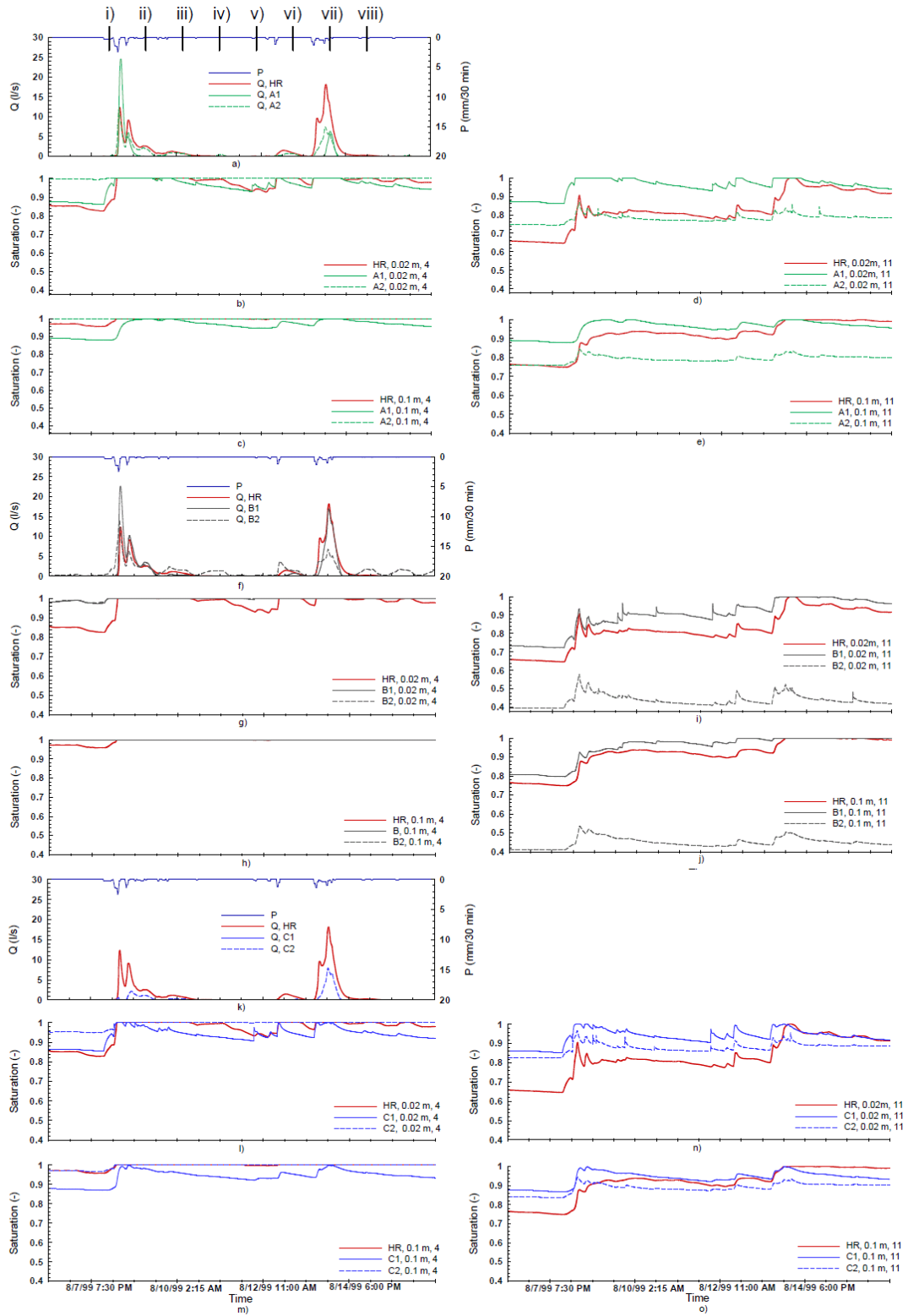
Figure 4.6 a), f), k) HR and A1, A2, B1, B2, C1, and C2 MODHMS hydrographs during the wet period A; b) - e), g) - j) and l) - o) HR and A1, A2, B1, B2, C1, and C2 MODHMS saturation at node 4 and node 11, depths 0.02 and 0.1 m.
