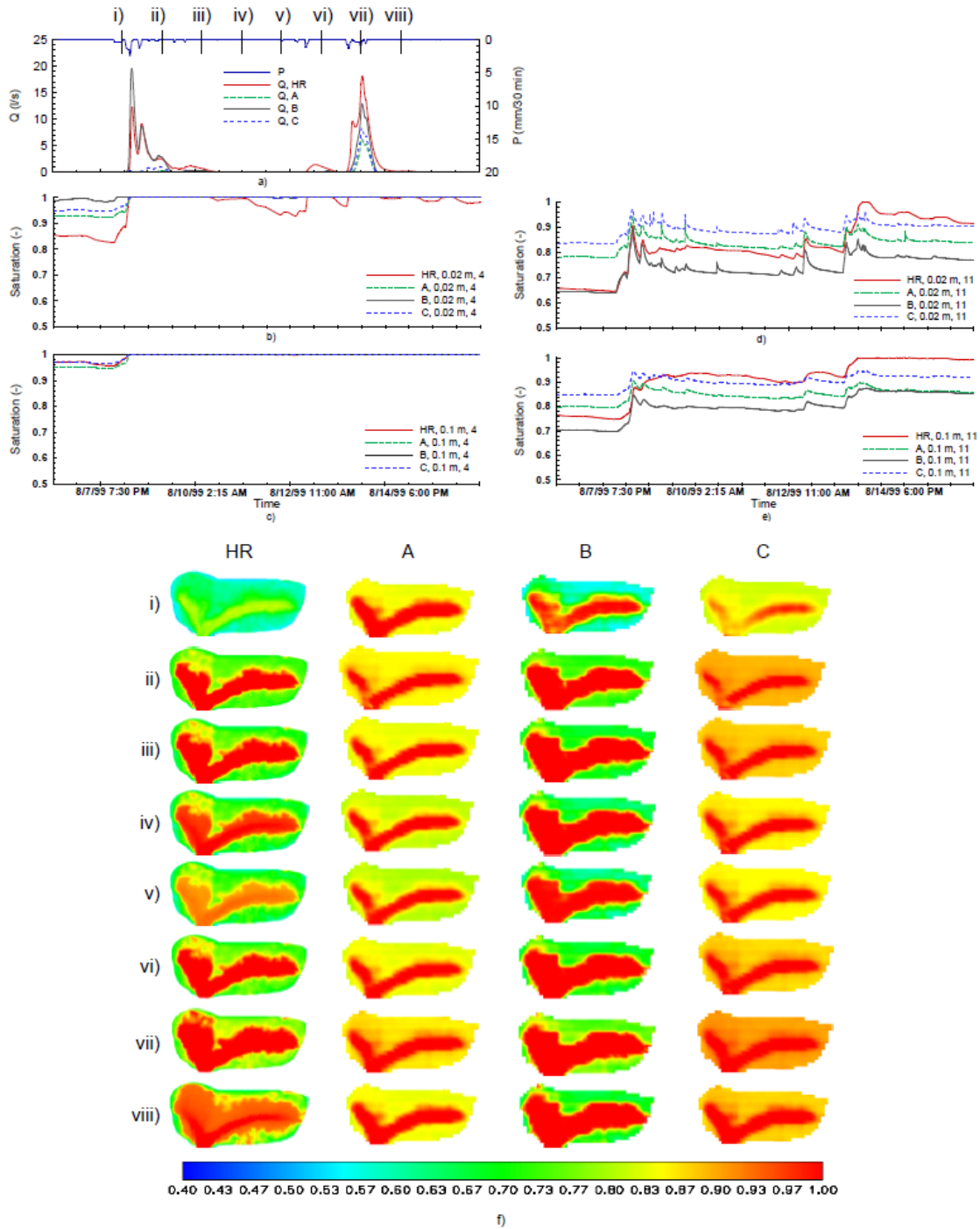
Figure 4.4 a) HR and A, B, and C MODHMS hydrographs during the wet period A; b) - e) HR and A, B, and C MODHMS saturation at node 4 and node 11, depths 0.02 and 0.1 m; f) spatial distribution of HR and A, B, and C MODHMS saturation in the top 2 cm at 24 h intervals, 8 August 1999, 0:00 AM to 15 August 1999, 0:00 AM.
