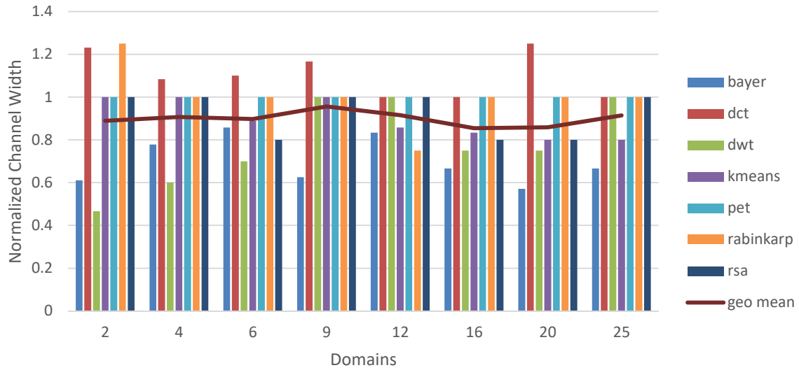
Figure 8.18. Channel width for EveryTime router compared to SPR.
