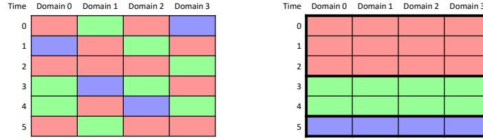
Figure 3.3. Example modulo schedule after flattening and IMS scheduling (left) and modulo schedule organized by mode (right).
