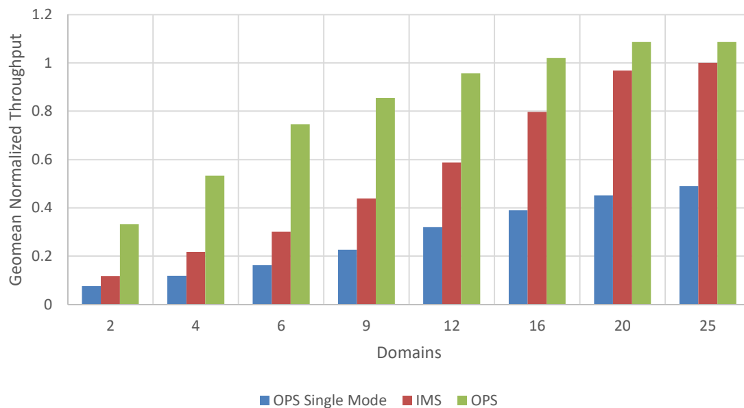
Figure 10.5. OPS to single mode applications.
