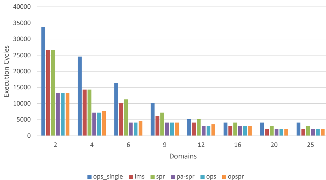
Figure 10.10. Cycles to execute DCT benchmark.
