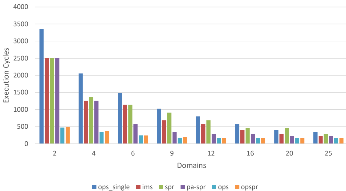
Figure 10.9. Cycles to execute Bayer benchmark.
