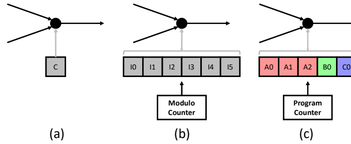
Figure 8.7. Configuration styles for (a) FPGAs, (b) modulo counter CGRAs, and (c) Offset Pipelined CGRAs.
