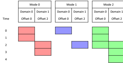
Figure 5.1. Example Offset Reservation Table.
