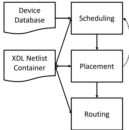
Figure 4.1. Tool chain overview.
