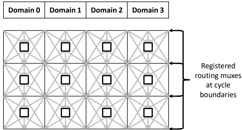
Figure 8.1. Simplified routing architecture
