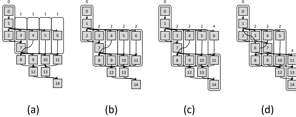
Figure 3.9. (a) Initial schedule, (b) front end shaping, (c) back end shaping, (d) rescheduling.
