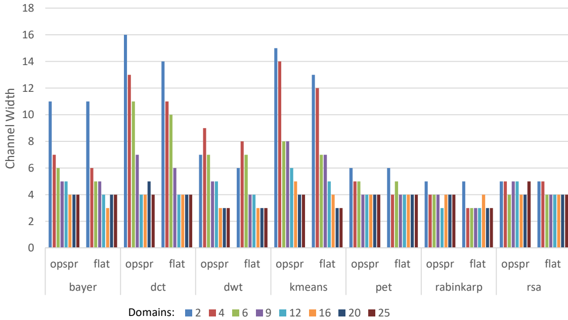
Figure 8.17. Absolute channel widths for EveryTime router compared to flattened baseline.
