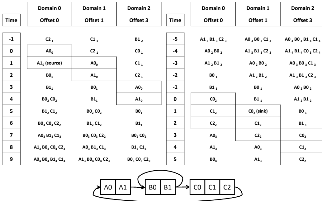
Figure 8.14. Unlocked net routed with a register file.
