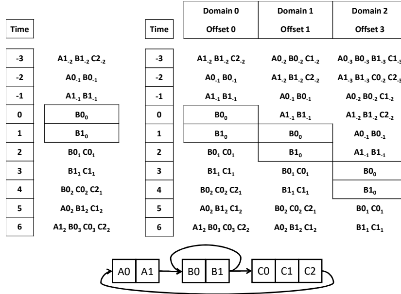
Figure 8.9. EveryTime table for mode B (left). EveryTime tables set to different offsets (right). Mode transition diagram for the EveryTime tables (bottom).
