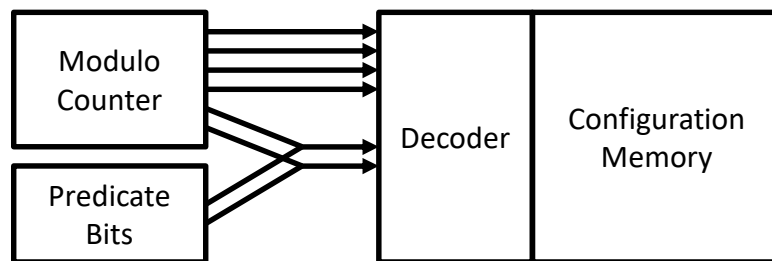
Figure 9.4. Predicate bits combined with modulo counter controlled configuration memory.
