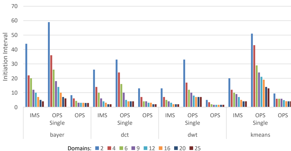
Figure 10.6. Scheduling II data for Bayer, DCT, DWT, and K-means benchmarks.
