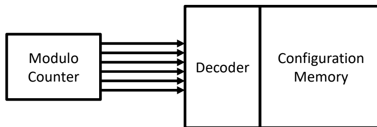
Figure 9.3. Modulo counter controlled configuration memory.
