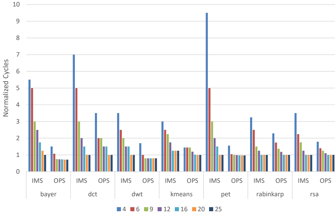
Figure 5.11. OPS vs IMS execution cycles normalized to recurrence limited II across various device sizes.
