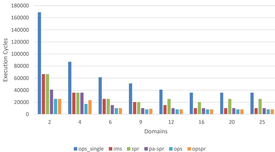
Figure 10.11. Cycles to execute DWT benchmark.
