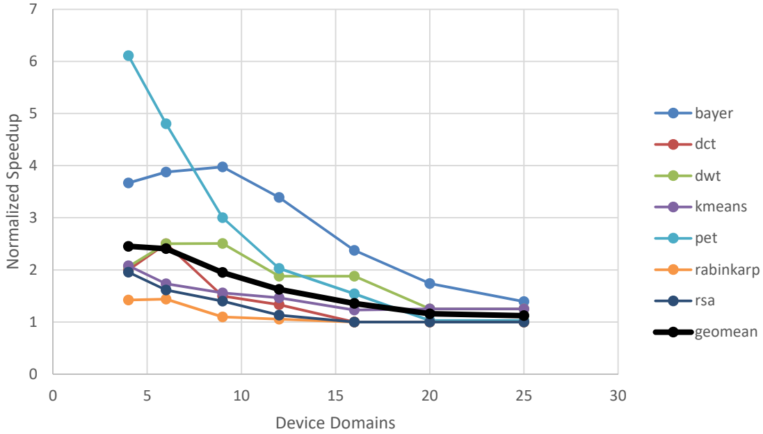
Figure 5.14. OPS vs IMS performance summary.
