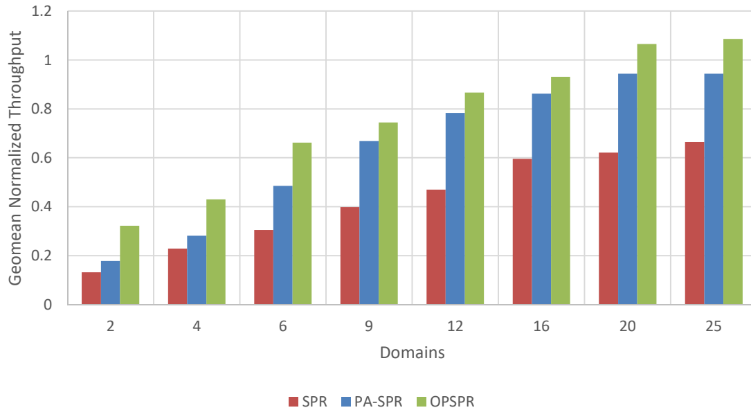
Figure 10.8. Offset Pipelining vs SPR and PA-SPR bound with performance normalized per benchmark to throughput of recurrence limited monolithic version.
