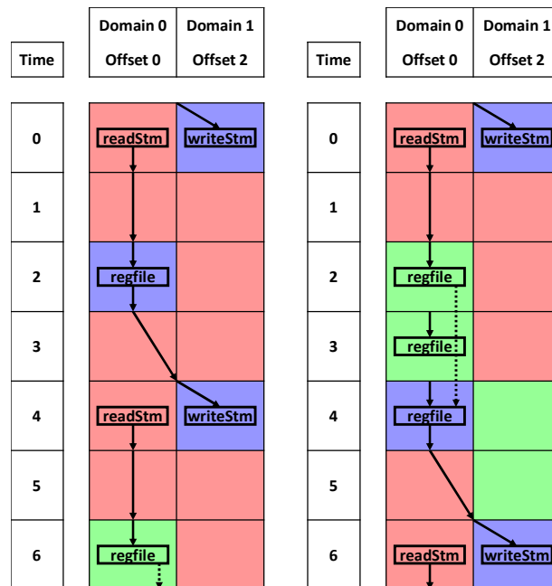
Figure 8.15. Example demonstrating the valid bit write enable for register files.
