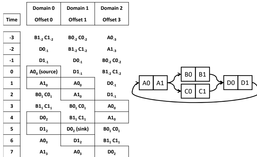
Figure 8.13. EveryTime table for fixed flight time multi-path net.
