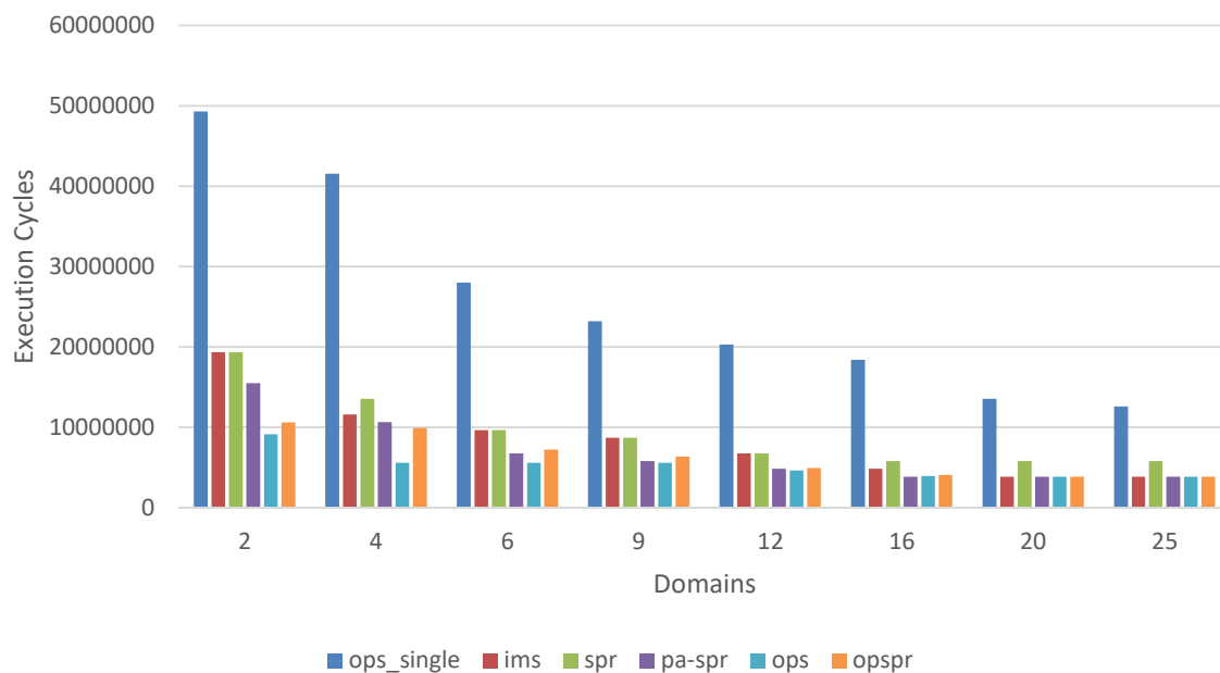
Figure 10.12. Cycles to execute K-means benchmark.
