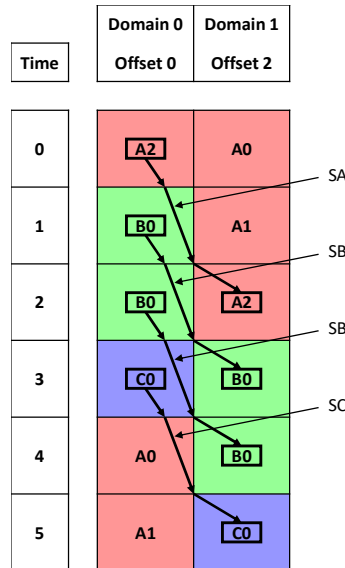
Figure 8.8. Resource costs for routing.
