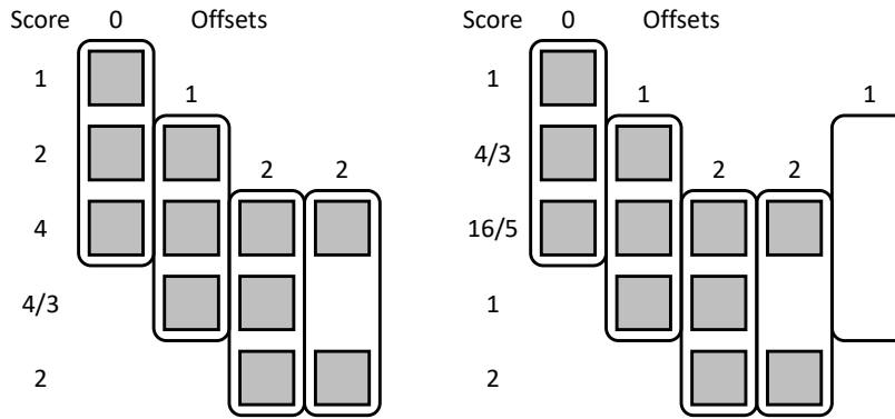
Figure 5.9. Spare domain offset assignment.
