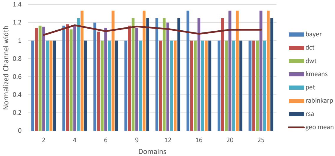
Figure 8.16. Channel widths for EveryTime router normalized to flattened architecture.
