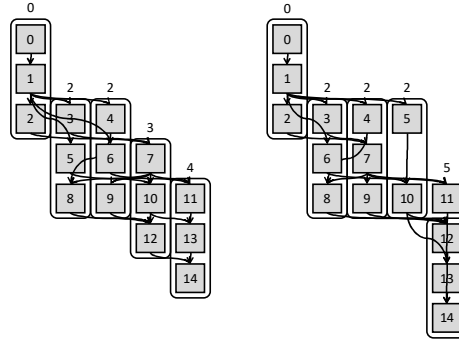
Figure 3.10. Offset Exploration with 0, 2, 2, 3, 4 and 0, 2, 2, 2, 5.
