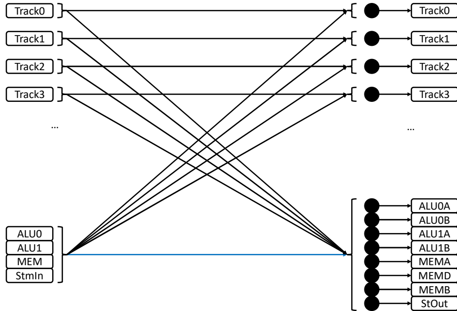
Figure 4.2. Domain interconnect organization.
