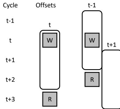
Figure 5.10. Memory operation scheduling cases.
