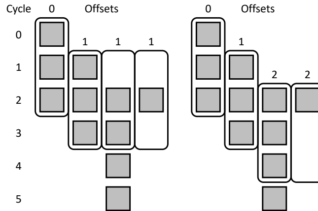
Figure 5.5. Before and after front-end shaping of a single mode with II = 3 .
