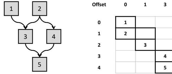
Figure 5.3. As-soon-as-possible operation scheduling.
