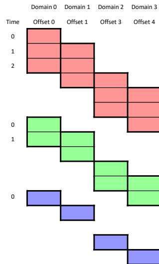
Figure 3.5. Independent mode schedules with shared staggering between resources.
