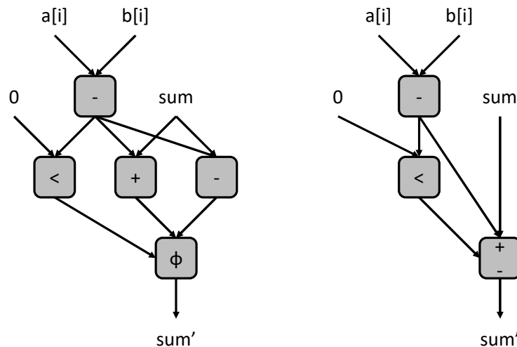
Figure 9.2. Predication (left) and predicate aware sharing (right) of Figure 9.1.
