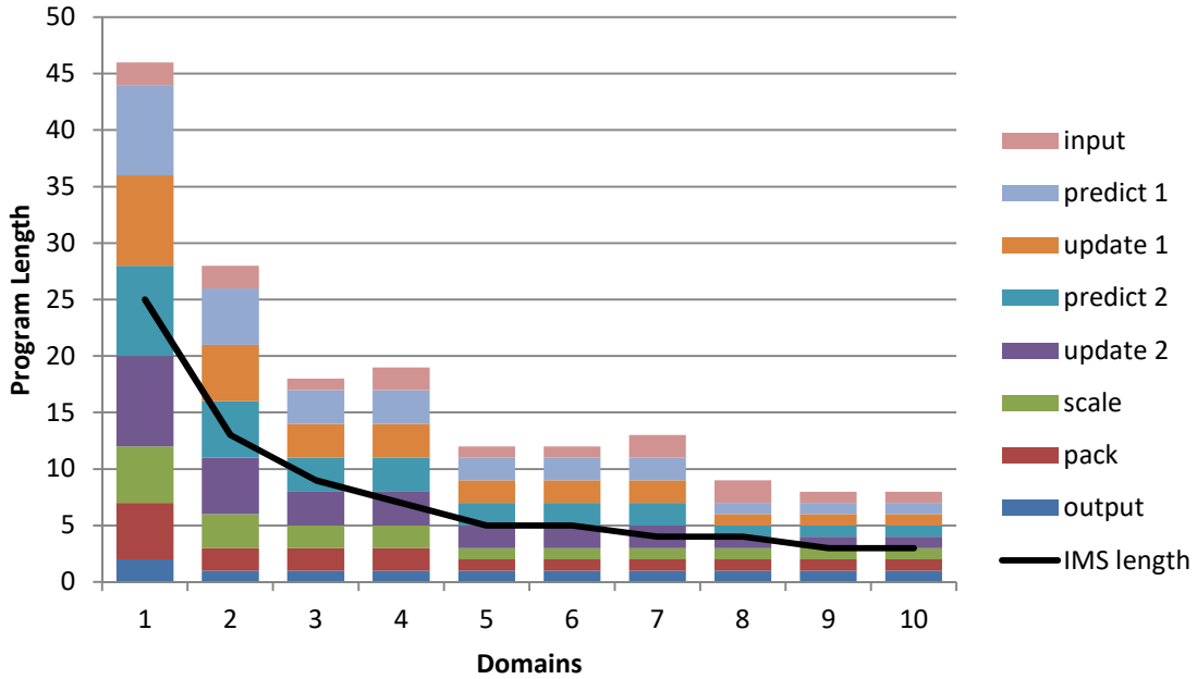
Figure 5.13. DWT mode IIs. Stacked bars are OPS mode IIs. The line is the IMS II.
