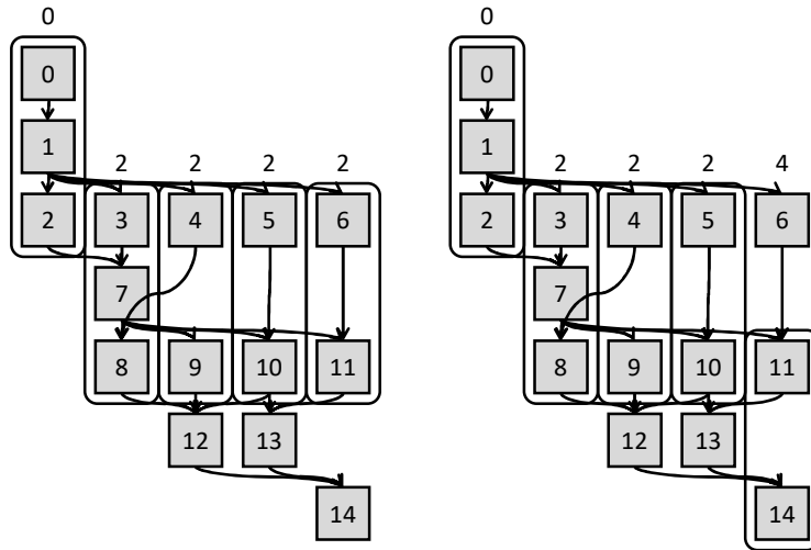
Figure 5.6. Before and after back end shaping. The initial schedule is infeasible. Subsequent scheduling passes will move operation 6 to a later cycle.
