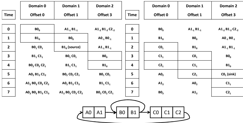
Figure 8.11. Source and sink relative routing tables for a net from mode B to mode C.
