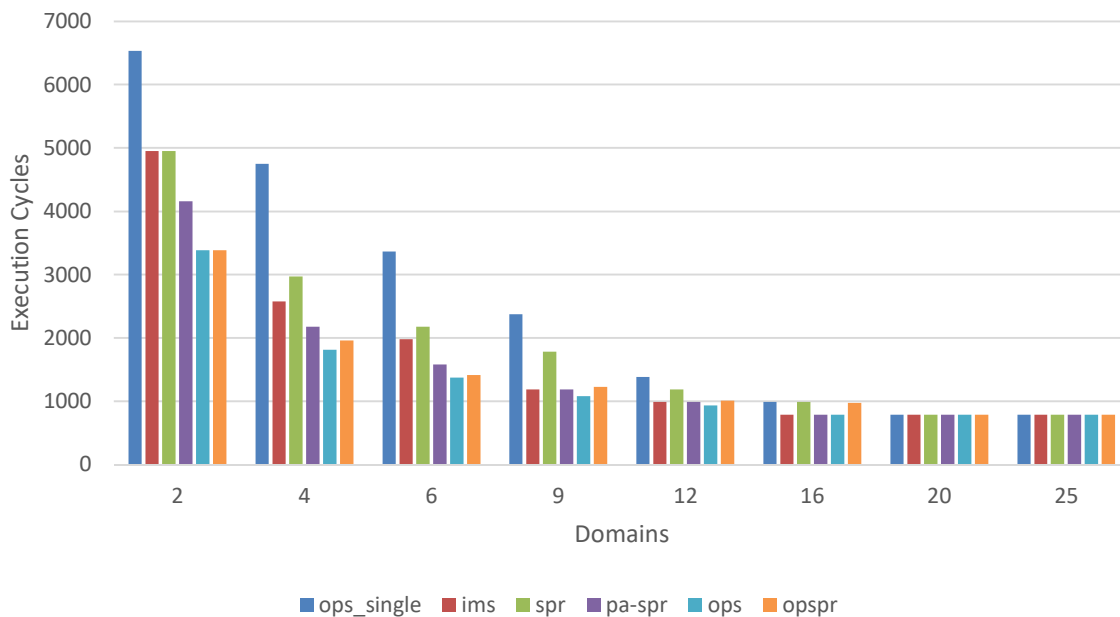
Figure 10.14. Cycles to execute RabinKarp benchmark.
