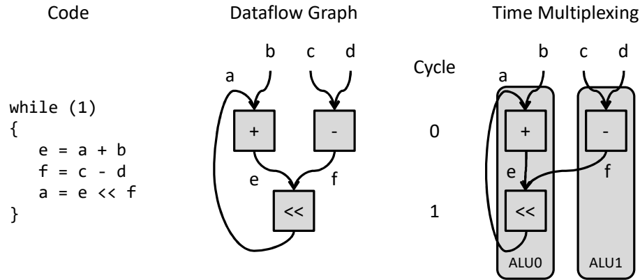
Figure 2.1. Source code (left) is converted to a dataflow graph (center) and mapped to a time multiplexed architecture (right).
