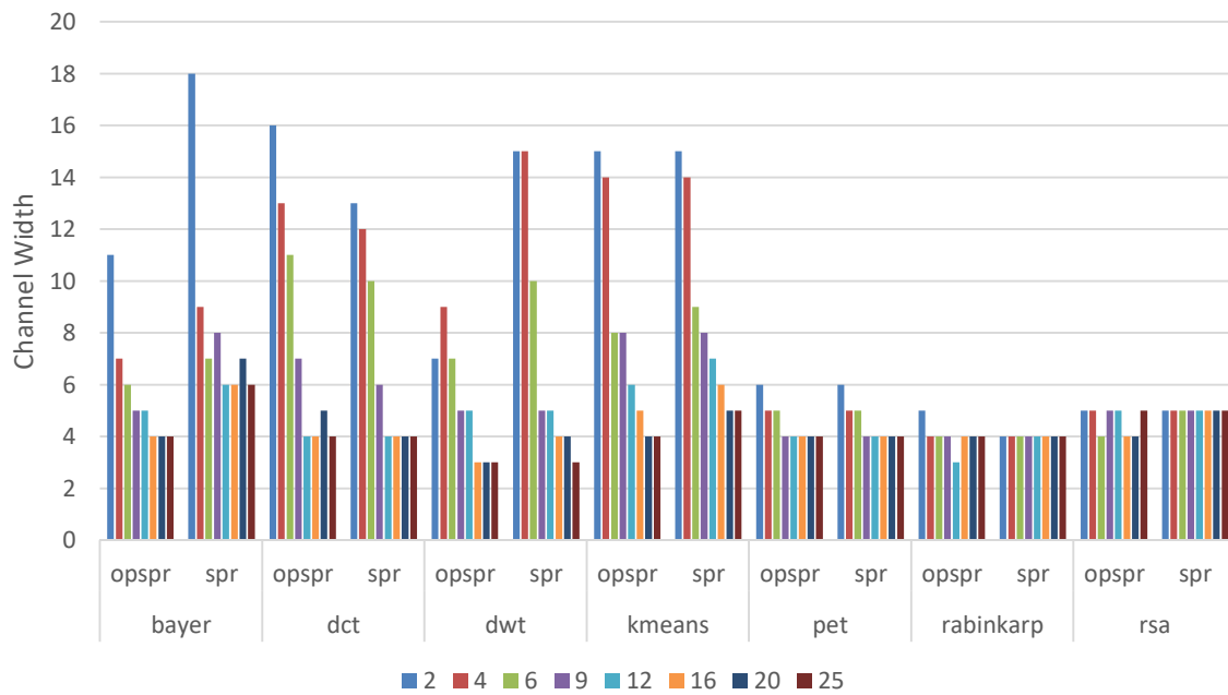
Figure 8.19. Absolute channel widths for EveryTime router compared to baseline SPR.
