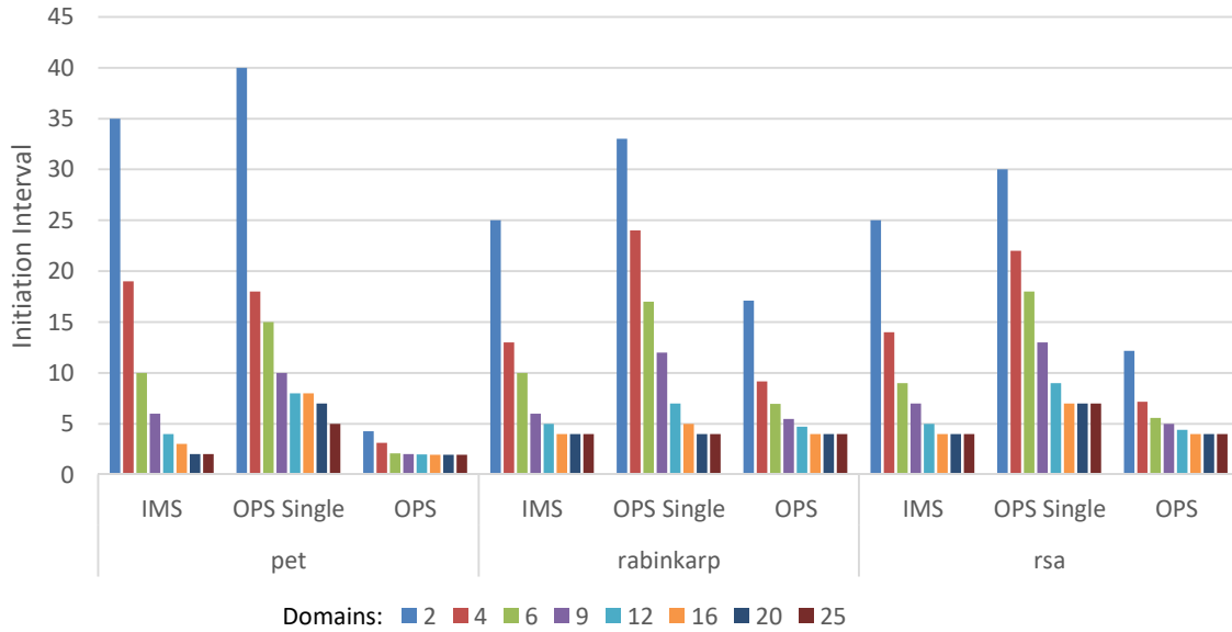
Figure 10.7. Scheduling II data for PET, RabinKarp, and RSA benchmarks.
