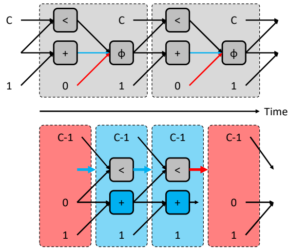
Figure 3.8. Phi nodes in modulo schedule (top), eliminated with Offset Pipelining (bottom).
