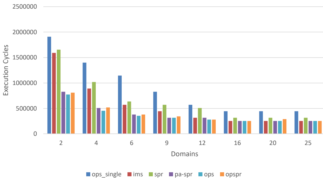
Figure 10.15. Cycles to execute RSA benchmark.
