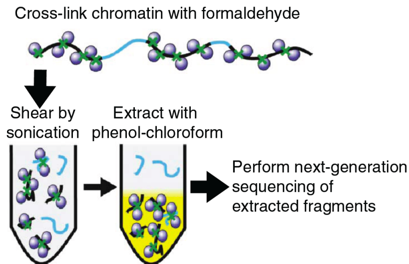
Figure 6.3. FAIRE-seq procedure.
