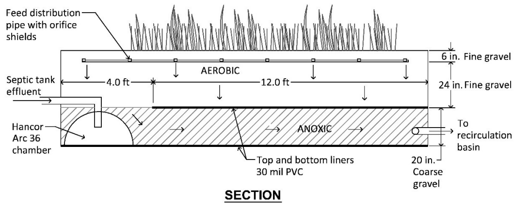
Figure 2. Schematic of the vegetated recirculating gravel filter system.
