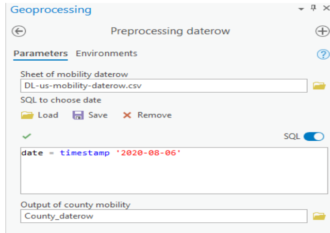
Figure A-4 Configuration of the custom tool
