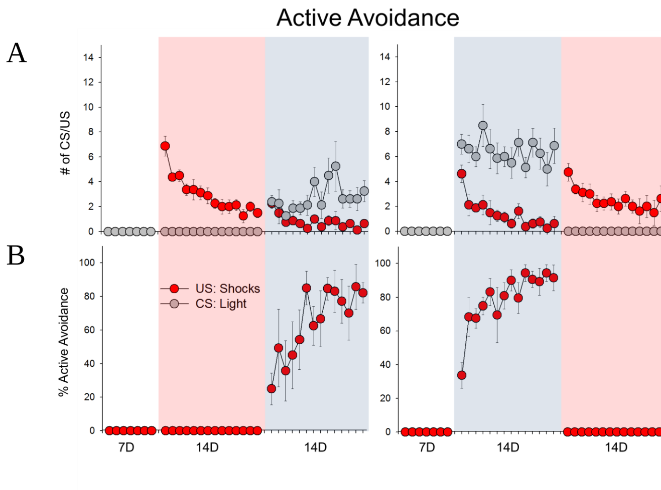
Figure 4.8. Number of US-shock (red) and CS-light (grey) presentations through signaled (blue) and unsignaled (pink) shock. (A) Number of light and shock presentations. (B) Percent of successful active avoidances through shock.
