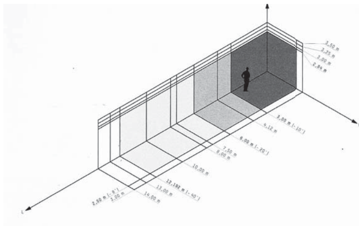
Fig: 4.5 Building Container Dimensions
