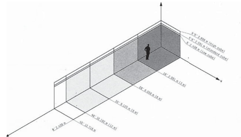
Fig: 4.3 Freight Container Dimensions
