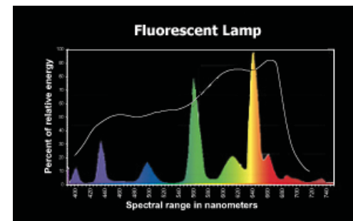
Fig: 3.2 Spectral Curve of Various Light Sources
