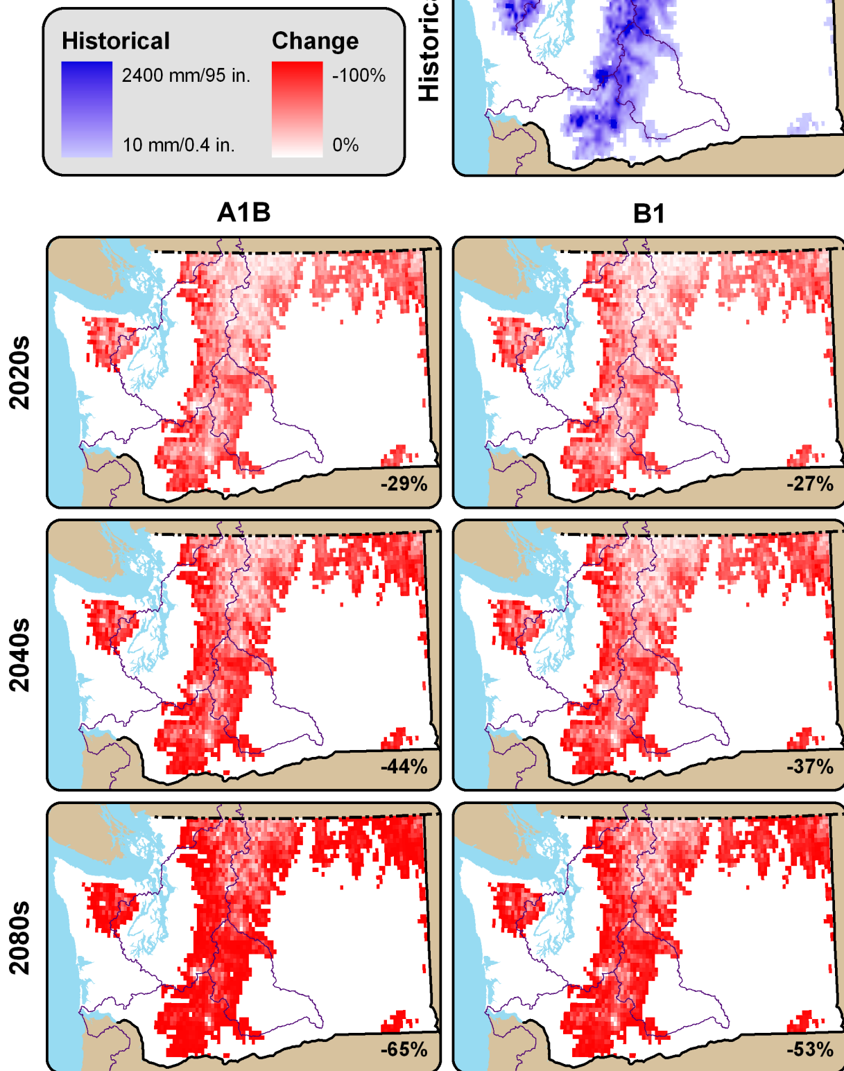
Figure 5. Summary of projected April 1 snow water equivalent (SWE) for the 2020s, 2040s and 2080s (A1B and B1 SRES scenarios) by the VIC model. Percent change values represent spatially averaged April 1 SWE across Washington State.
