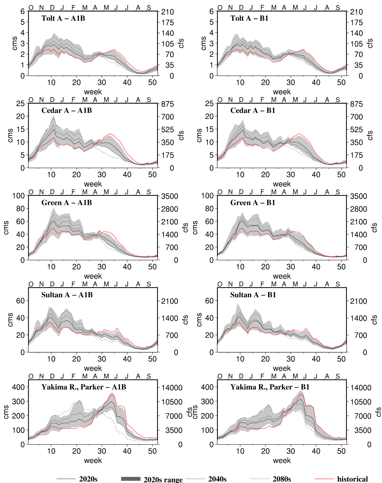
Figure 13. Projected changes in weekly streamflow for the 2020s, 2040s, and 2080s (A1B and B1 SRES scenarios). Results in the top four pairs of panels are based on DHSVM simulations, while the bottom pair of panels are based on VIC model simulations. Units are cubic meters per second (cms).
