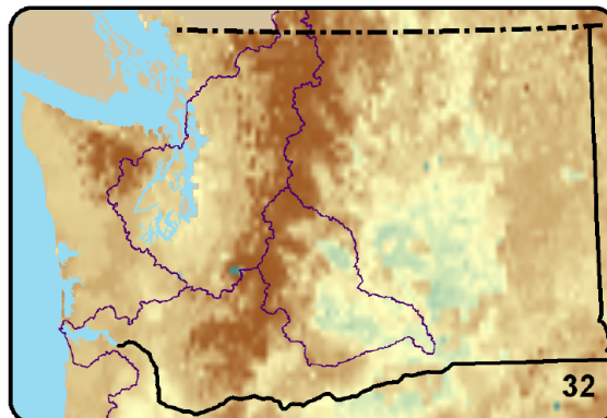
Figure 7. Summary of projected July 1 soil moisture for the 2020s, 2040s, 2080s (A1B and B1 SRES scenarios) as percentile of simulated historical mean from 1916-2006 (using the VIC model). Percentiles less than 50 represent a decrease in soil moisture, while percentiles greater than 50 show an increase in soil moisture. Reported values represent spatially averaged percentile across Washington State.
