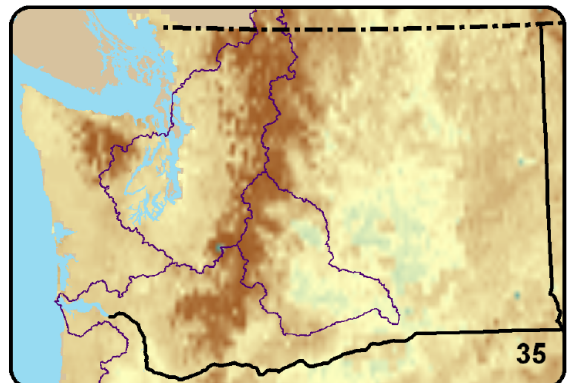
Figure 7. Summary of projected July 1 soil moisture for the 2020s, 2040s, 2080s (A1B and B1 SRES scenarios) as percentile of simulated historical mean from 1916-2006 (using the VIC model). Percentiles less than 50 represent a decrease in soil moisture, while percentiles greater than 50 show an increase in soil moisture. Reported values represent spatially averaged percentile across Washington State.
