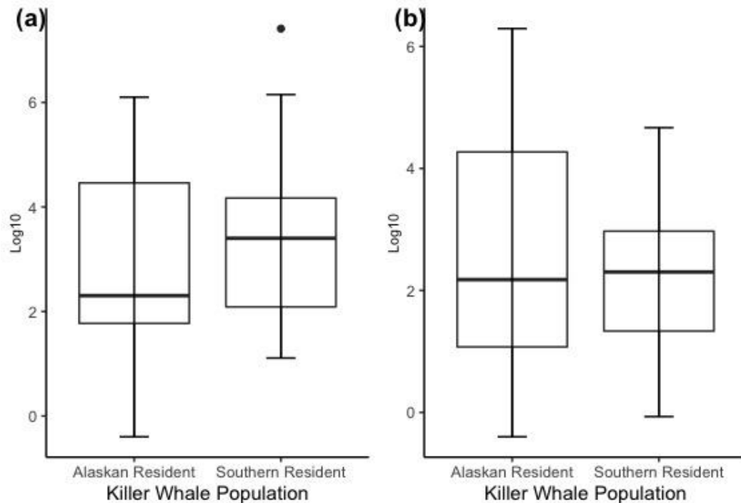
Figure 6. Total number of microparticles per gram of dry fecal matter compared across the two killer whale populations for both (a) microfragments and (b) microfibrils. Thick horizontal lines represent median values per population, boxes enclose the 25th–75th percentiles and whiskers indicate the largest variable within 1.5 X above or below the interquartile range and the dots are the samples that fall outside of this and are outliers
