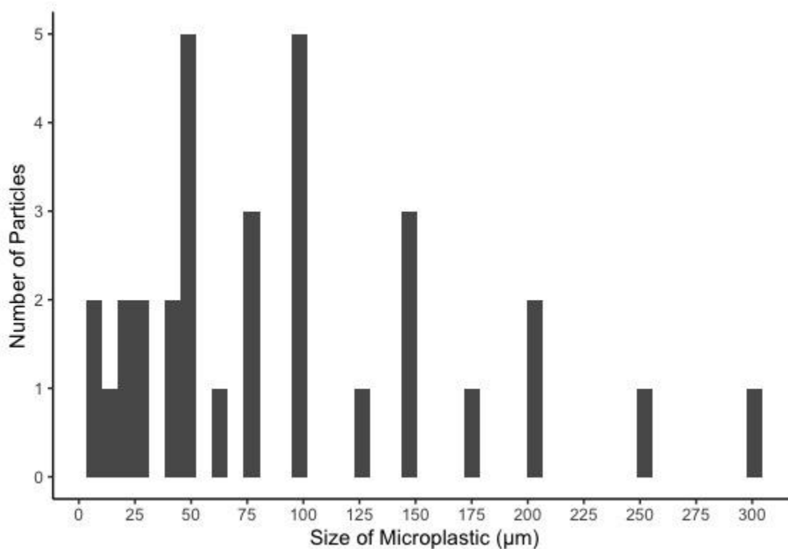
Figure 13. Distribution of the size (μm) of microplastic particles isolated from killer whale fecal samples and analyzed using Raman microspectroscopy.
