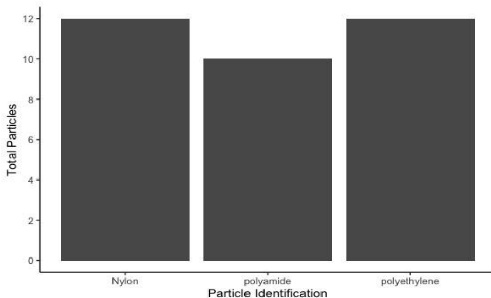
Figure 11. Verification and identification of microparticles polymer type from killer whales' fecal samples using Raman microspectroscopy. Microparticles identified as fluorescence may or may not be synthetic, these were unable to be identified due to fluorescence interference.
