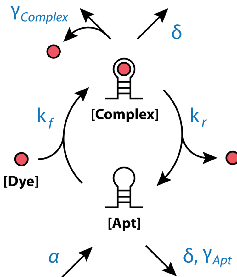
Figure 5.3. A system model for the molecular interactions of MGA5S. Aptamer concentration is affected by synthesis, degradation, dilution, binding, and unbinding events.
