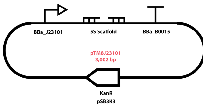
Figure 4.5. SBOL diagram of the no-apramer control plasmid. The core, 38-nucleotide aptamer sequence was removed from MGA5S.
