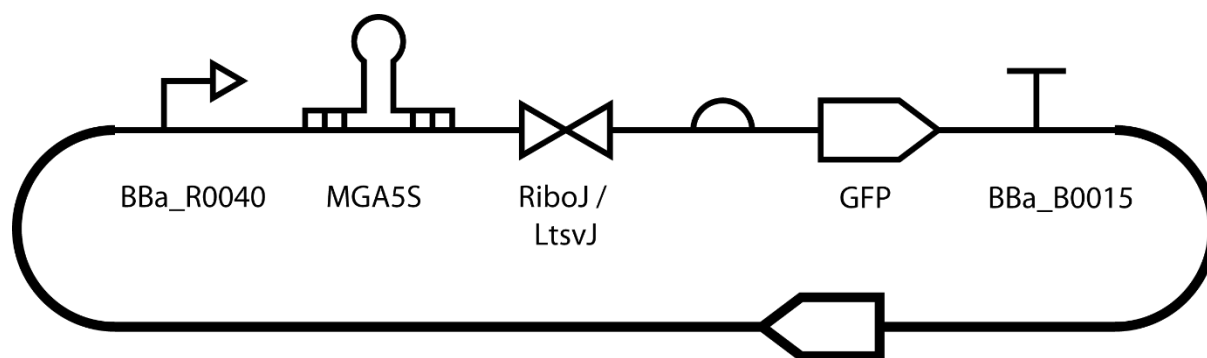
Figure 7.14. SBOL diagram of synthetic gene networks that utilize cis -cleavage to separate aptamer and protein-coding domains.
