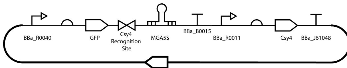
Figure 7.6. SBOL diagram of Csy4-cleaved RNA gene network design. MGA5S was placed downstream of a GFP coding sequence. Additionally, the GFP and MGA5S domains were separated by the 28 nucleotide Csy4 recognition sequence.
