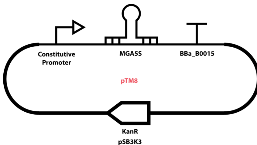
Figure 5.1. SBOLv diagram of the general strategy for expressing MGA5S in E. coli . Various constitutive promoters of differing strength were used to control MGA5S product within cells.
