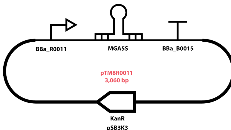
Figure 4.13. SBOL diagram of plasmid used to induce MGA5S expression with IPTG. BBa_R0011 is the IPTG-inducible promoter, placi.
