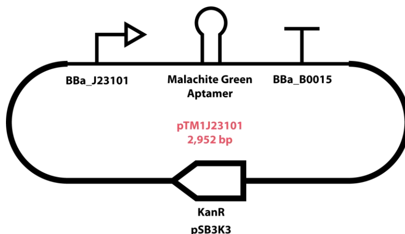
Figure 4.1. SBOL diagram for an initial attempt to express malachite green aptamer in E. coli .
