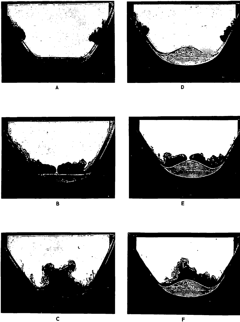
Figure 6. Convection currents produced in model experiments to simulate conditions of convective flow in the lake at the end of the meltwater stage (A-C) and at the present time (D-F).
