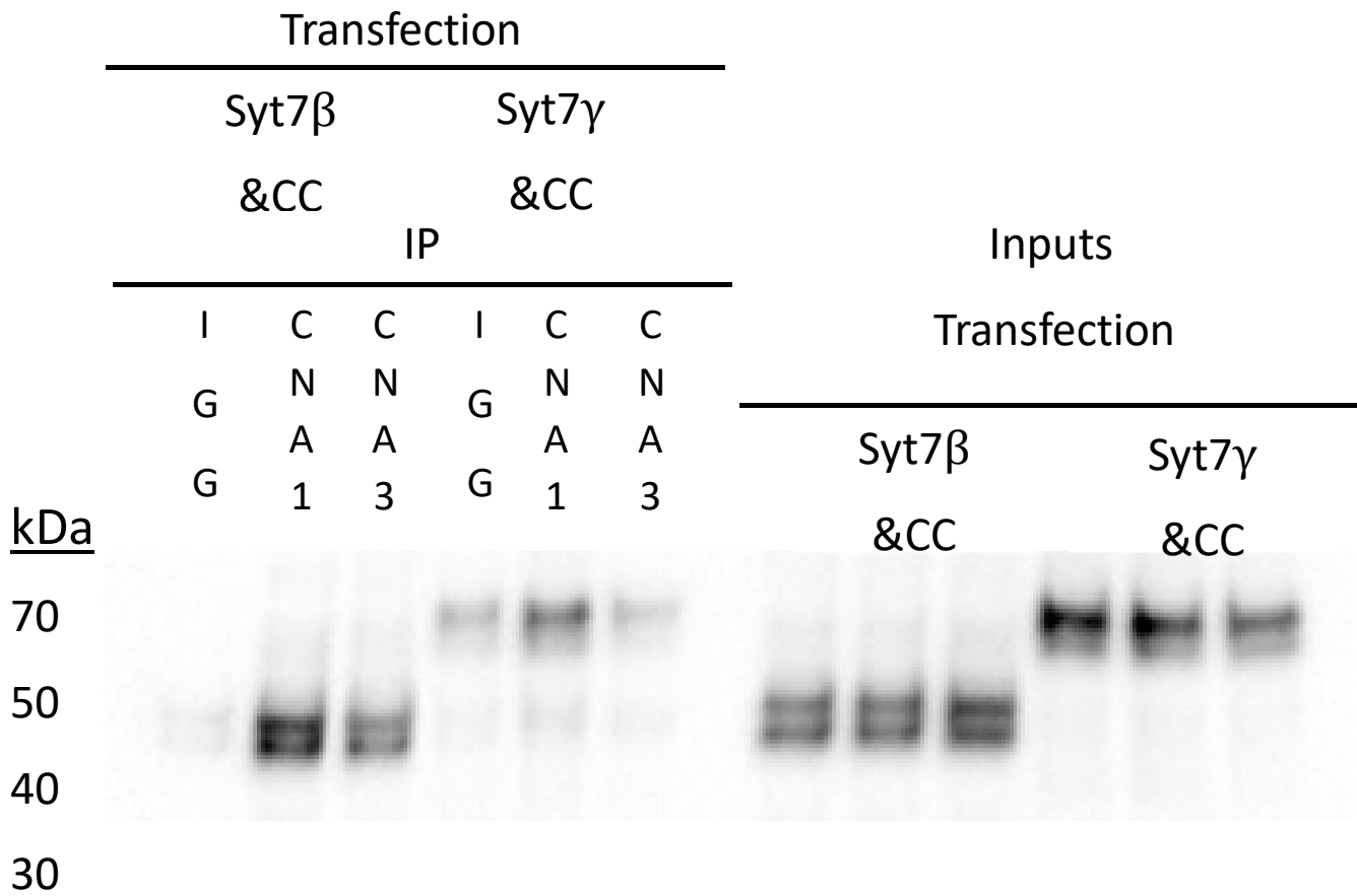
Supp. Fig. Across three separate experiments, all three neuronal isoforms of Syt7 independently co-precipitate with Cav2.1.
