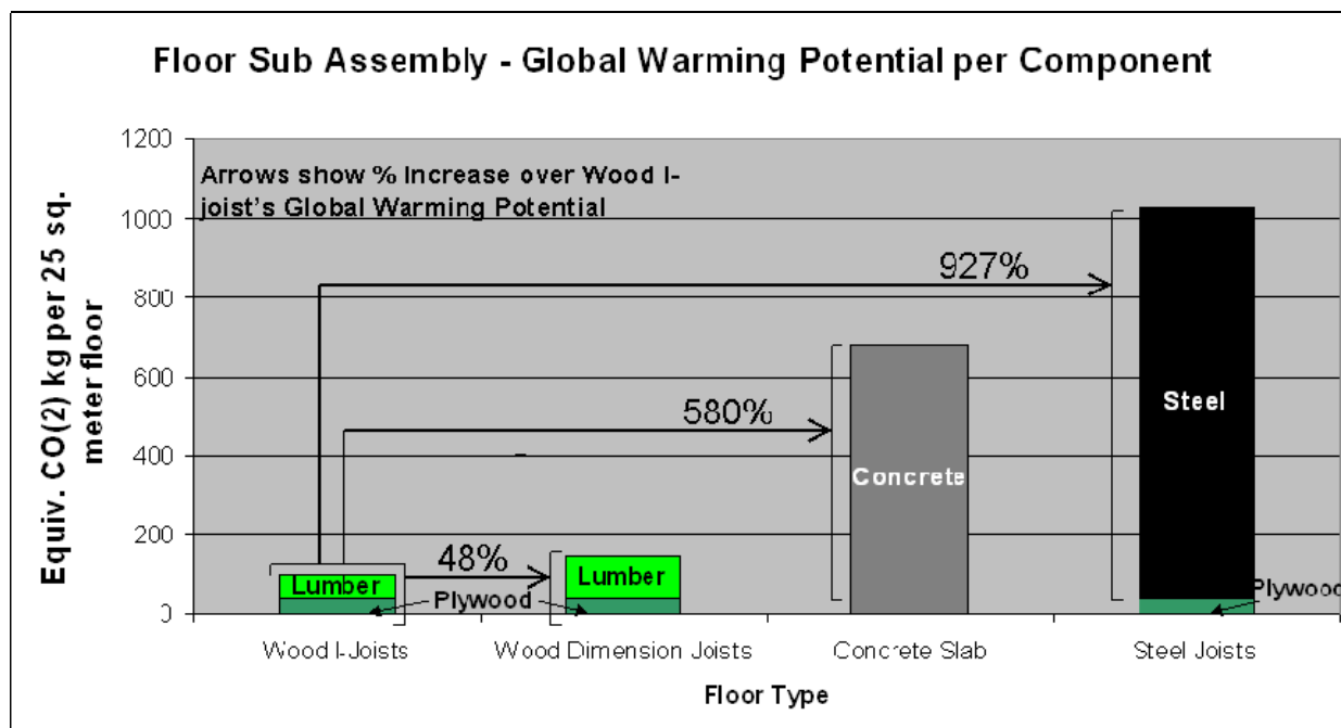
Figure 15. Comparison of global warming potential for floor sub-assemblies using different materials.
