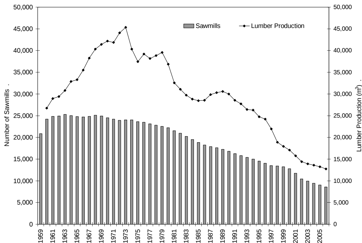
Figure 9. Number of sawmills and lumber production in Japan, 1959-2006.
