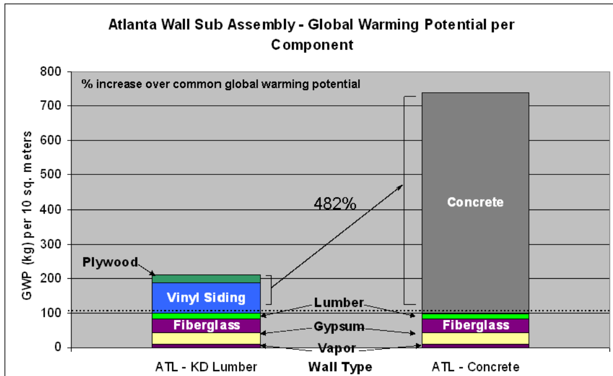
Figure 14. Comparison of global warming potential for wood framed vs concrete walls.
