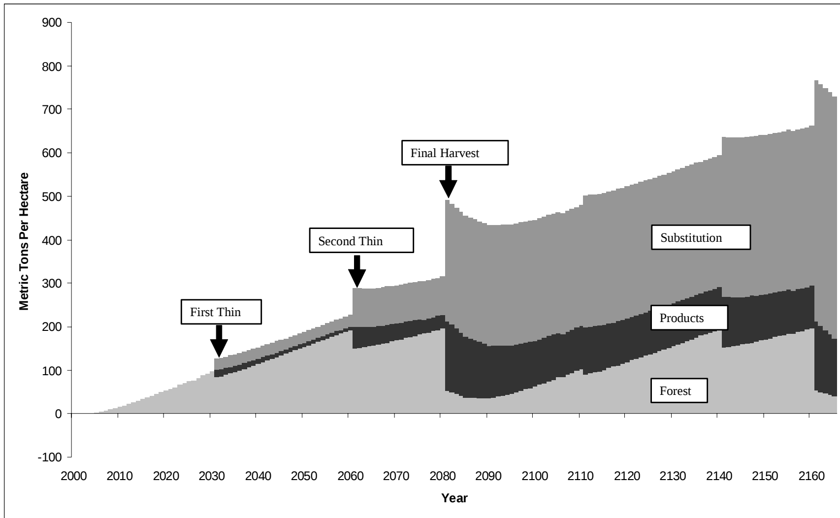
Figure 16. Carbon in forest, product, and substitution (avoided concrete) pools: 80-year rotation.
