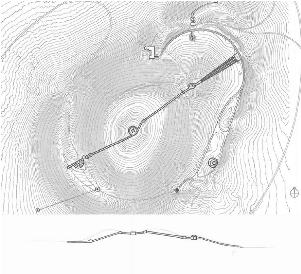
Figure 37: Roden Crater Plan and Section
