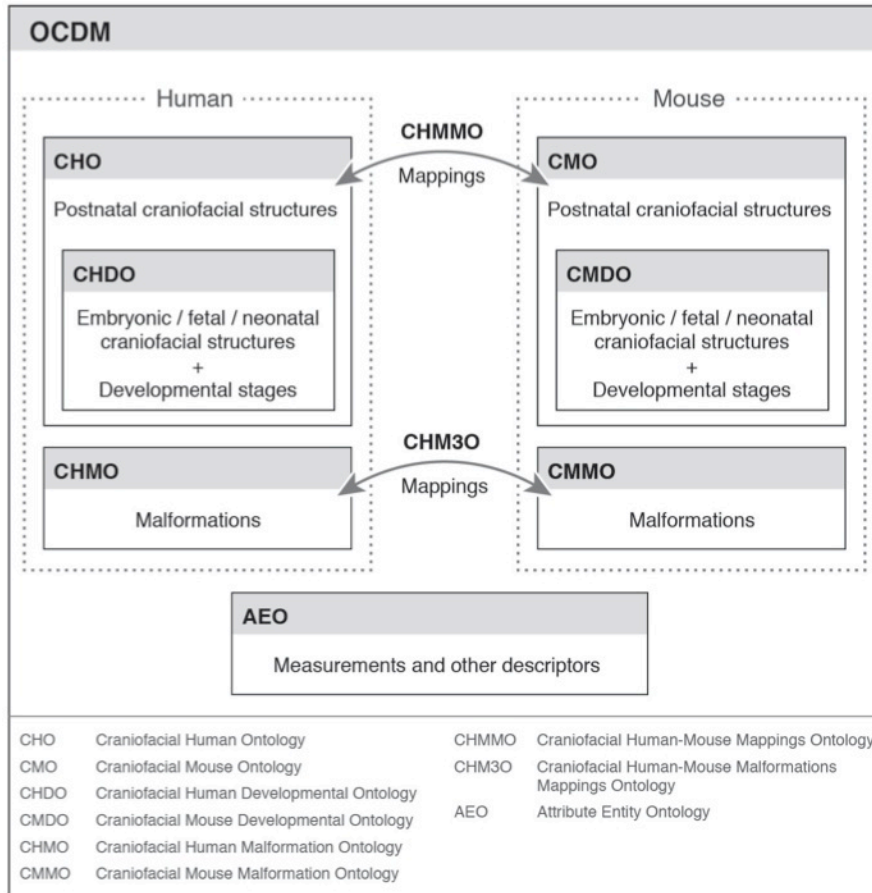
Figure 6-1. Overview of the sub-ontologies of the ODCM.
