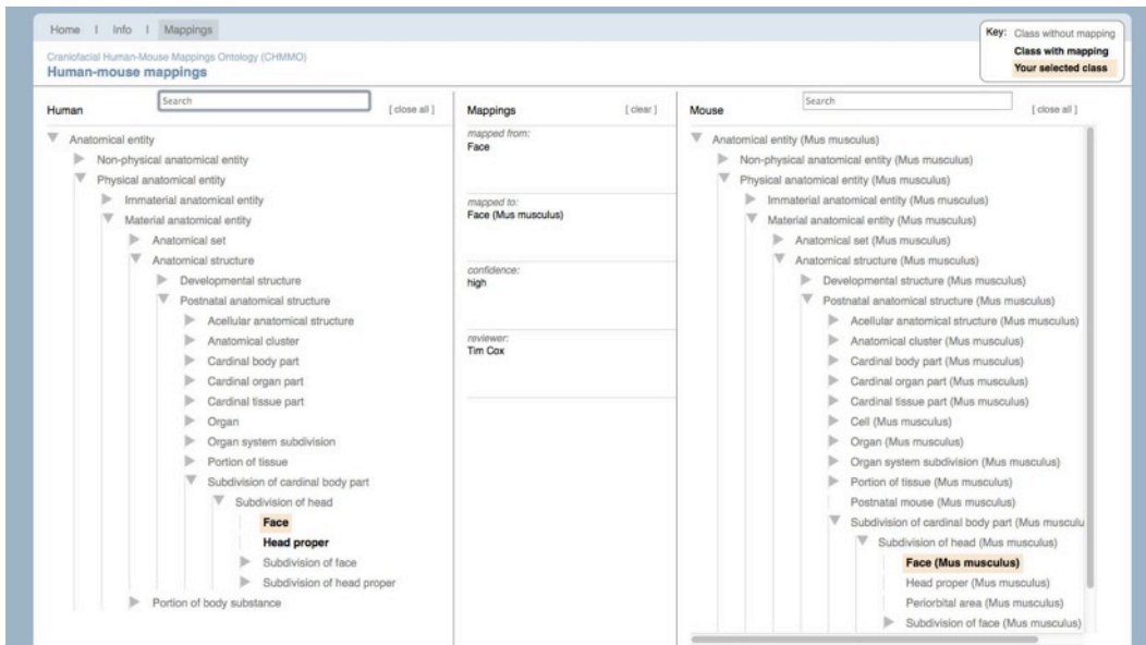
Figure 6-19. Screen layout for displaying mappings within the OCDM. The left and right panels are class hierarchies, with human on the left and mouse on the right. Classes with mappings are shown in bold (“Face” and “Head proper” in the human panel in this screen capture). The class “Face” has been selected in the human hierarchy, and its mapping properties are shown in the middle panel and the mapped class for mouse is highlighted in the left panel.
