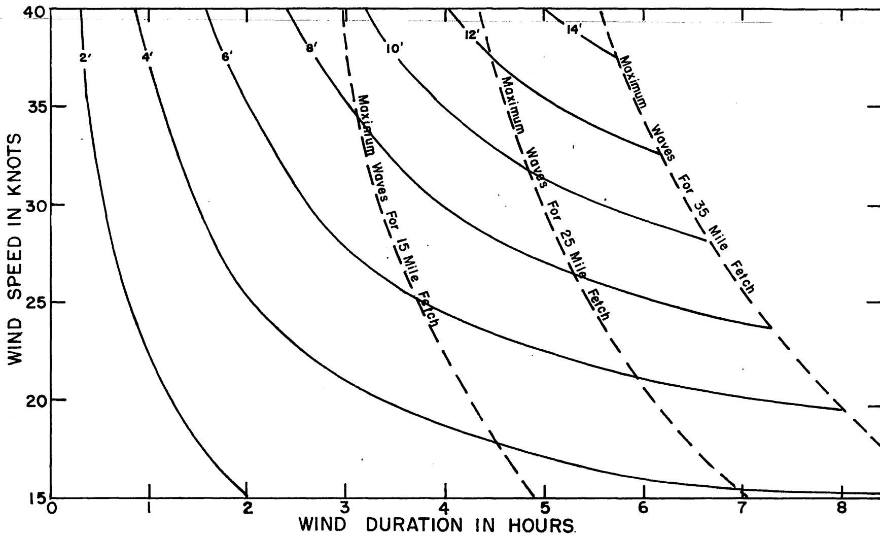
FIGURE 17. Wind wave height as a function of wind speed, duration of wind and length of fetch. Solid lines represent wave height in feet.
