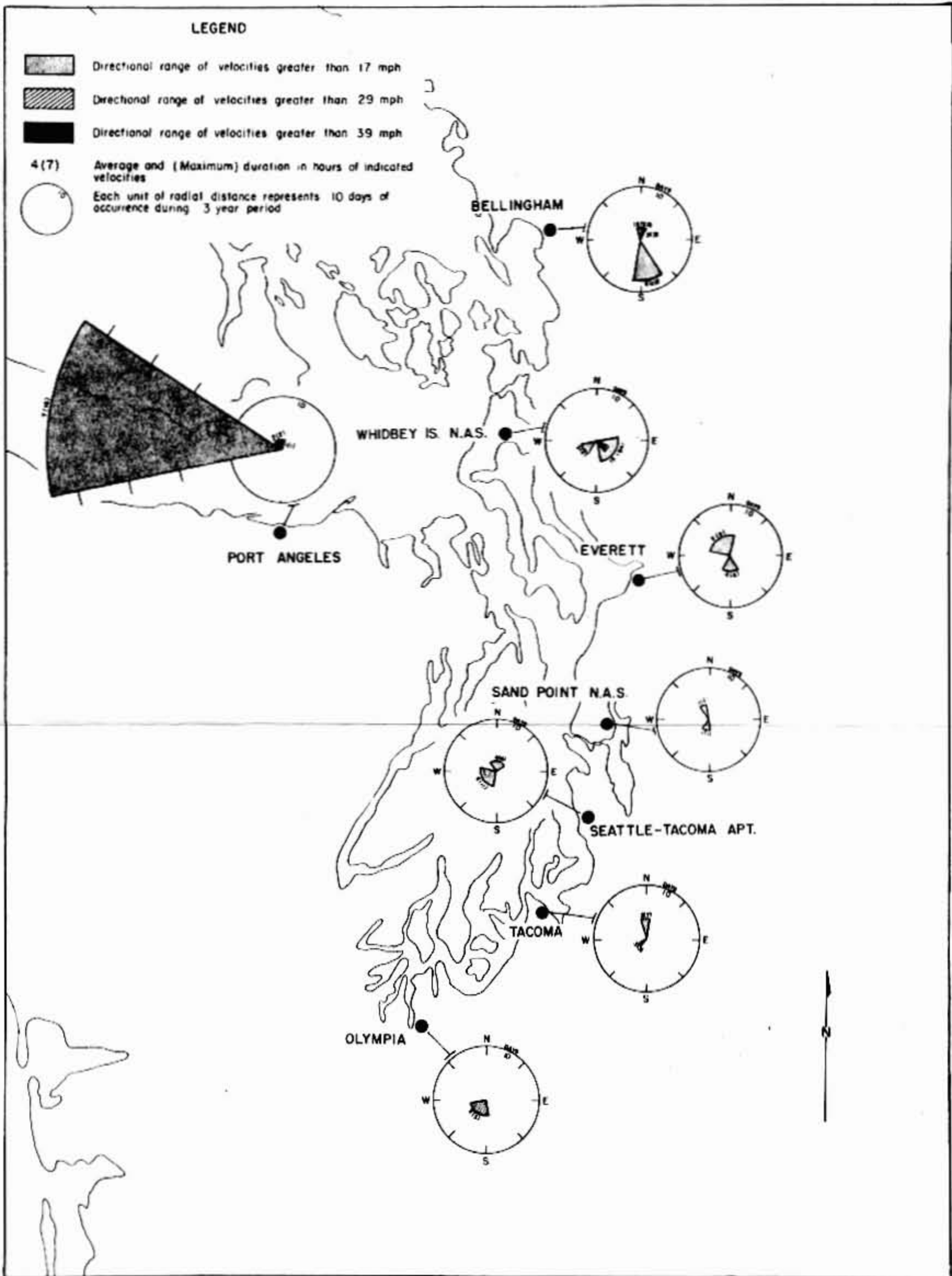
FIGURE 37. High surface wind frequency and duration - August.
