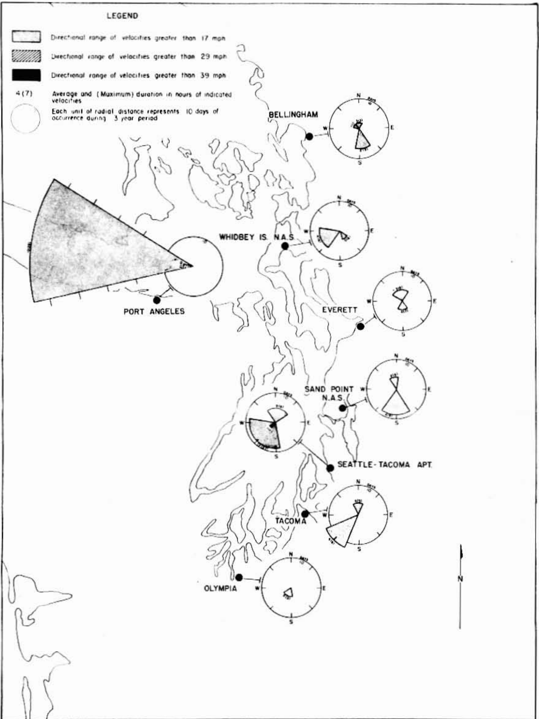
FIGURE 35. High surface wind frequency and duration - June.
