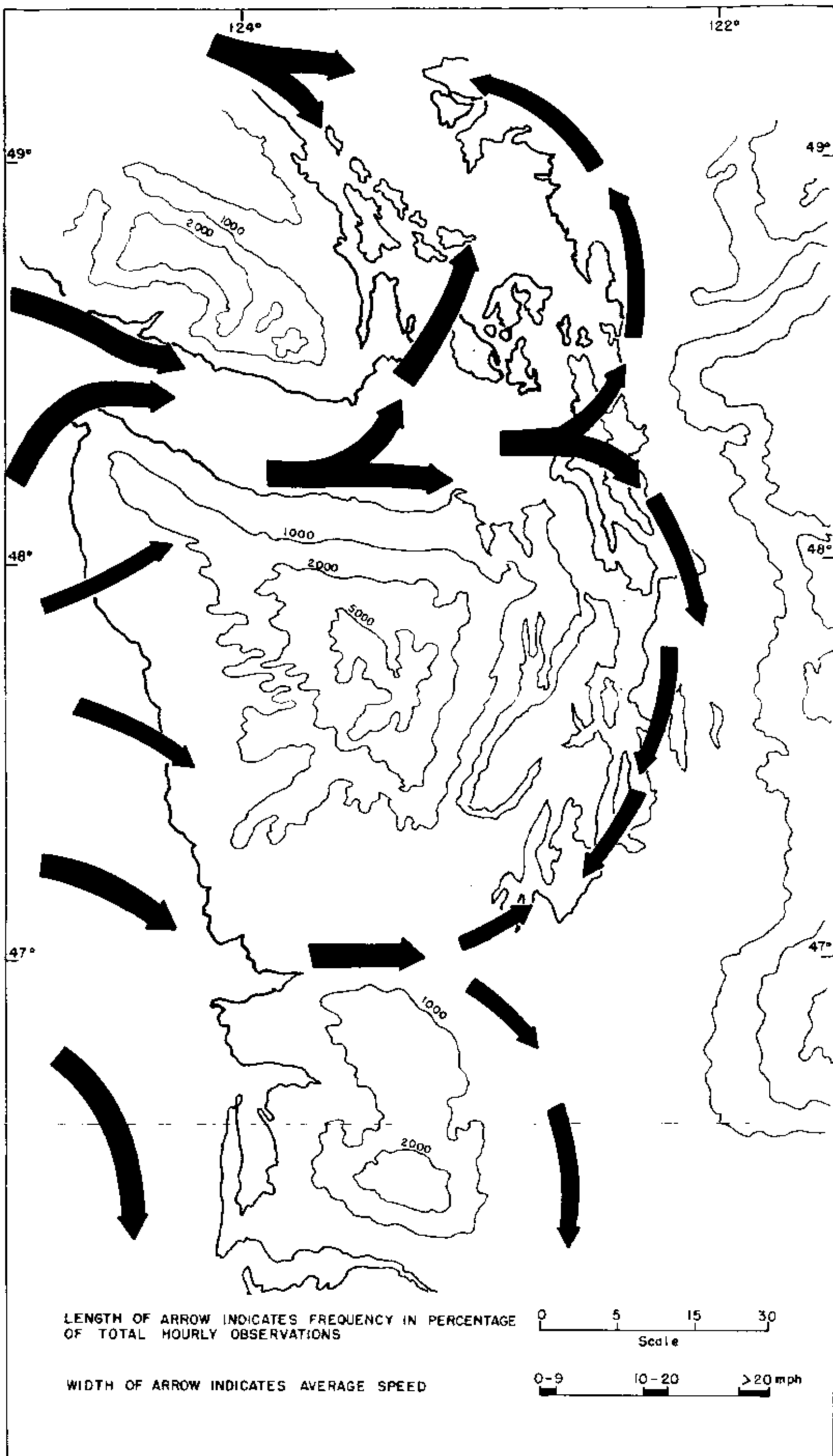
FIGURE 6. Prevailing surface winds: June - September.
