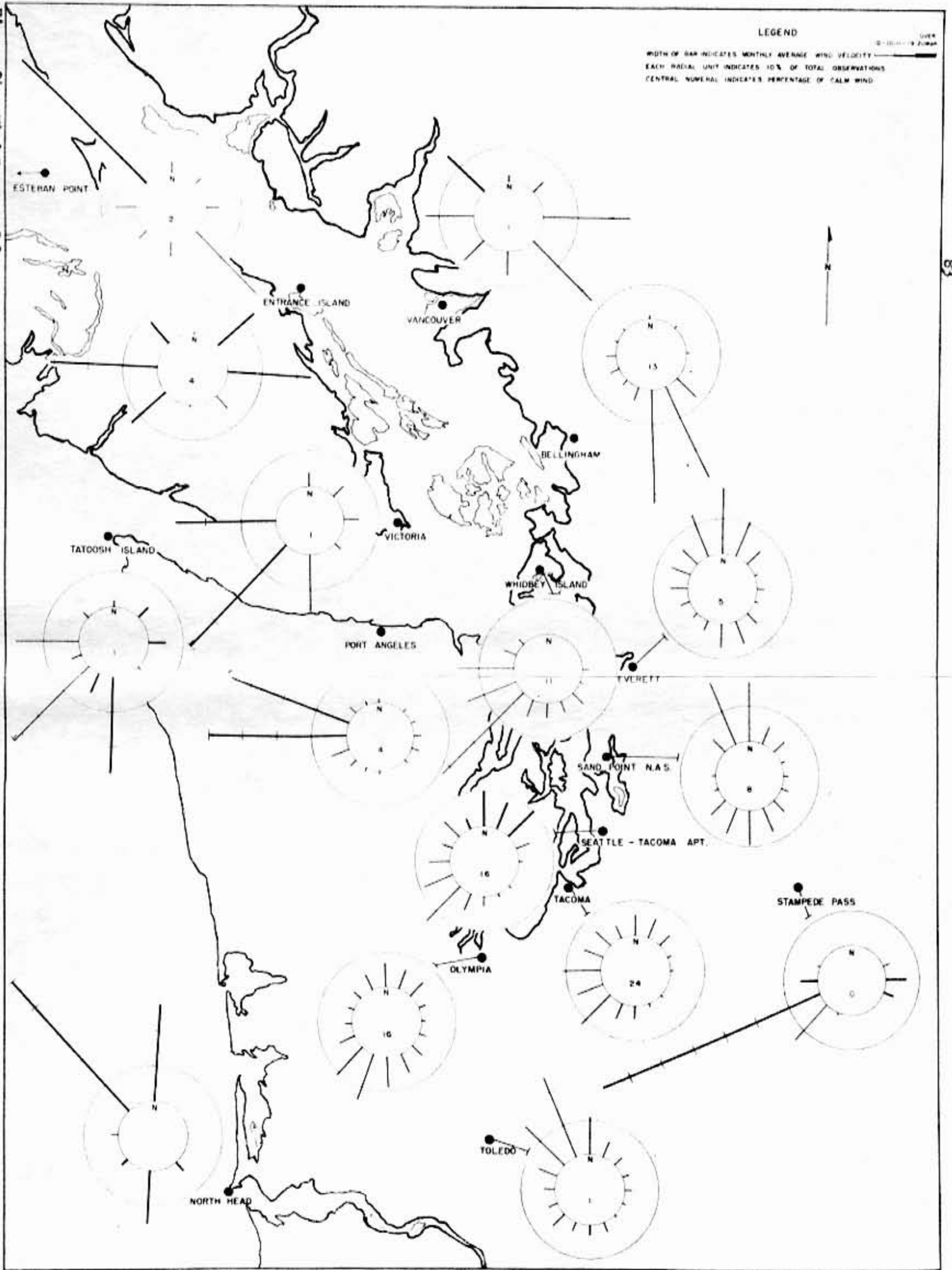
Figure 24. Wind Roses - July
