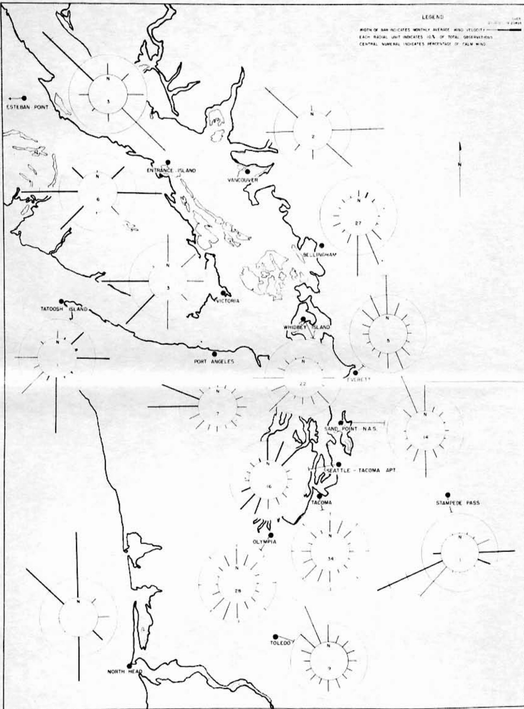
Figure 26 Wind Roses - September
