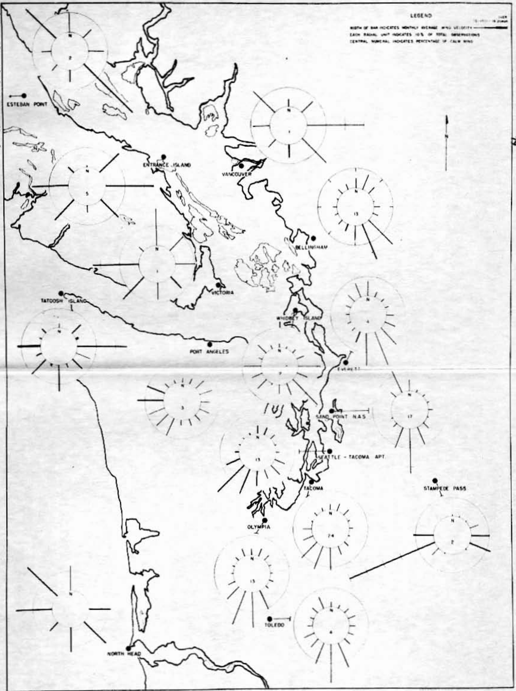
Figure 20 Wind Roses - March
