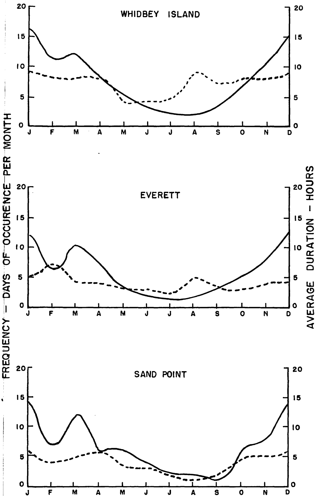
FIGURE 9. Frequency and duration of surface wind velocities over 18 mph (all directions). Solid lines represent frequency in days of occurrence per month. Dashed lines represent average duration in hours.
