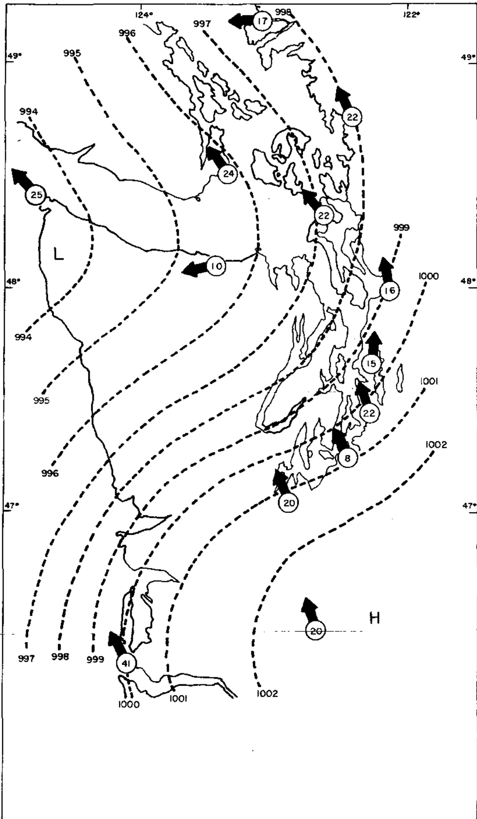
FIGURE 11. Surface wind flow 0400 PST, 2 January 1951. Dashed lines indicate barometric pressure in millibars. Arrow indicates surface wind direction. Circled numbers represent wind velocity in miles per hour.
