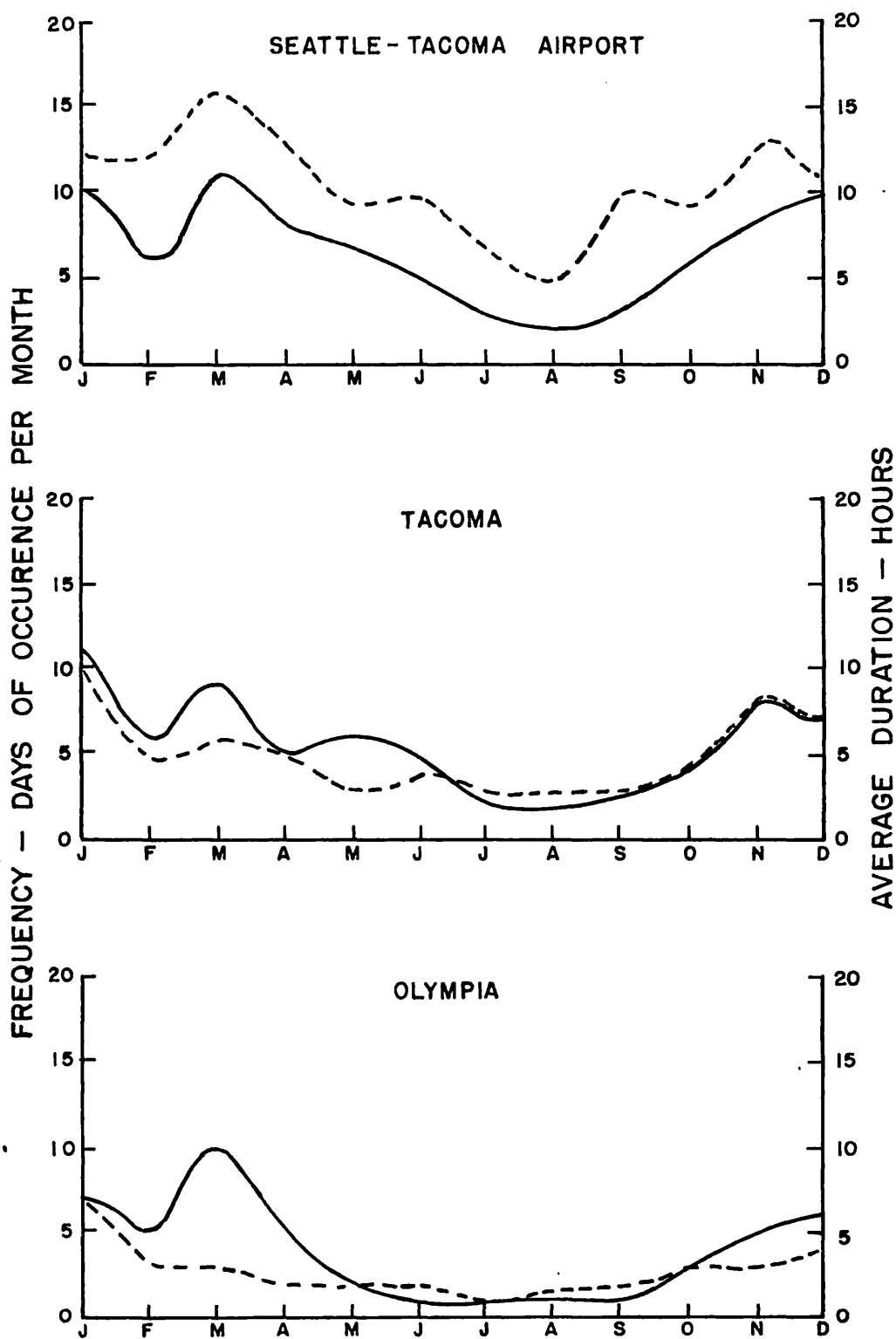
FIGURE 8. Frequency and duration of surface wind velocities over 18 mph (all directions). Solid lines represent frequency in days of occurrence per month. Dashed lines represent average duration in hours.
