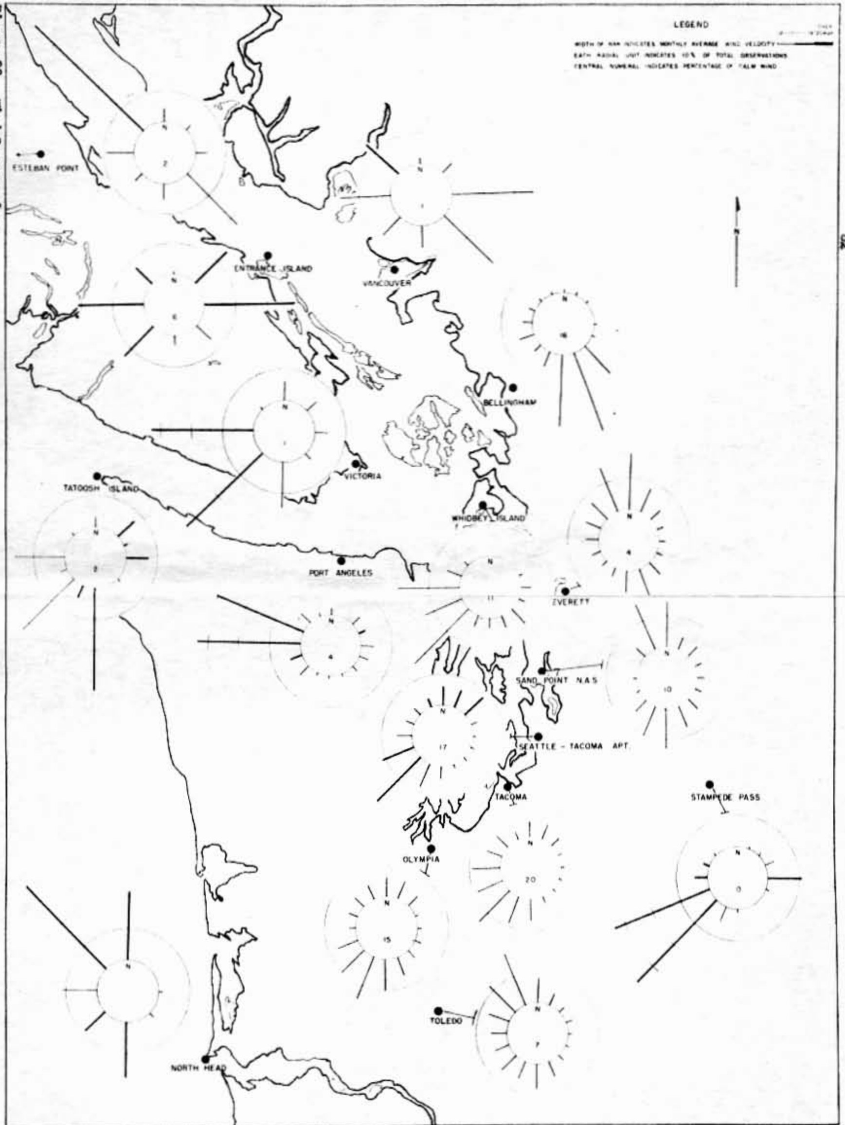
Figure 23 Wind Roses - June
