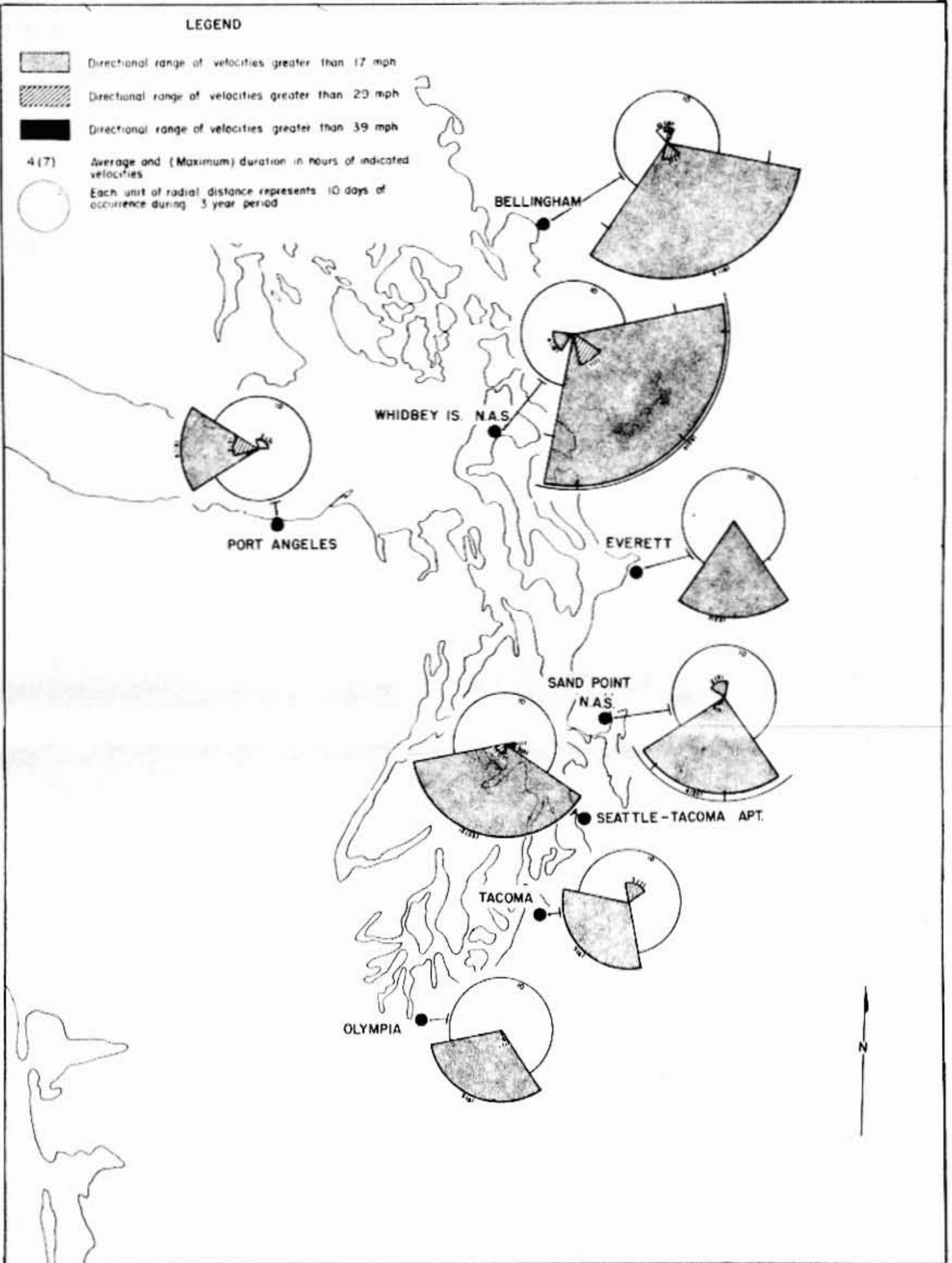
FIGURE 31. High surface wind frequency and duration - February.
