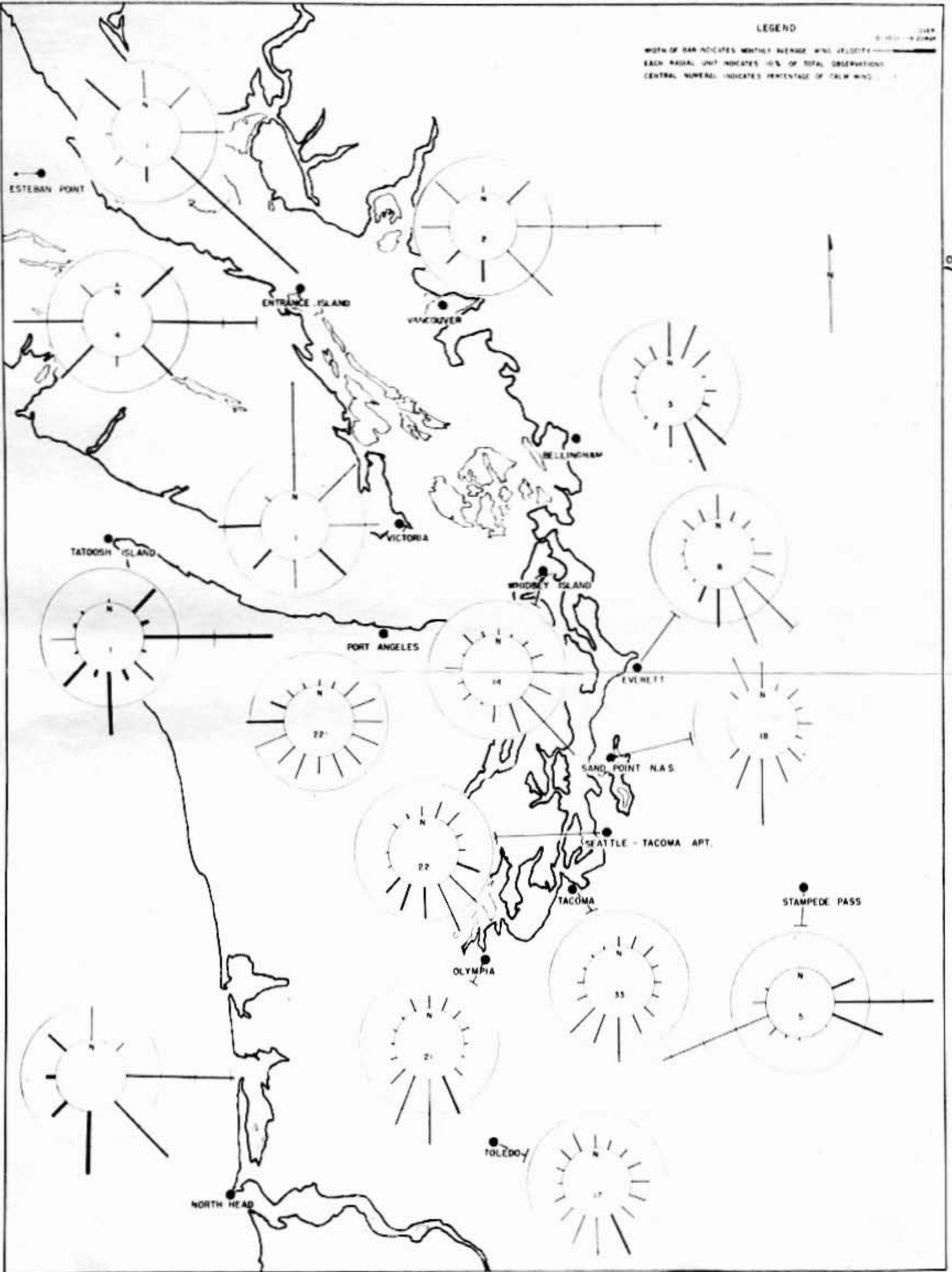
Figure 28 Wind Roses - November
