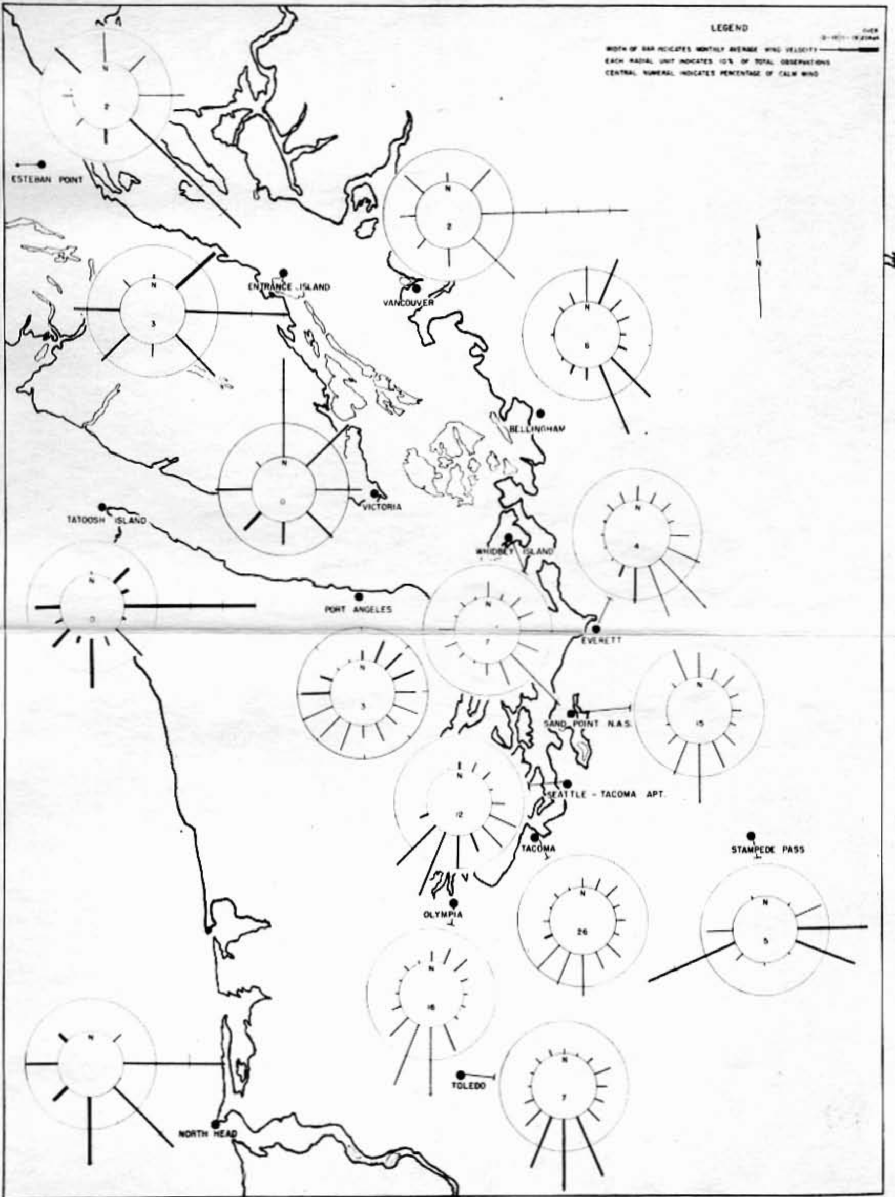
Figure 18 Wind Roses - January
