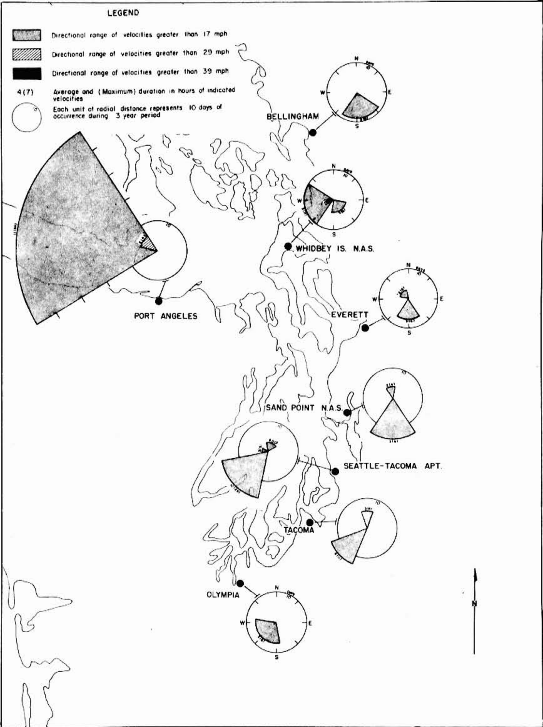
FIGURE 24. High surface wind frequency and duration - May.
