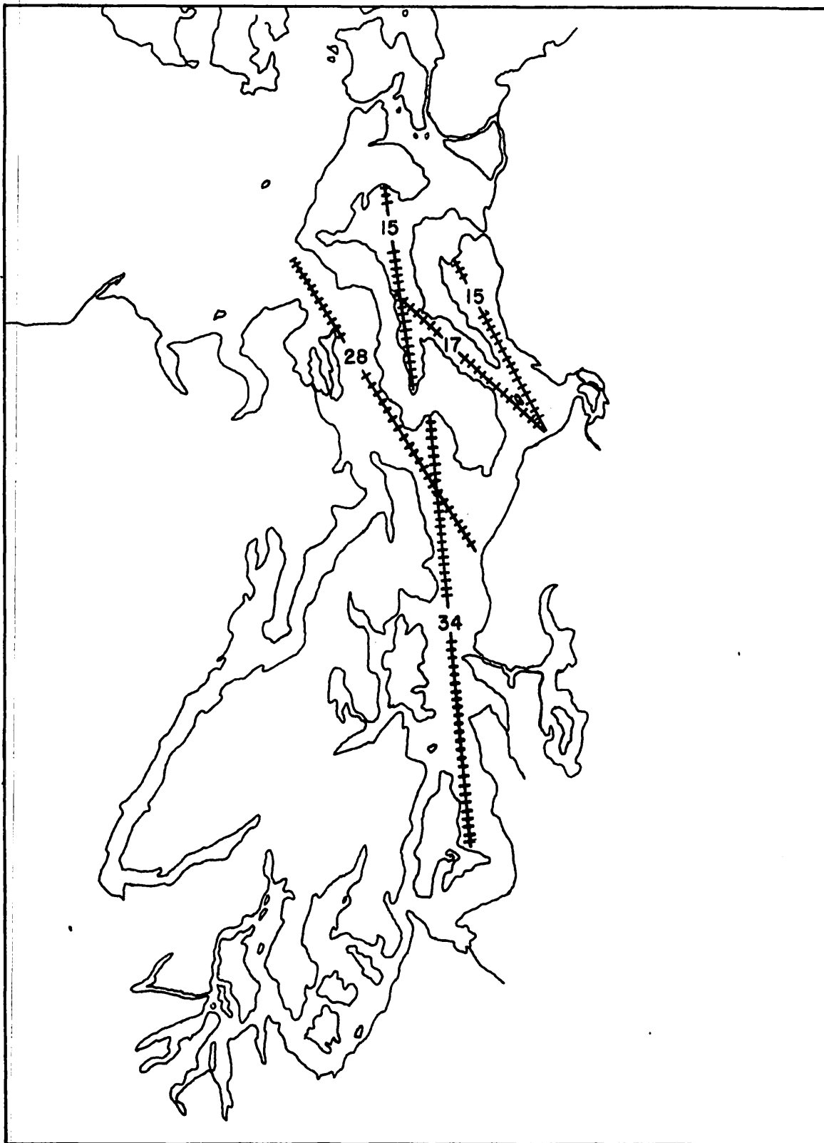
FIGURE 16. Fetch lengths on Puget Sound system. (in nautical miles).
