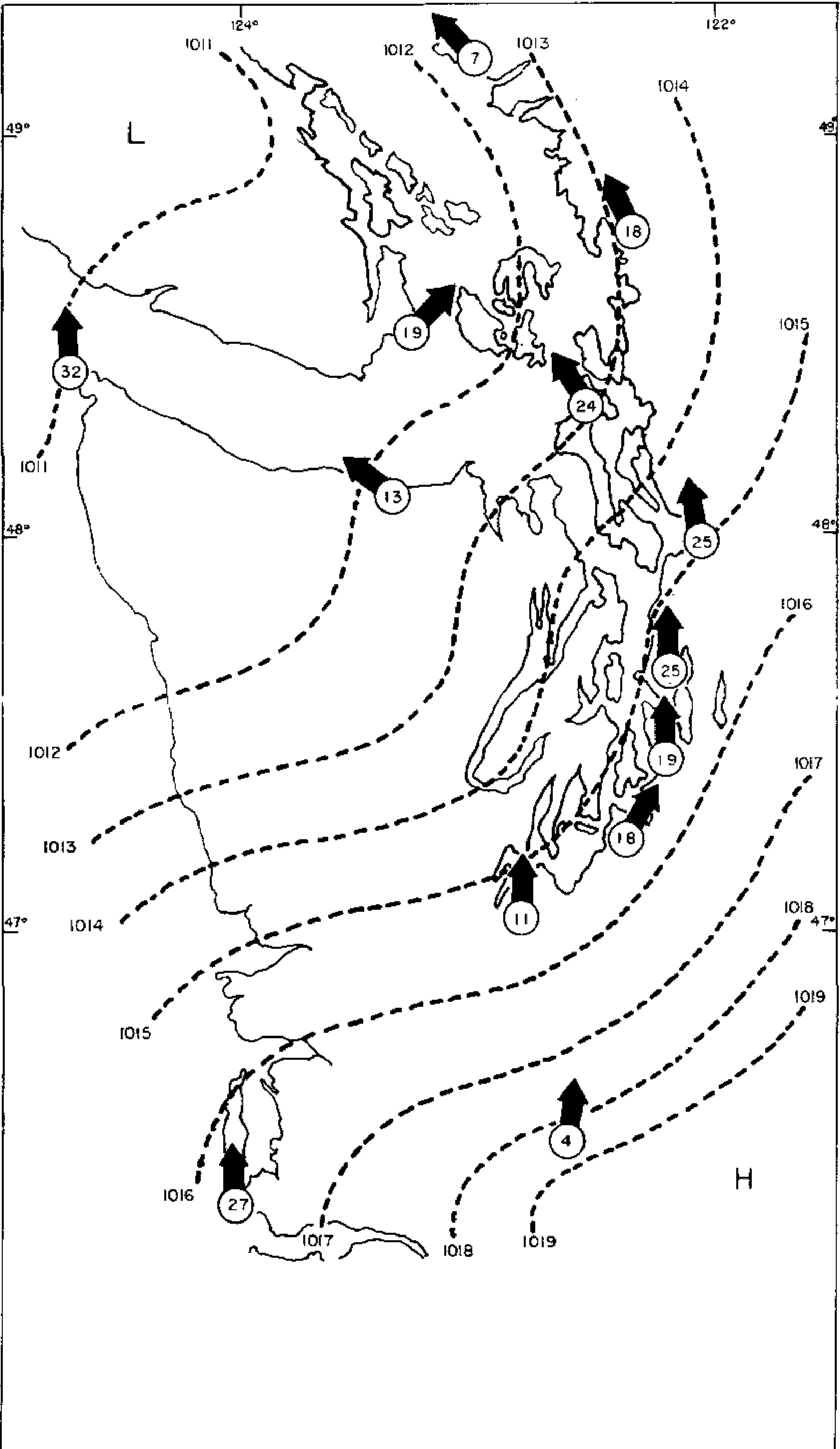
FIGURE 4. Surface wind flow 0600 PST, 25 January 1951. Dashed lines indicate barometric pressure in millibars. Arrow indicates surface wind direction. Circled number represents surface wind velocity in miles per hour.
