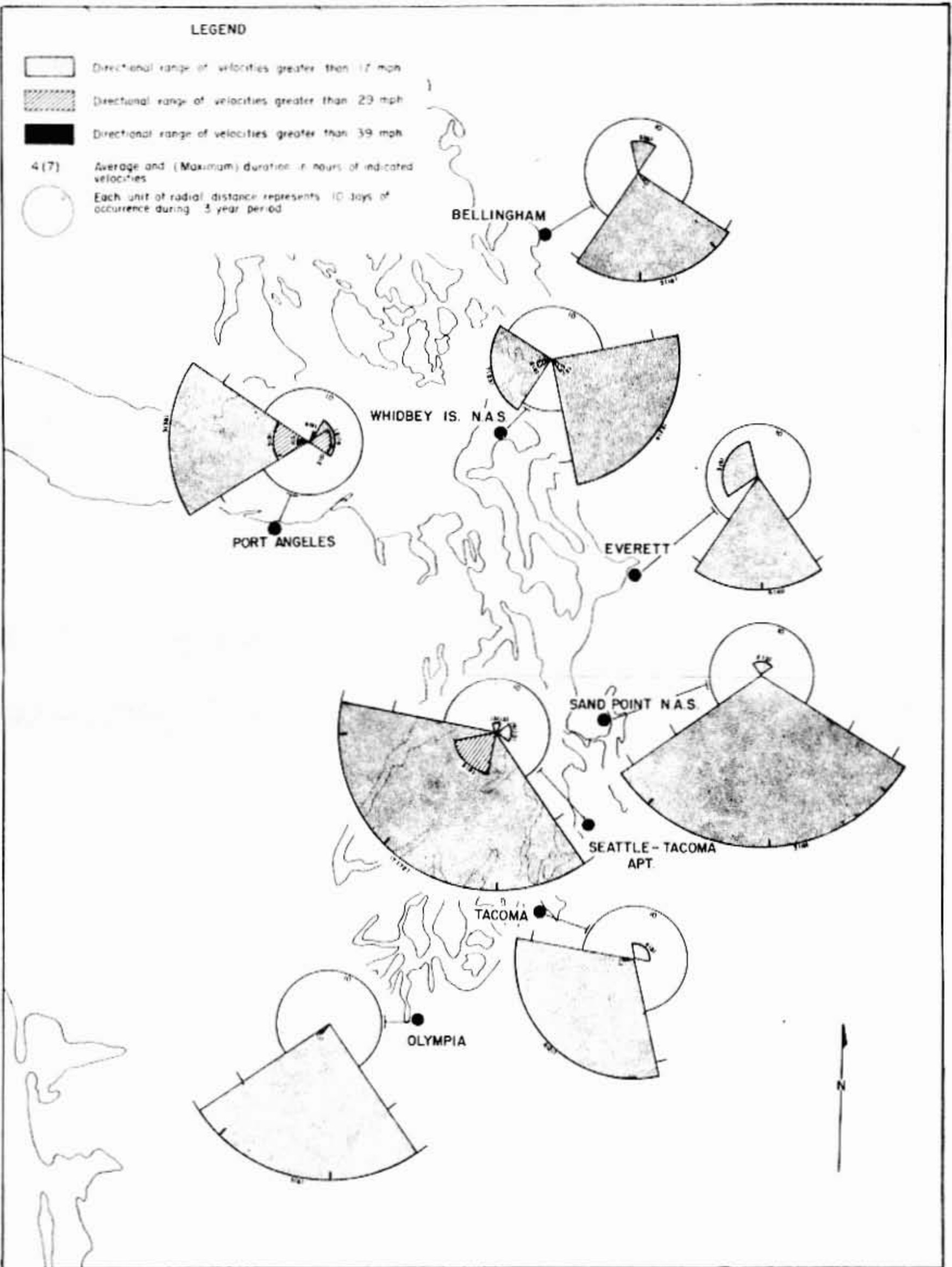
FIGURE 32. High surface wind frequency and duration - March.
