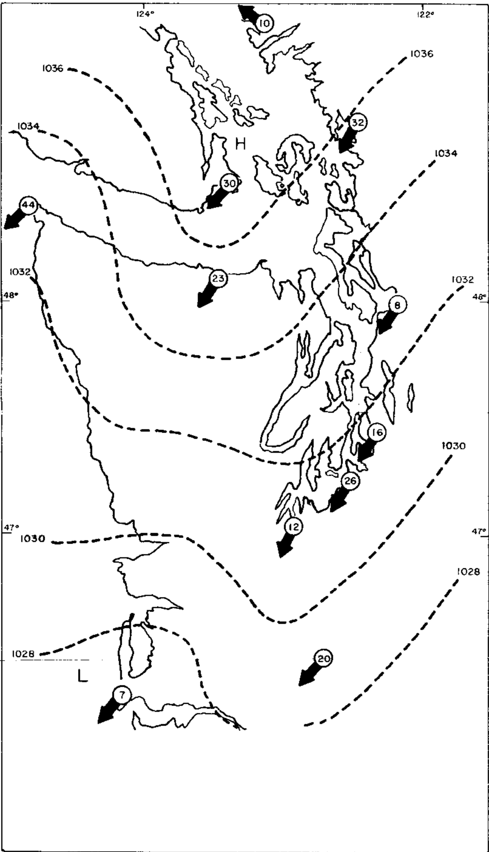
FIGURE 14. Surface wind flow OAOO PST, 28 January 1951. Dashed lines indicate barometric pressure in millibars. Arrow indicates surface wind direction. Circled number represents surface wind velocity in miles per hour.
