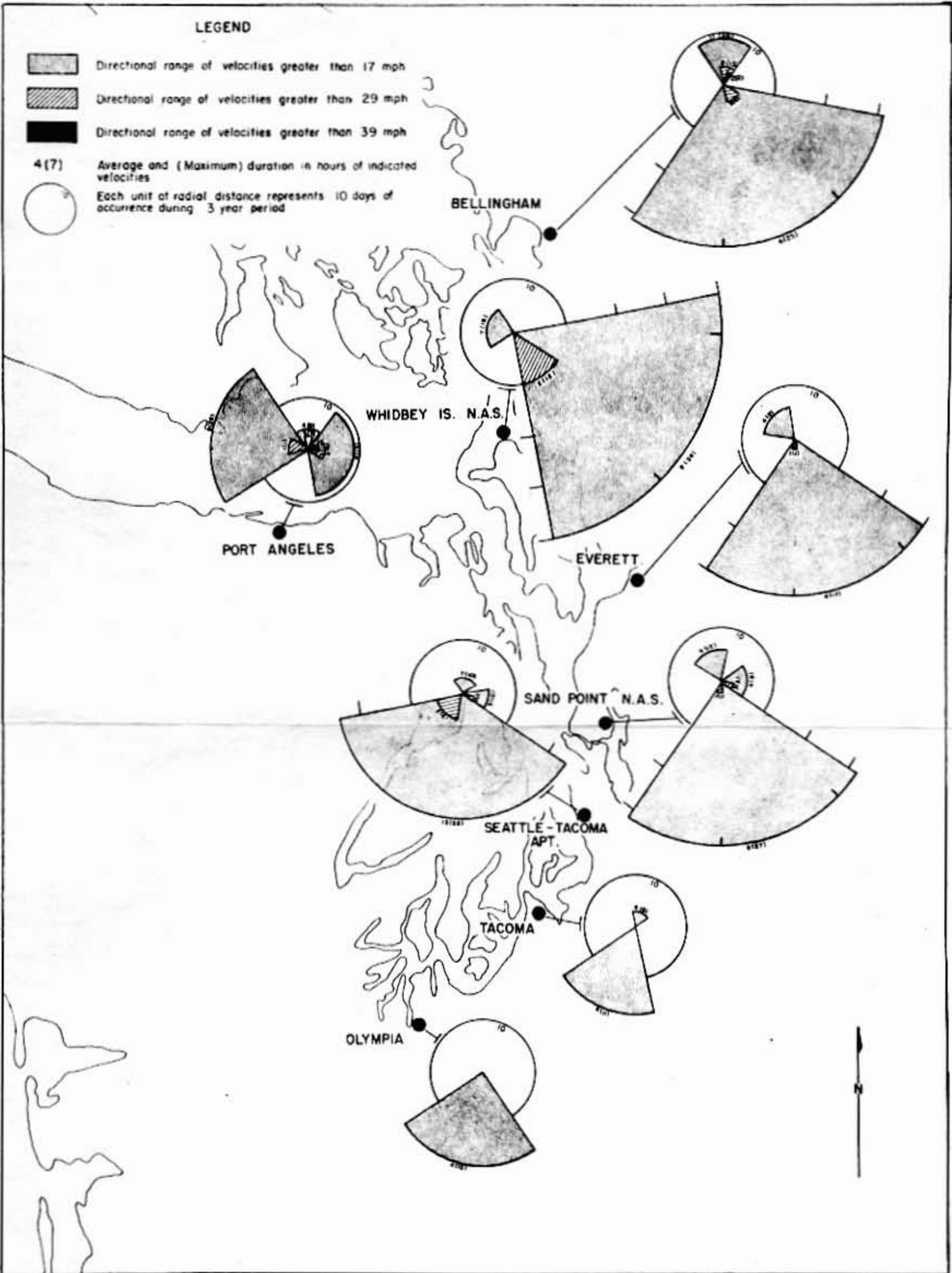
FIGURE A1. High surface wind frequency and duration - December.
