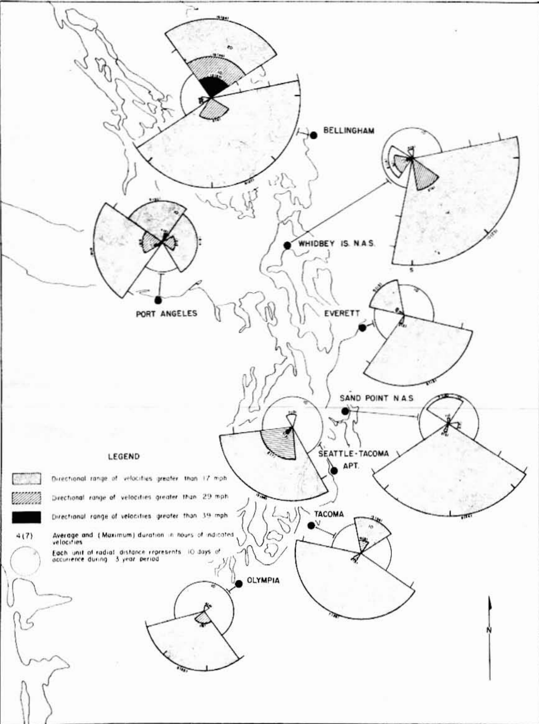
FIGURE 30. High surface wind frequency and duration - January.
