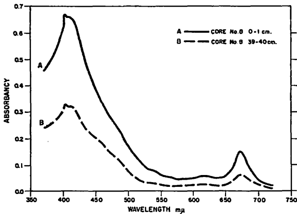
Figure 1. Absorption spectra of 90% acetone solutions of sediments.
