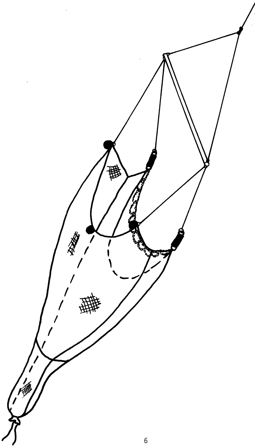
Figure 3. Diagram of the 3m beam trawl used to assess crab resources in Lummi Bay.
