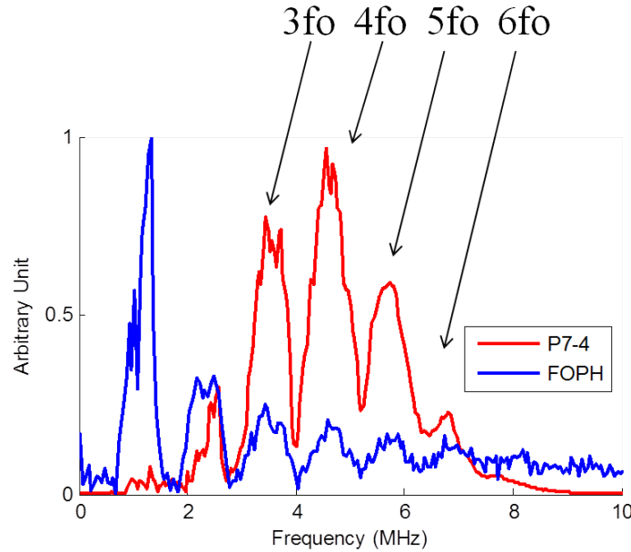
Figure 5.6 The two spectrums from FOPH and P7-4 received signal at 55.1MPa HIFU peak positive pressure are overlapped on the same harmonics. Both could detect up to 6th harmonic of the signal. The P7-4 has higher sensitivity from 4MHz to 7MHz. FOPH has a relatively constant sensitivity across the frequency range (0 to half of the sampling frequency, 20MHz)
