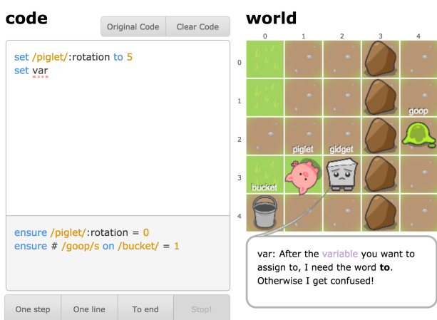
Figure 3.6. Gidget's syntax highlighting (left) and explanation of the error (right).
