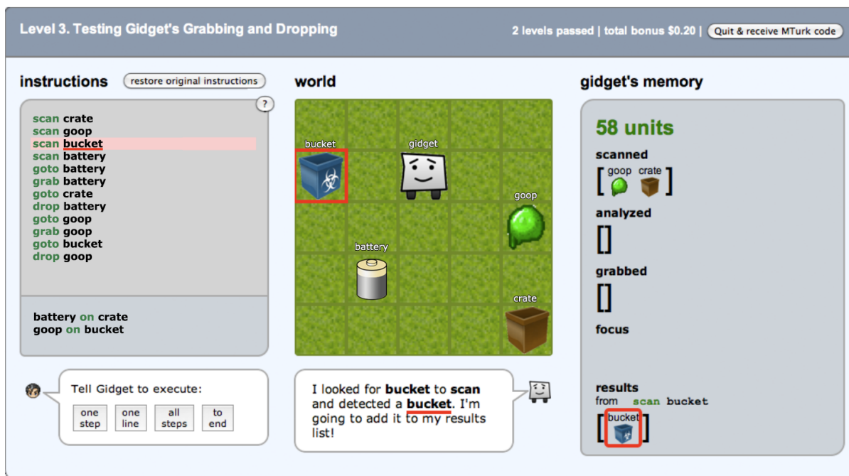
Figure 3.9. Screenshot of the first version of Gidget using the original language.
