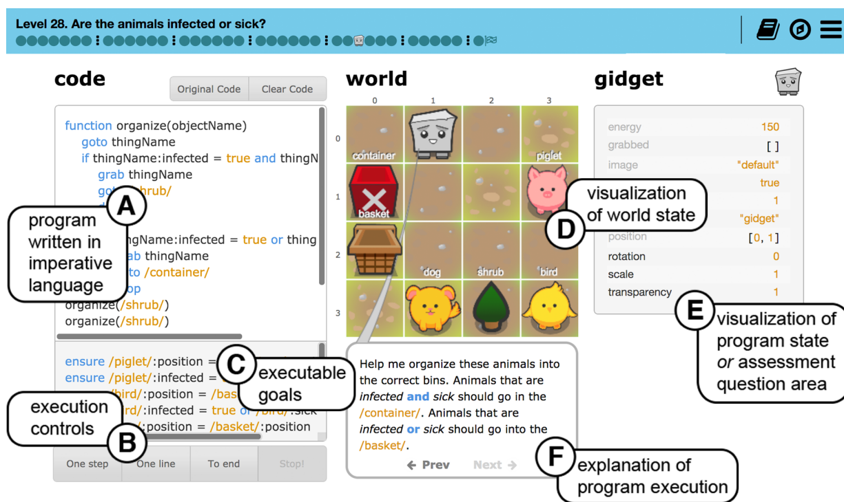
Figure 3.1. Screenshot of Gidget with added callouts on different interface elements.
