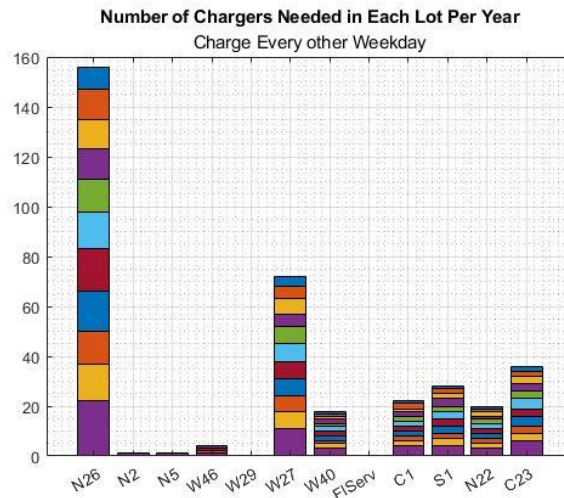
Figure 4.15. Chargers per Parking Lot Each Year for Case 7
