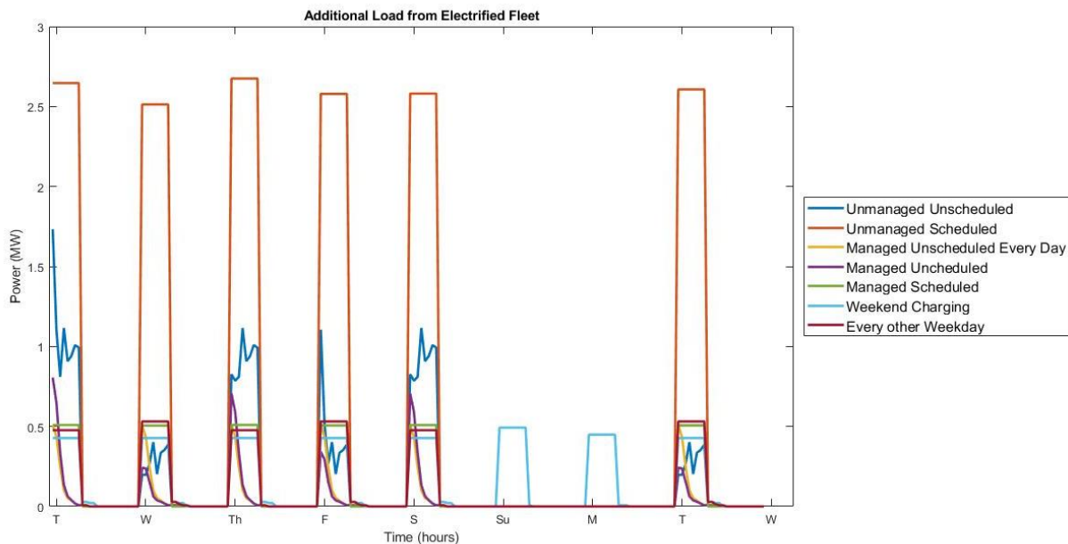
Figure 5.4. Electrified Fleet Hourly Load
