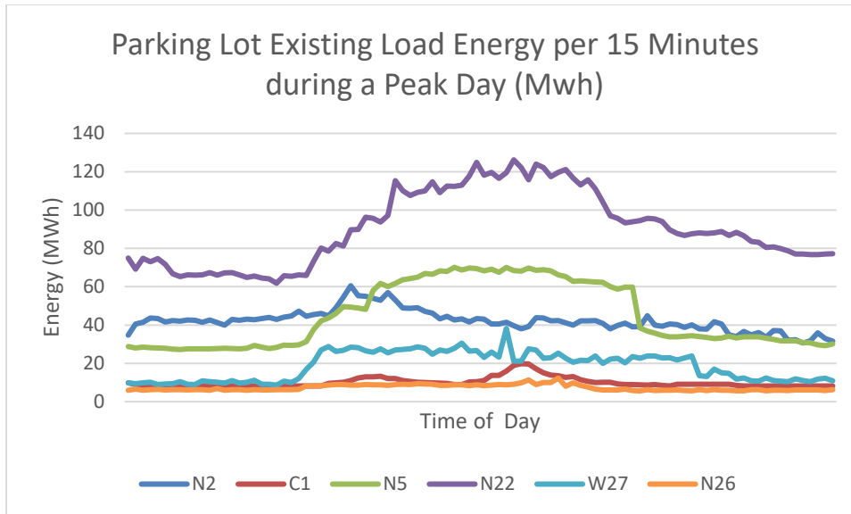
Figure 5.2. Parking Lot Existing Load Energy
