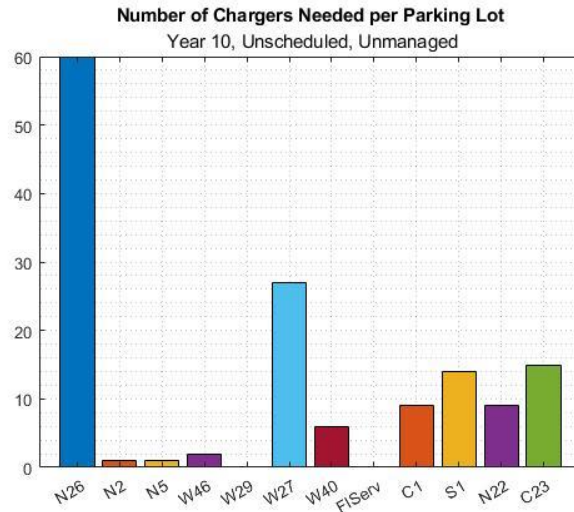
Figure 4.6. Year 10 Chargers per Parking Lot for Case 1
