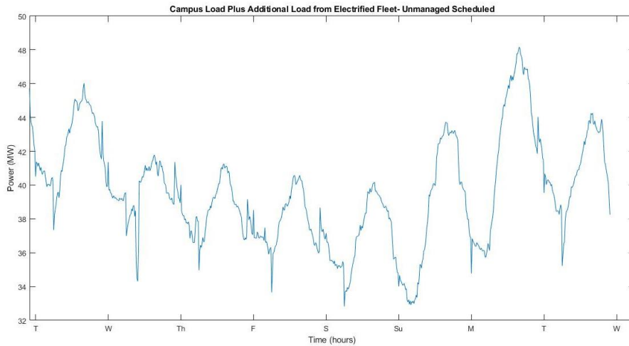
Figure 5.6. Total Load for Unmanaged Scheduled Charging
