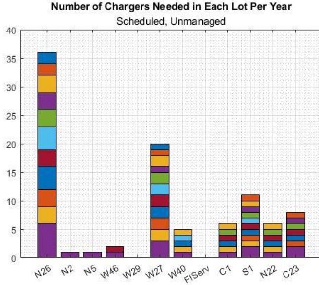
Figure 4.8. Chargers per Parking Lot Each Year for Case 2
