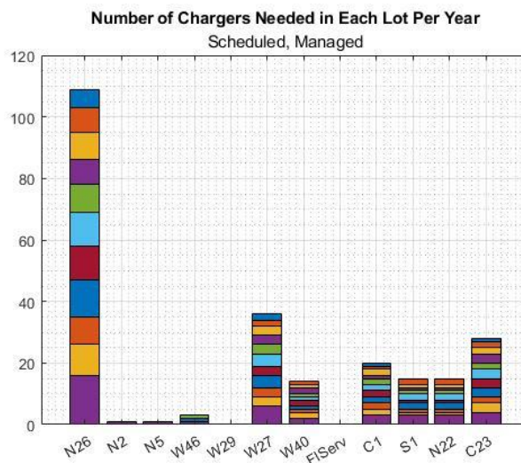
Figure 4.13. Chargers per Parking Lot Each Year for Case 5
