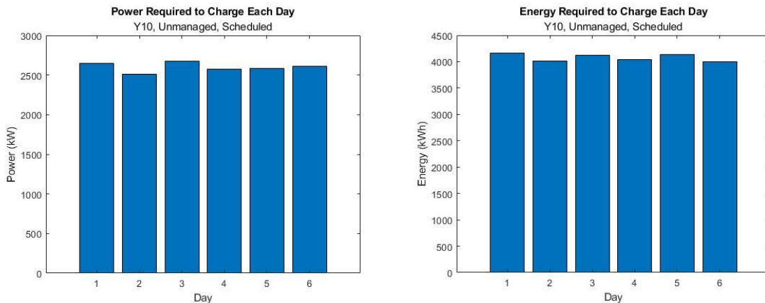
Figure 4.9. Year 10 Power and Energy Required to Charge Each Day for Case 2
