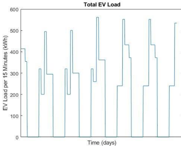
Figure 2.5. Power Schedule for the UW Transportation Electrified Fleet
