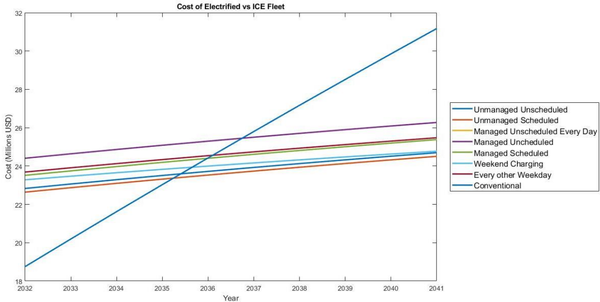
Figure 4.16. Costs of the Original versus Electrified Fleet
