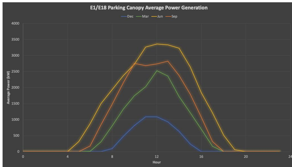
Figure 2.8. Average Power Generation from the E1/E18 Solar Canopy
