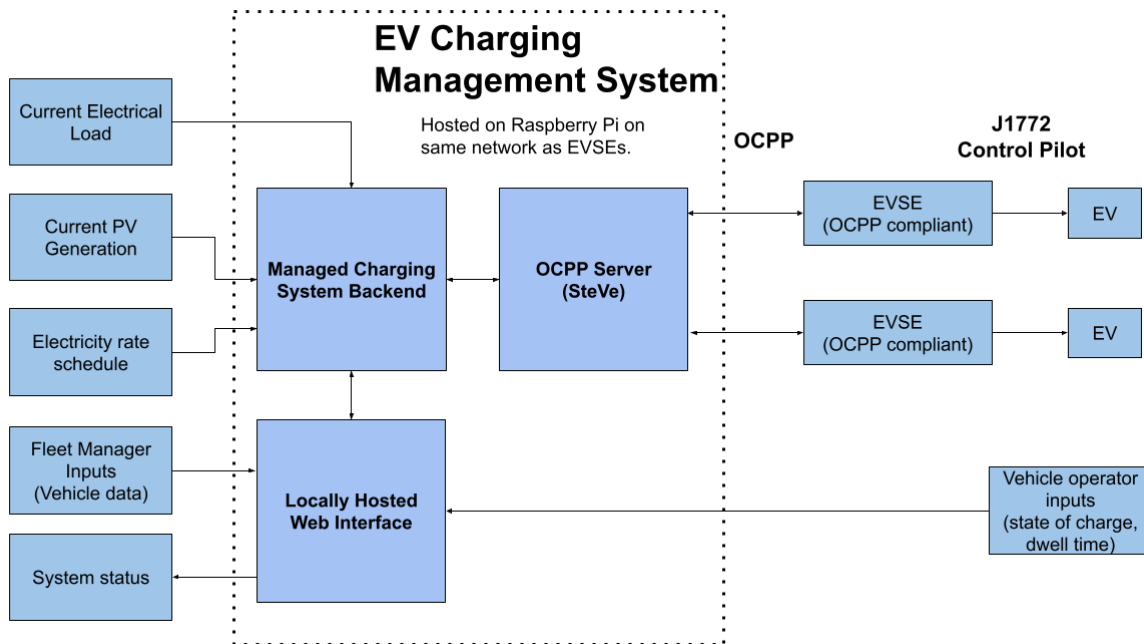
Figure 2.1. Software System Architecture
