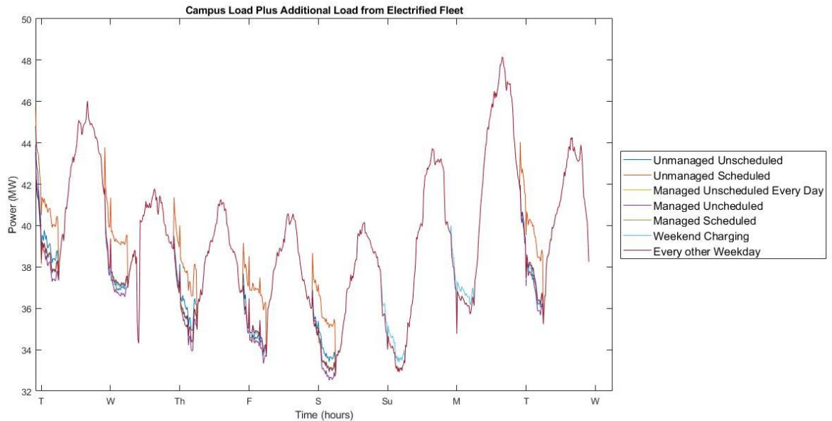
Figure 5.5. Total Hourly Campus Load Including Electrified Fleet Load
