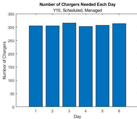
Figure 4.12. Year 10 Total Chargers each Day for Case 5
