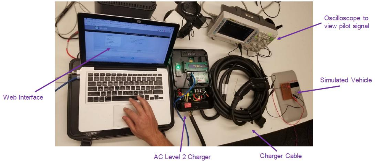
Figure 2.4. Capstone Test Setup
