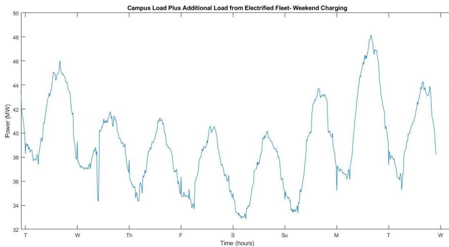
Figure 5.7. Total Load for Weekend Charging
