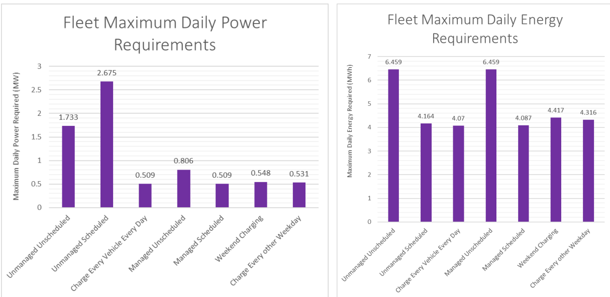
Figure 5.1. Power and Energy Requirements for Each Charging Scenario
