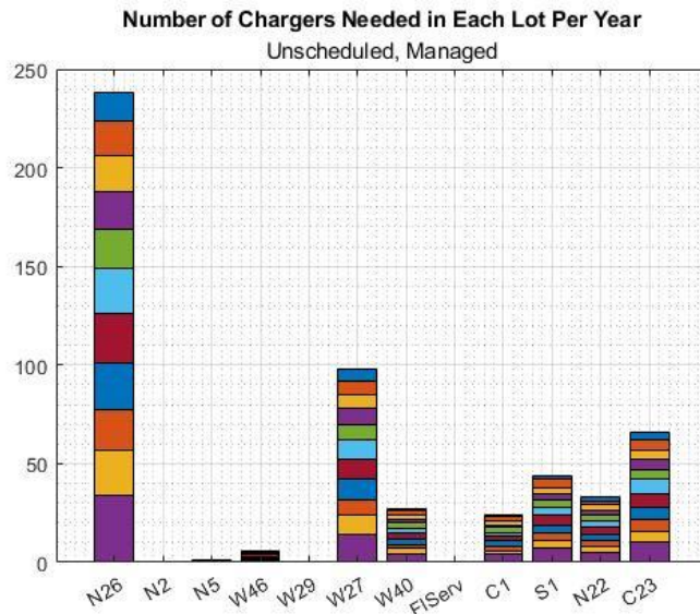
Figure 4.10. Chargers per Parking Lot Each Year for Case 3
