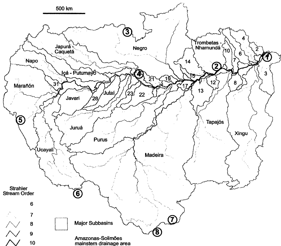
Figure 3.6. Amazon major subbasins and river network extracted from the drainage direction map. River reaches with a Strahler order of 6 and higher are shown. Each of the larger subbasins is labeled with the name of its mainstem(s); smaller basins are labeled with their subbasin numbers (see Table 3.1). Circled numbers indicate prominent hydrographic ambiguities and data problems: (1) Mouth of the Amazon, with multiple channels draining into the Ocean, bifurcations, small coastal catchments, and connection to the Tocantins river. (2) Combined Trombetas and Nhamundá confluence into the mainstem. (3) Linkage to the Orinoco Basin via the Negro-Casiquire connecting channel. (4) Bifurcation of the Japurá-Caquetá confluence into the mainstem. (5) Marañón headwaters mainstem dropped from the DCW network and reconstructed manually. (6) Apurimac source headwaters dropped from the basin. (7) Ambiguous hydrological connectivity in the Bañados del Izozog wetlands. (8) Iteñez headwaters in the Itonamas-Parapeti river dropped from the basin.
