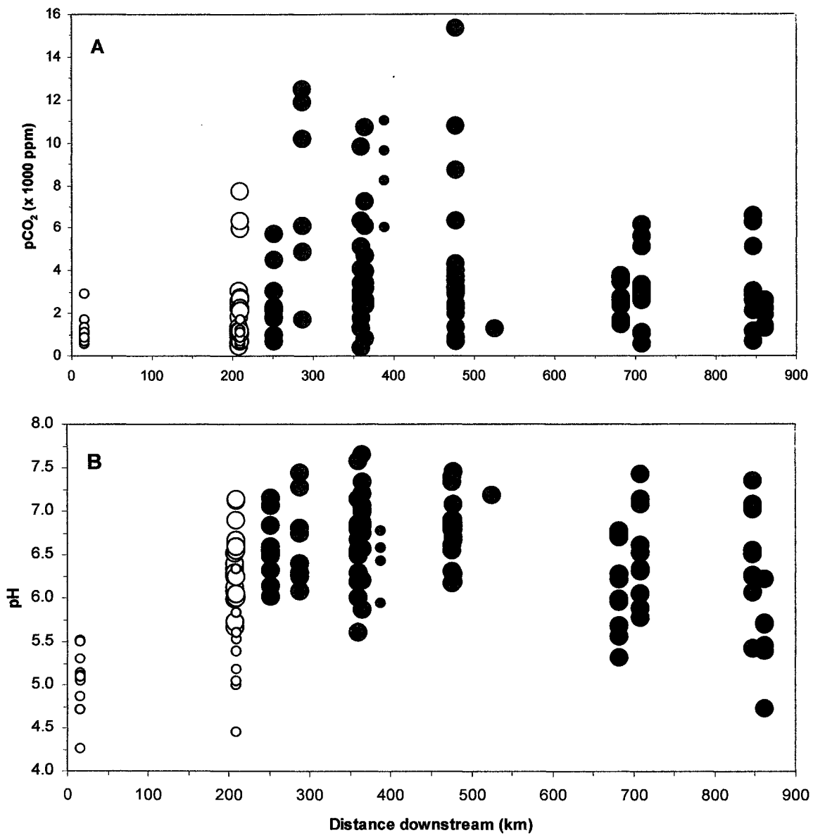
Figure 6.10. Downstream p\text{CO}_2 and pH evolution in the Ji-Paraná basin. Symbology is the same as in Fig. 6.8. A) p\text{CO}_2 . B) pH.
