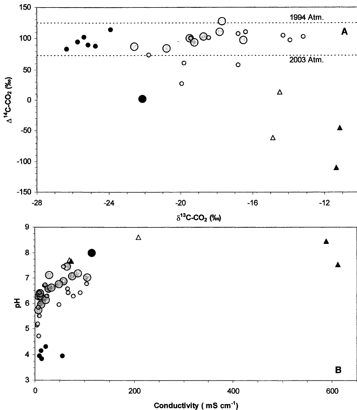
Figure 6.7. Sites with drainage area <9,000 km 2 . Symbology is the same as in Fig. 6.1, but size does not distinguish previously published data. Small symbols represent sites with drainage area <4,000 km 2 . A) \Delta^{14}\text{C-CO}_2 vs. \delta^{13}\text{C-CO}_2 . Two sites in the Andean headwaters of the Ucayali are not shown, as their \Delta^{14}\text{C} content is very low. Horizontal lines show the mean atmospheric \Delta^{14}\text{C-CO}_2 in tropical South America for the first and last sampling years in this sample set (1994 and 2003, respectively). B) pH vs conductivity. A site in the Andean headwaters of the Ucayali is not shown, as its conductivity is very high.
