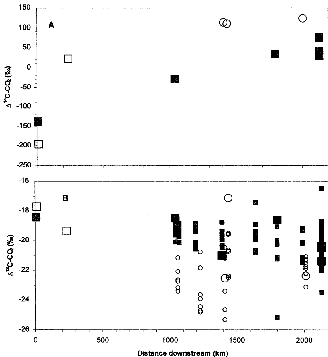
Figure 6.17. Downstream \text{CO}_2 isotopic evolution along the Amazon mainstem from the Ucayali-Marañón confluence to Manacapuru. Symbology is the same as in Fig. 6.1, but dark gray represents the Solimões-Amazonas mainstem and white the immediate tributaries to that system. A) \Delta^{14}\text{C} . B) \delta^{13}\text{C} .
