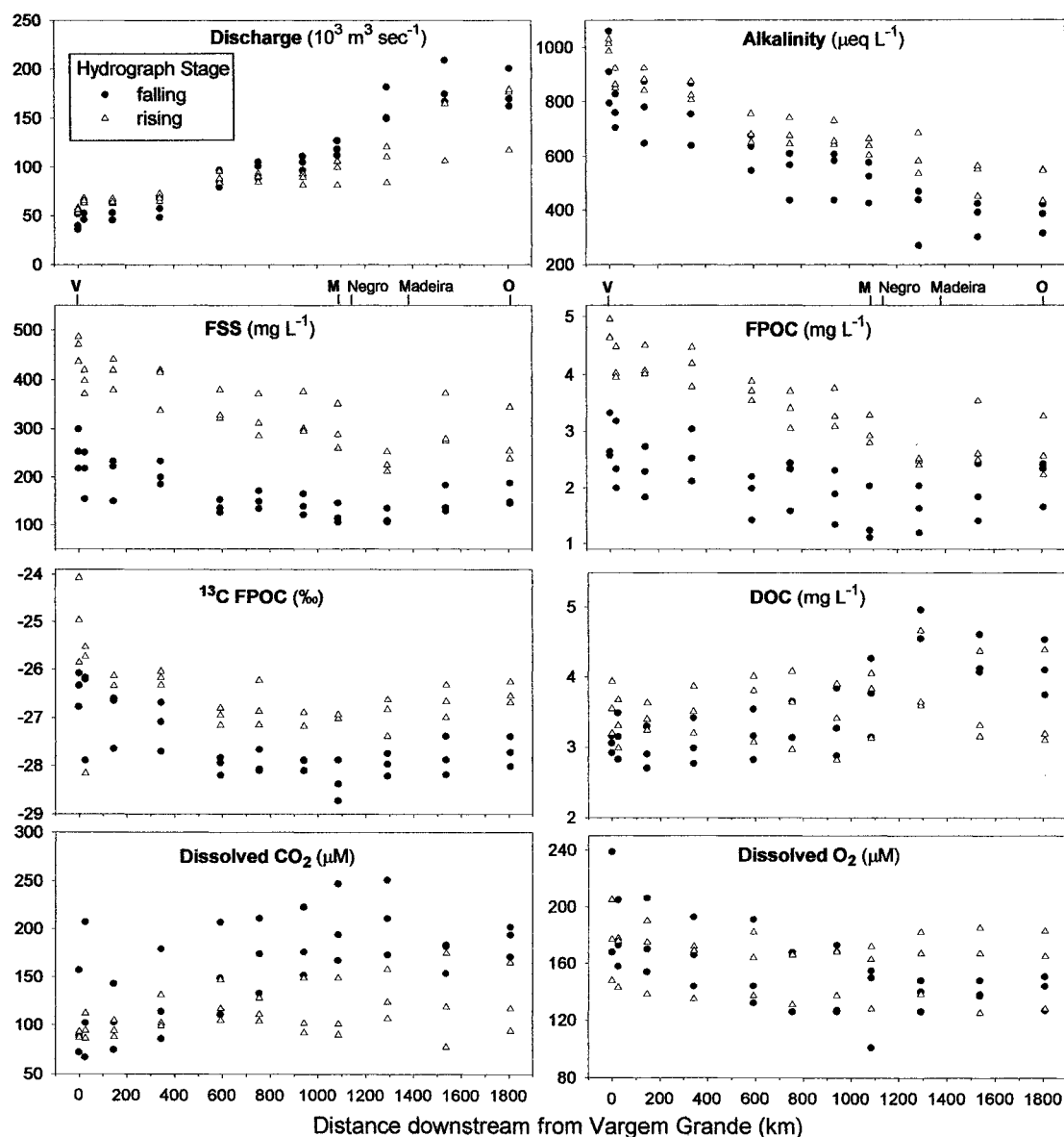
Figure 2.7. Longitudinal trends along an 1800 km reach in the Solimões-Amazonas mainstem from Vargem Grande to Óbidos in Brazil. The data have been divided into falling (closed circles) and rising (open triangles) stages according to major hydrograph periods, to highlight seasonal differences. Variables shown are river discharge, alkalinity, fine suspended sediment (FSS), fine particulate organic carbon (FPOC), carbon-13 content of FPOC, dissolved organic carbon (DOC), dissolved \text{CO}_2 gas, and dissolved oxygen. The sampling station labels at the top of the graph are the same as in Fig. 2.2. Data from Richey et al. (1990) and Quay et al. (1992).
