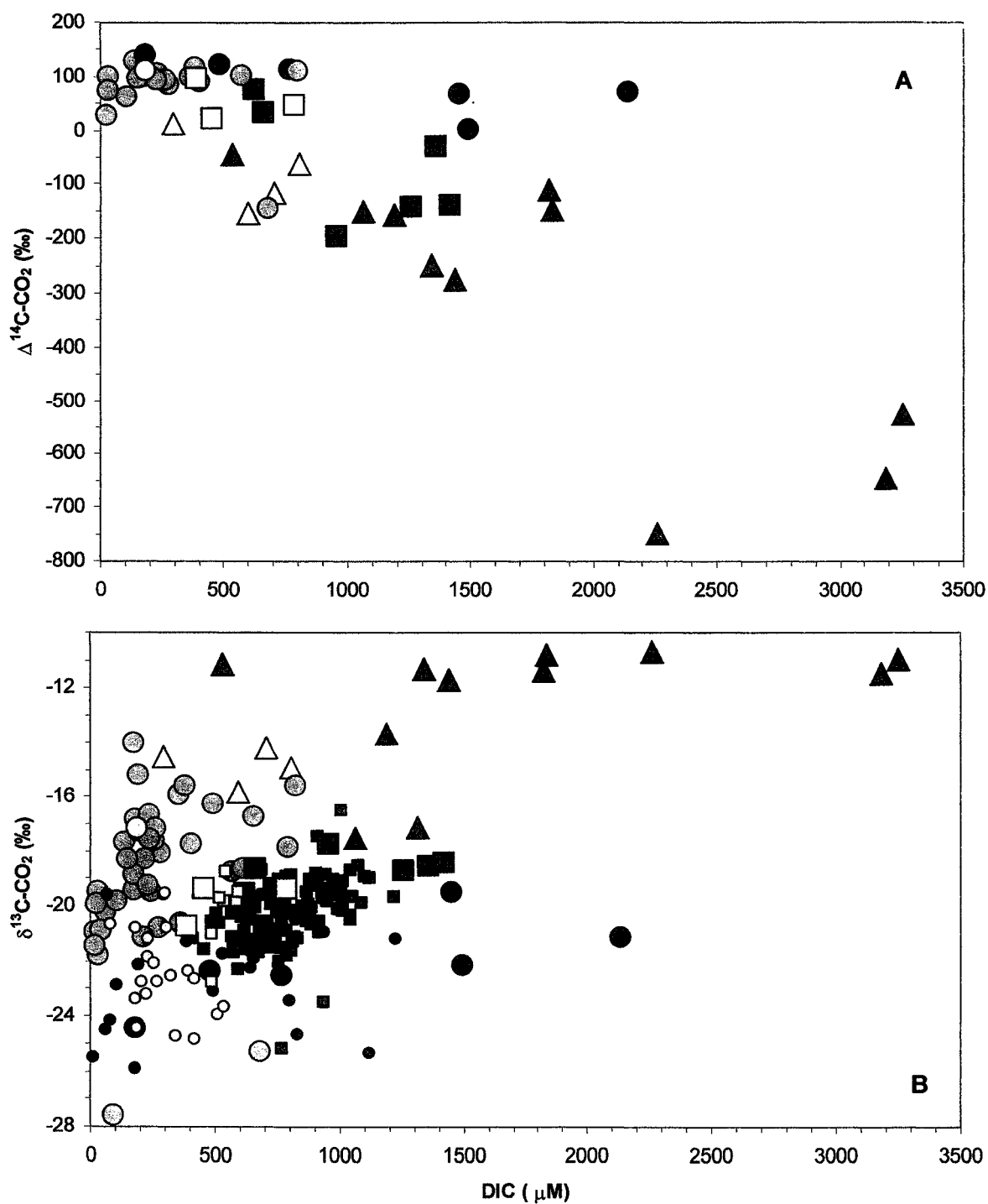
Figure 6.5. CO 2 isotopic variability with respect to DIC concentration. A) \Delta^{14}\text{C} . B) \delta^{13}\text{C} . Symbology is the same as in Fig. 6.1.
