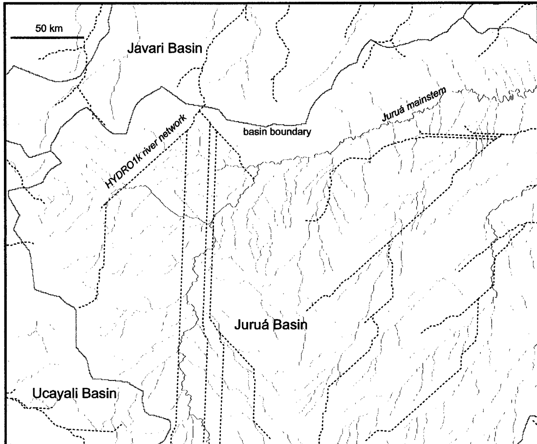
Figure 3.7. Comparison of CAMREX river network (solid lines) and HYDRO1k network (dotted lines) in the Juruá headwaters, in the lowlands of the central Amazon basin. The basin boundaries shown are the subbasin boundaries shown in Fig. 3.6 and created from the CAMREX drainage direction map. In this region, HYDRO1k drains the entire Juruá headwater system as parallel straight channels into the Javari basin to the North.
