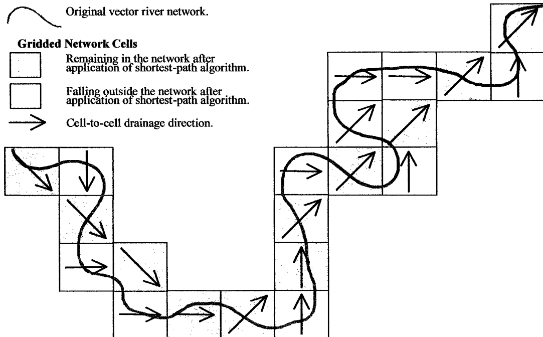
Figure 3.3. Gridding of a vector river network reach and application of a shortest cell-to-cell path distance scheme to extract in-channel drainage paths on the gridded network. This example illustrates meander smoothing and overall shortening of network path lengths when applying the shortest-distance scheme.
