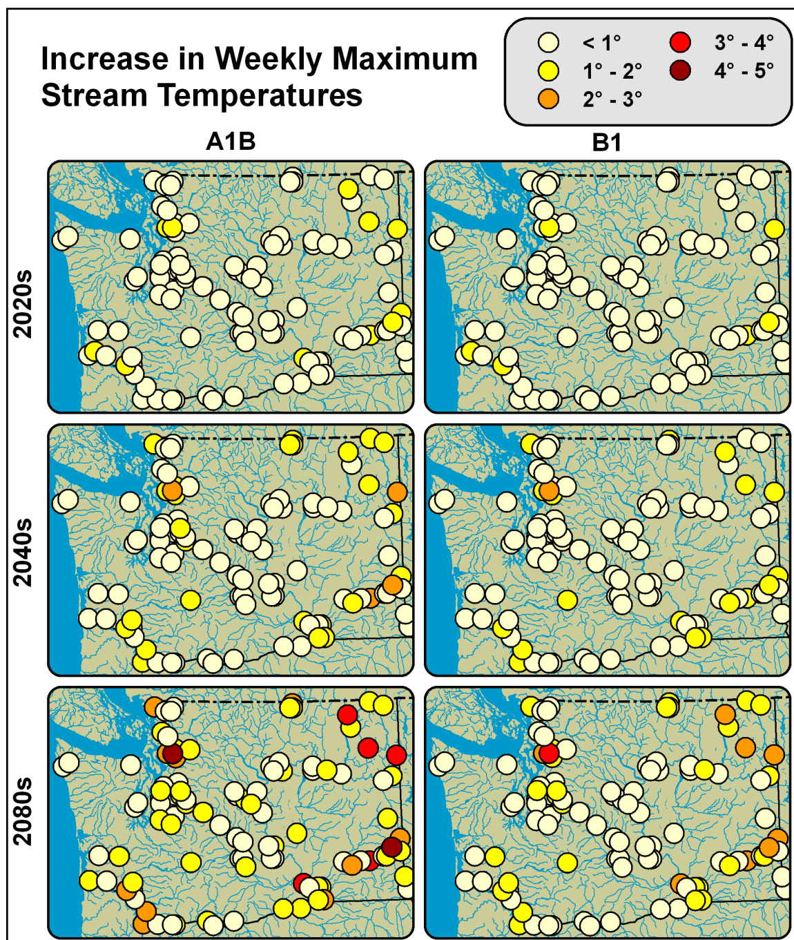
Figure 3. Simulated increases in the annual maximum of weekly water temperatures ( ^{\circ}\text{C} ) relative to the 1980s for select locations in Washington State. Top panels show simulated changes for the 2020s, middle panels for the 2040s, and bottom panels for the 2080s. Composite A1B emissions scenarios are in the left column, composite B1 emissions scenarios are in the right column.
