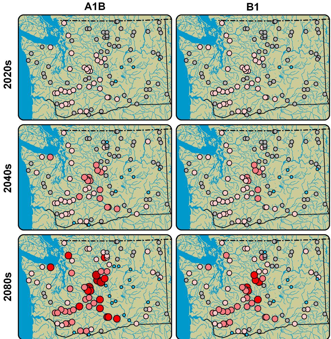
Figure 9. Ratio of the 20 year flood magnitudes for simulated future and historic streamflows at select locations. Top panels show simulated changes for the 2020s, middle panels for the 2040s, and bottom panels for the 2080s. Composite A1B emissions scenarios are in the left column, composite B1 emissions scenarios are in the right column.
