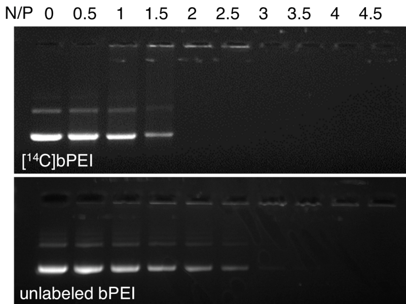
Figure 2.5: Gel retardation assay of unlabeled and [^{14}\text{C}] -labeled bPEI. [^{14}\text{C}] -labeled and unlabeled bPEI were complexed with unlabeled plasmid DNA at different charge ratios (N/P) and loaded onto 0.8% agarose gels. Plasmid DNA was visualized using ethidium bromide.
