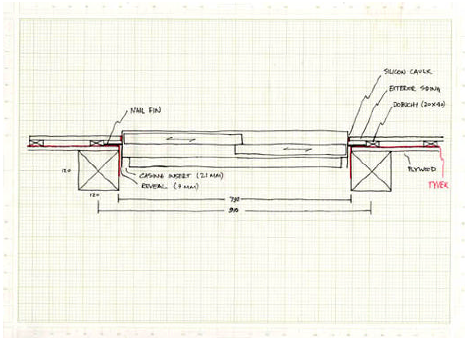
Figure 46. Technical drawing of a double slider window installed between posts with a dobuchi rain screen siding exterior. Note the space between the exterior siding and the window frame that is filled with a silicon caulk.
