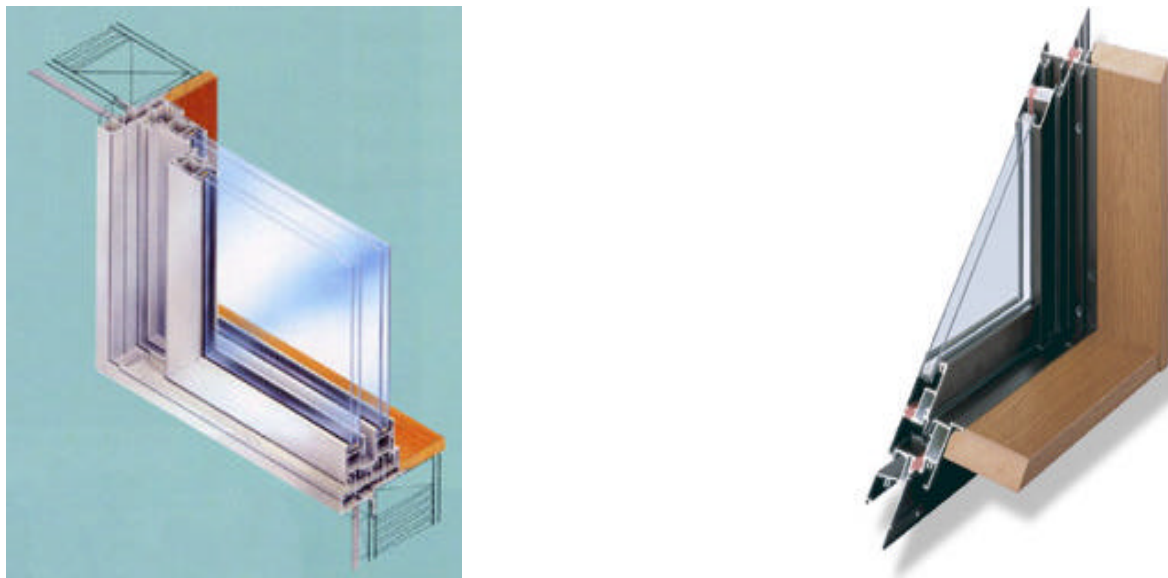
Figure 13. Corner details of YKK aluminum clad wood windows. Source: YKK website
