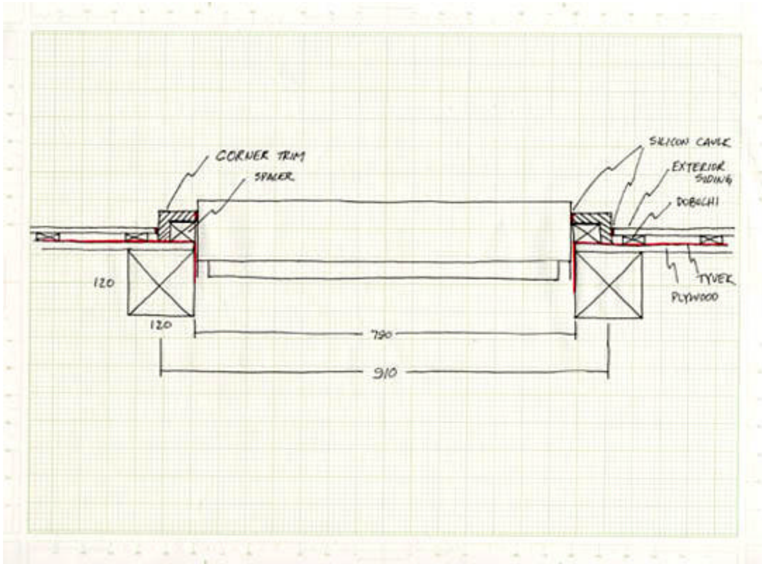
Figure 47. Technical drawing of double hung window with the dobuchi siding system. Note that the window is pulled away from the exterior wall with a spacer and the exterior siding butts up against the corner trim, not the window frame.
