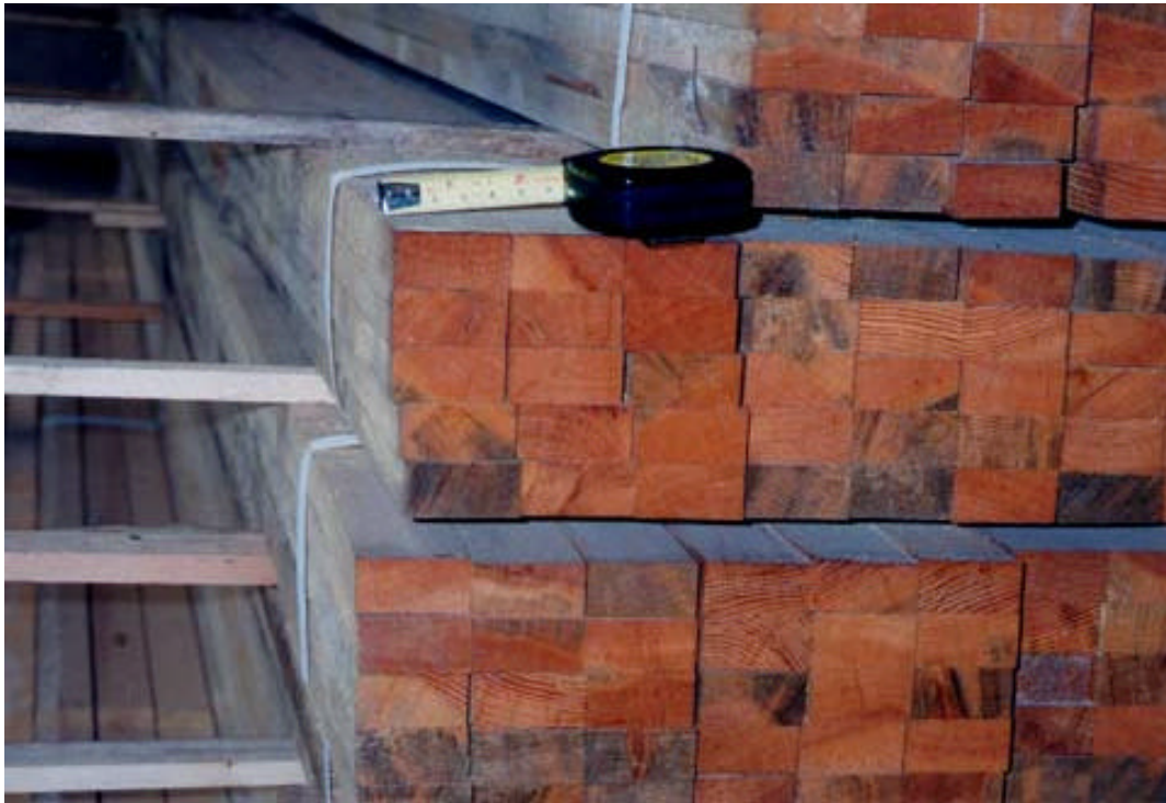
Figure 43. Wood dobuchi strips (20mm by 40 mm) are used in the rain screen siding system.
