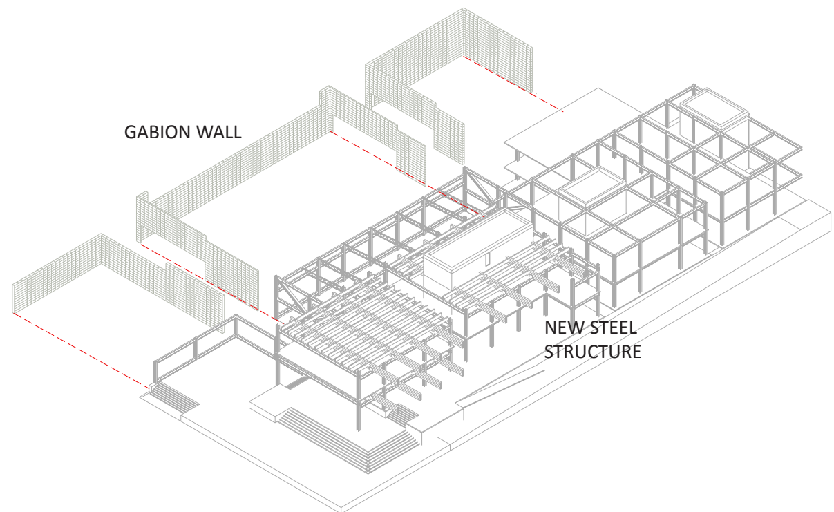
Fig. 4.7 Crushed concrete gabion walls attach to new steel frame structure on the west side of the building
