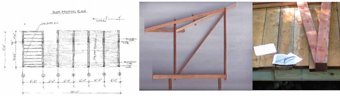
Figure. 9 Floor plan, Truss Model and Construction Photo of Bunk House.
