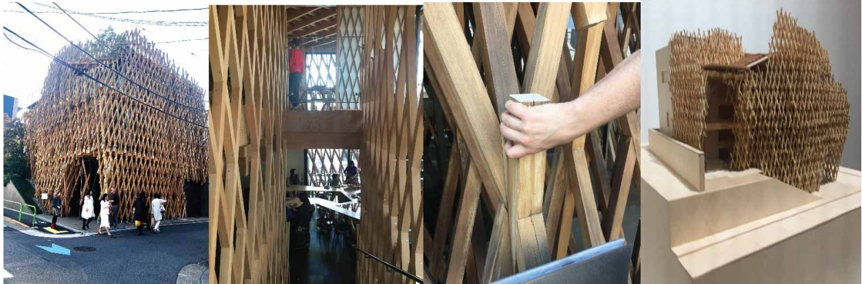
Figure 8. Sunny Hills in Site, Structure, Size of beam in Relation to Hand and Scale Model.
