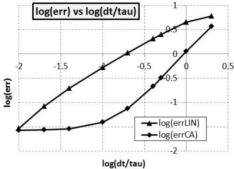
Figure 4.3 Error in predicted strain at 100 days vs. time step.
