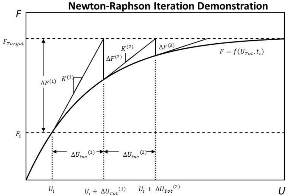
Figure 3.4 Graphical illustration of Newton-Raphson iteration scheme.
