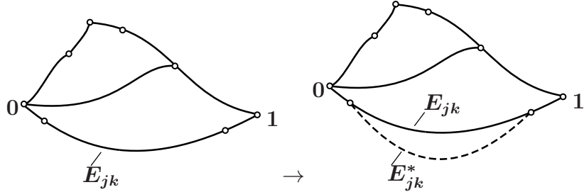
Figure 2.6: Case (2) in the construction.
