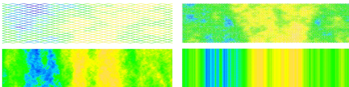
Figure 4.8: Scaled simulation of the process when the ratio is 1/n : 1/n , for n = 32, 128, 512, \infty .
