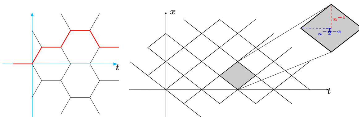
Figure 4.6: Index set: Honeycomb graph and \alpha -rhombus grid
