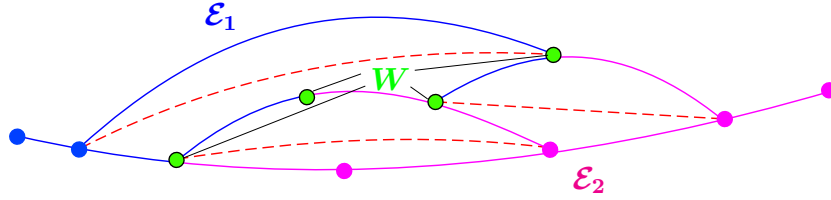
Figure 3.6: (X(t) : t \in \mathcal{E}_1) is independent of (X(t) : t \in \mathcal{E}_2) given X_W .
