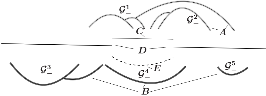
Figure 2.11: A , B , C , D and E parts of \mathcal{G} .
