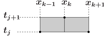
Figure 6.2: Rectangle R_{jk}
