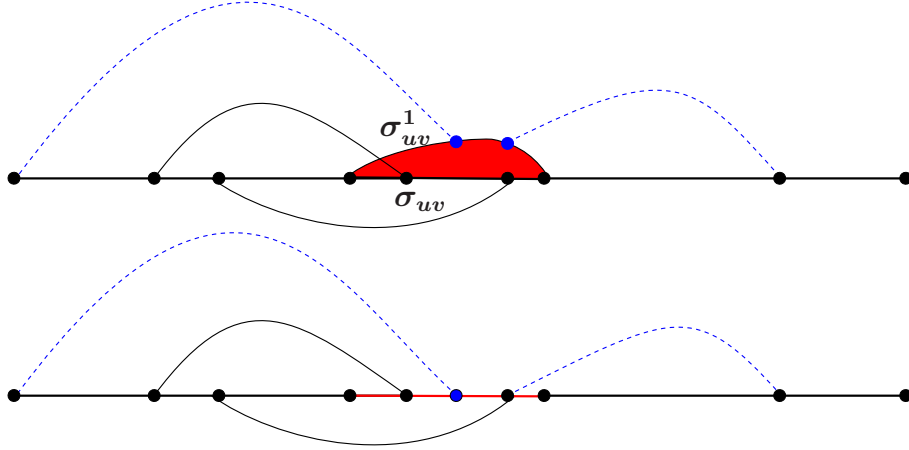
Figure 1.19: Transformation from \mathcal{G} to \mathcal{G}^\circ .
