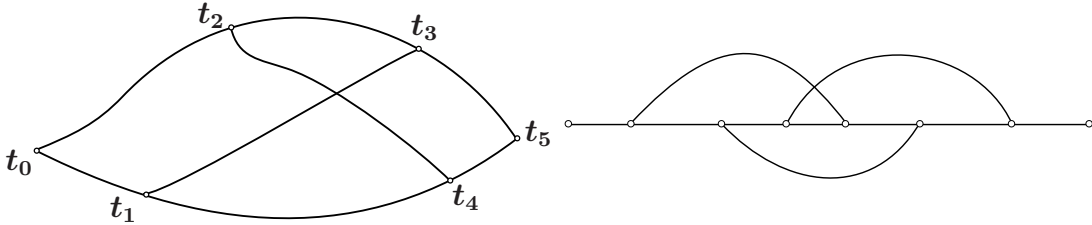
Figure 1.12: Non-planar \text{TLG}^* .
