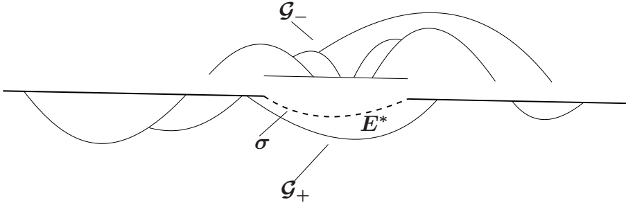
Figure 2.10: \mathcal{G}_- and \mathcal{G}_+ with respect to \sigma .
