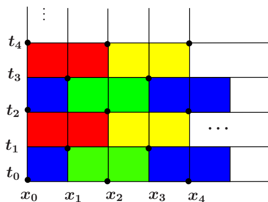
Figure 6.1: Euler method
