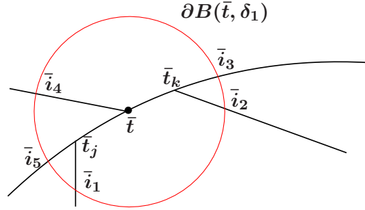
Figure 1.17: The representation intersected by a sphere. In this case we have I = \{i_1, \dots, i_5\} .
