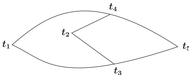
Figure 8.9: A planar TLG that is not a TLG^{**} .
