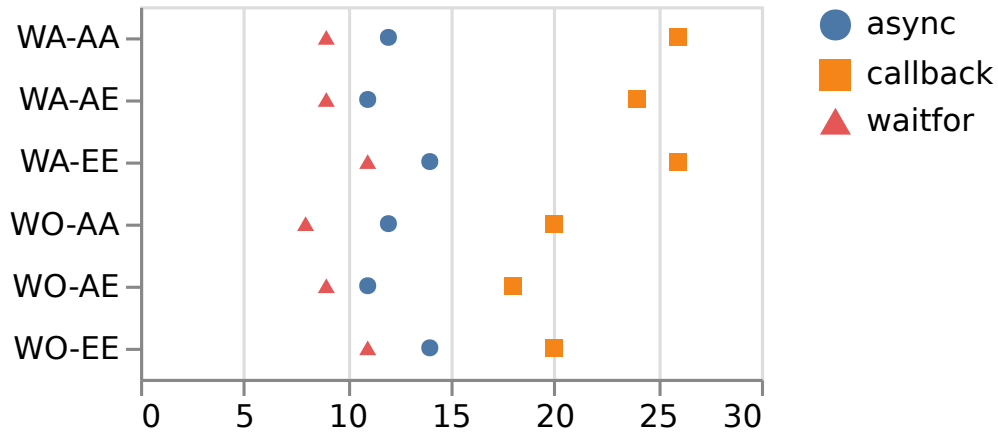
Figure 6.3: Systematic evaluation results: concurrency patterns vs. number of blocks.
