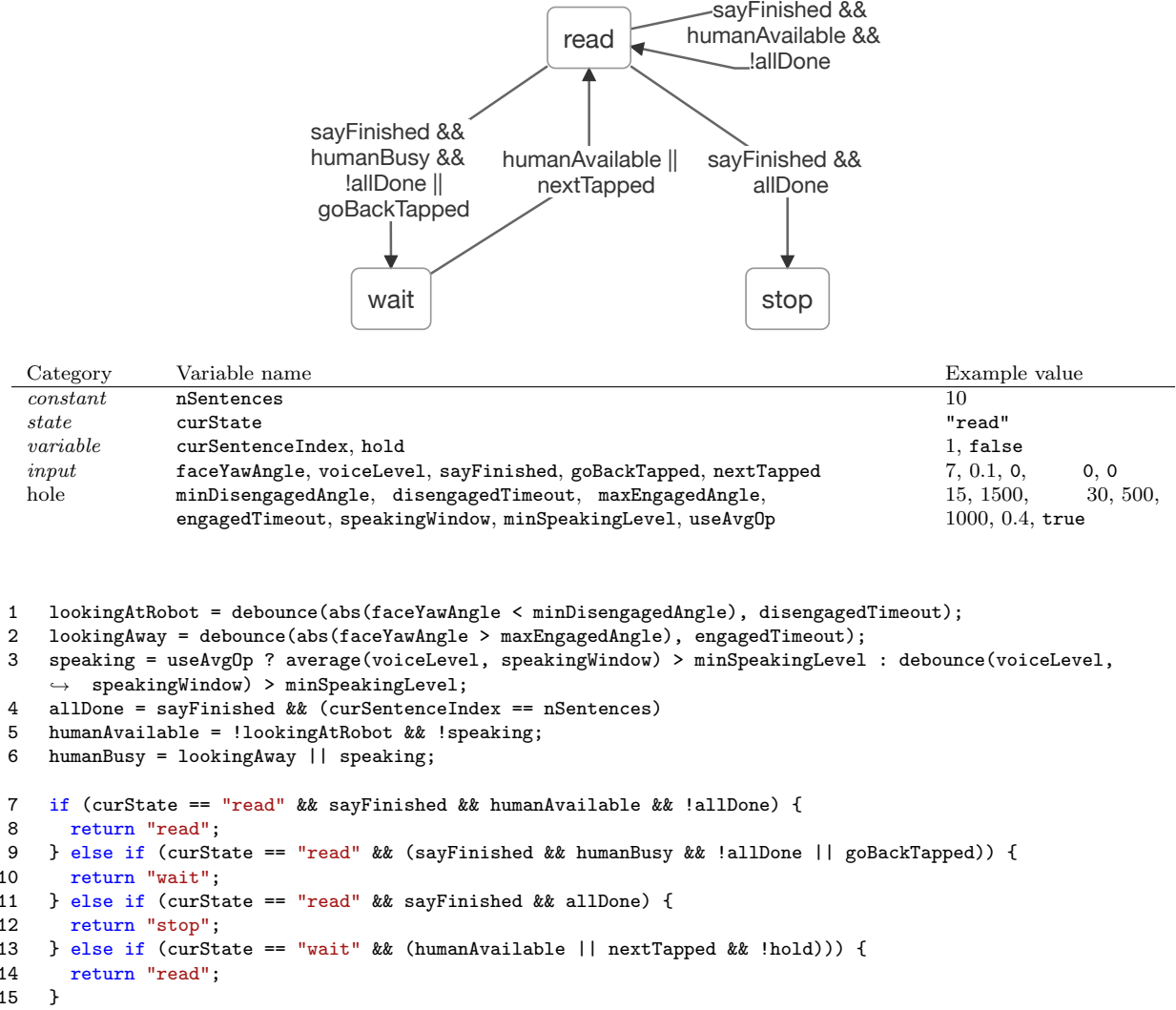
Figure 7.3: An example program in SoRTSketch. (top) the social robot used this paper and an FSM visualization for the storytelling program; (middle) Instantiation of SoRTSketch in a storytelling social robot domain with defined constants, inputs, variables, and holes; (bottom) transition function program with variable definitions and if-else statements.
