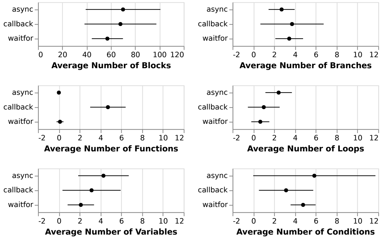
Figure 6.5: User study results: interfaces vs. measures.
