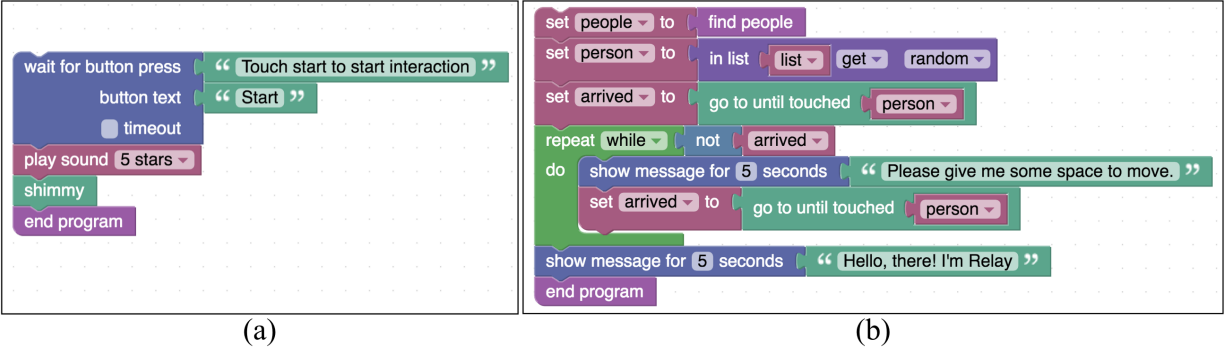
Figure 5.1: Example applications written in iCustomPrograms . (a) Simple interactive application; the robot first waits for a user to engage in interaction by pressing a button. It then plays a sound and shimmies in response. (b) Approaching a person application; the robot finds nearby people using findPeople , randomly selects a person, and approaches them. The goToUntil primitive returns true if the robot successfully reaches the destination and false if it is interrupted by a person tapping its touchscreen.
