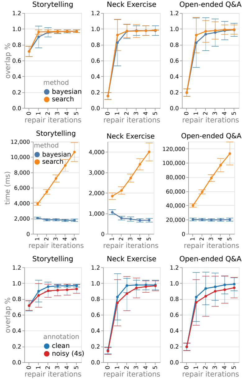
Figure 7.5: Results from the simulation experiment. (top) Percentage overlap over five repair iterations using IterativeRepair (labeled as search) and IterativeBayesRepair (labeled as bayesian) algorithms across three tasks (storytelling, neck exercise, Q&A). (middle) Computation time of the algorithms for the same settings. (bottom) Overlap percentage over five repair iterations for the IterativeBayesRepair algorithm using clean and noisy state corrections for repair. Error bars show standard deviations.
