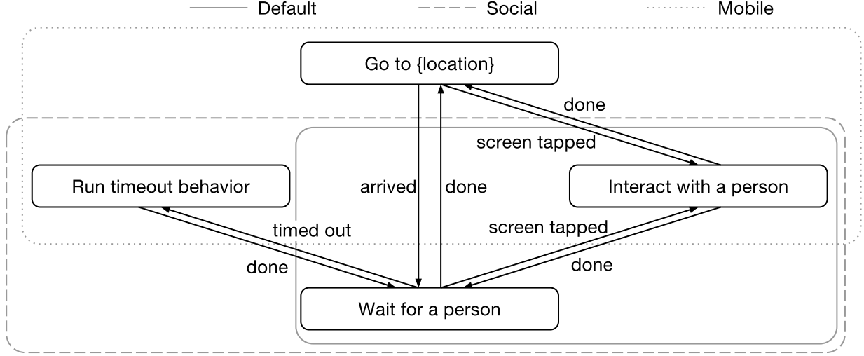
Figure 4.4: Finite state machines that implement the three robot behaviors: Baseline, Social, and Mobile.
