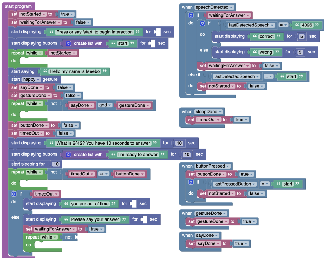
Figure 6.7: User-created programs using “callback” ConCodeIt!
