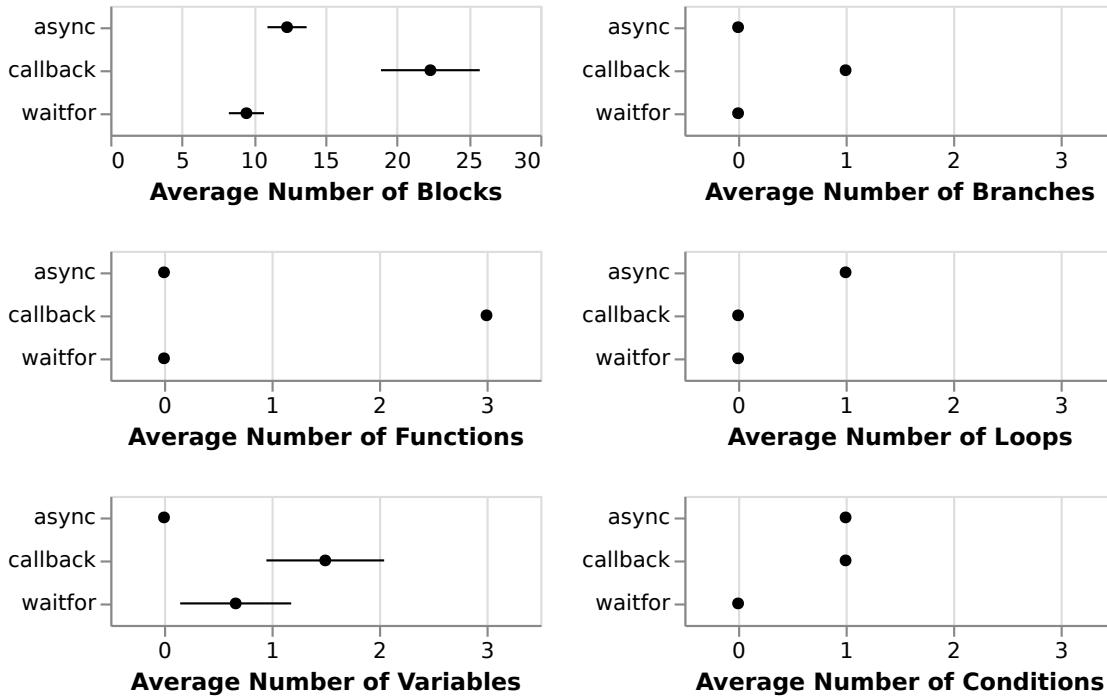
Figure 6.2: Systematic evaluation results: interfaces vs. measures.
