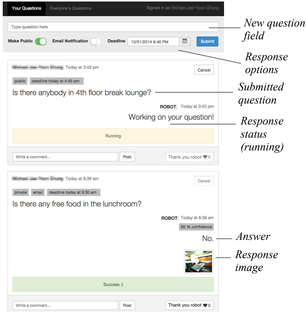
Figure 3.4: InfoBot front-end web interface.
