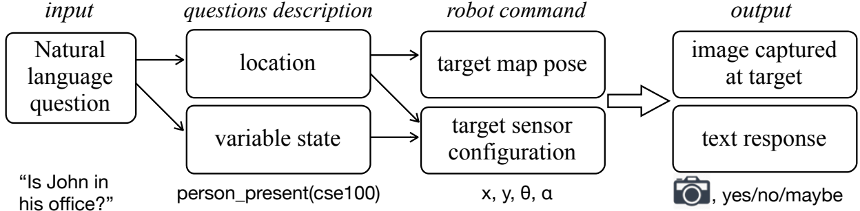
Figure 3.1: Steps for information checking. The solid arrows represent the input processing steps and the hollow arrow represent the step involving physical robot actions (e.g. navigation) that produces the outputs.
