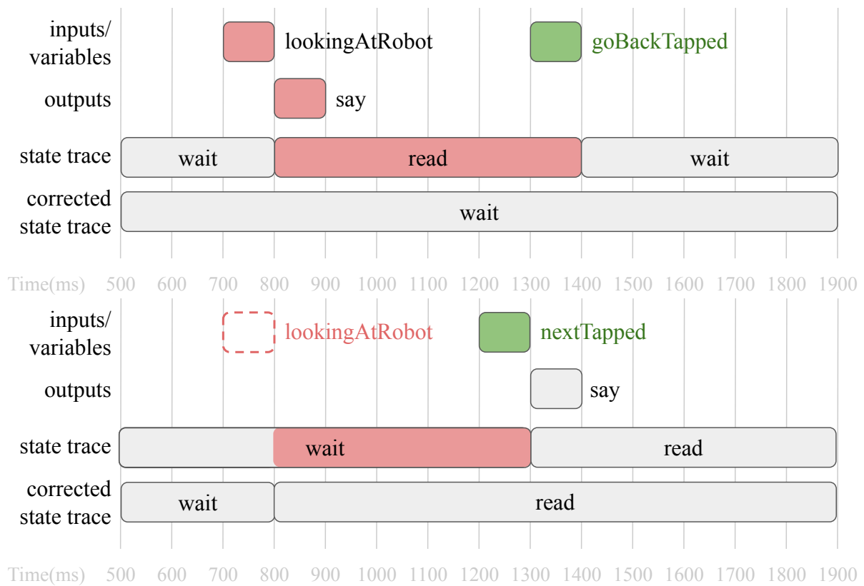
Figure 7.4: Incorrect (above) and missing (below) transition errors and recovery examples from the storytelling robot example. Incorrect states and associated variables are highlighted in red. Implicit feedback in the user input is highlighted in green. The dotted red square represents an undetected human action.
