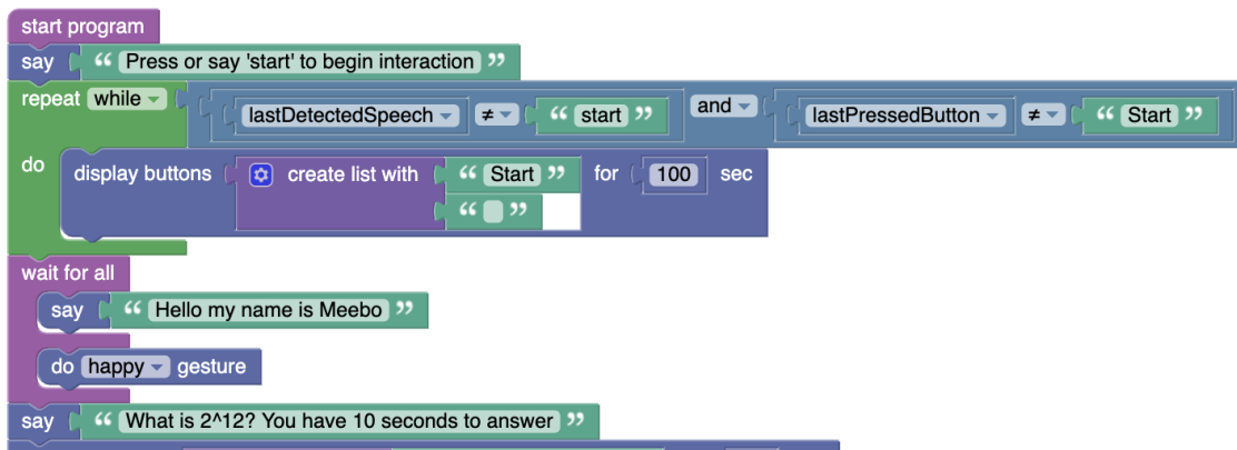
Figure 6.8: A user-created program using “waitfor” ConCodeIt!
