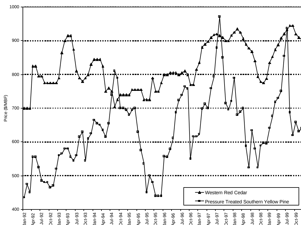
Figure 1. National Average Monthly Price per Thousand Board Foot of 5/4" × 6" Western Red Cedar and Southern Yellow Pine Treated Lumber Radius Edged Deck Materials, January 1992 through October 1999.
