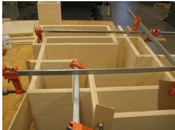
Fig. 9.6 Shelf assembly glue up.
