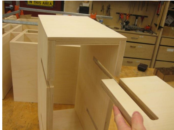
Fig. 9.5 Interlocking slot detail and assembly
