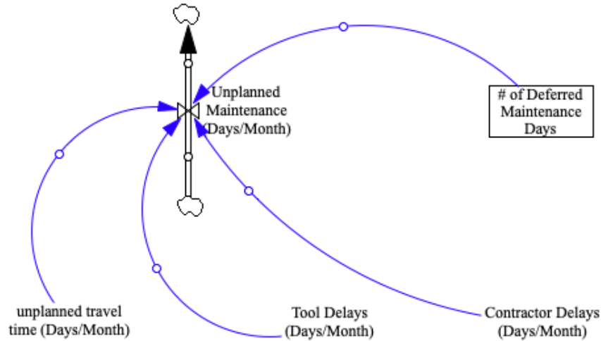
Figure 6: The auxiliary variables that feed the rate of unplanned maintenance days per month are unplanned travel time, tool delays and contractor delays. The stock of deferred maintenance days also feeds this rate, and acts as a time delay between maintenance that is not completed, and systems failures that result from skipped maintenance.
