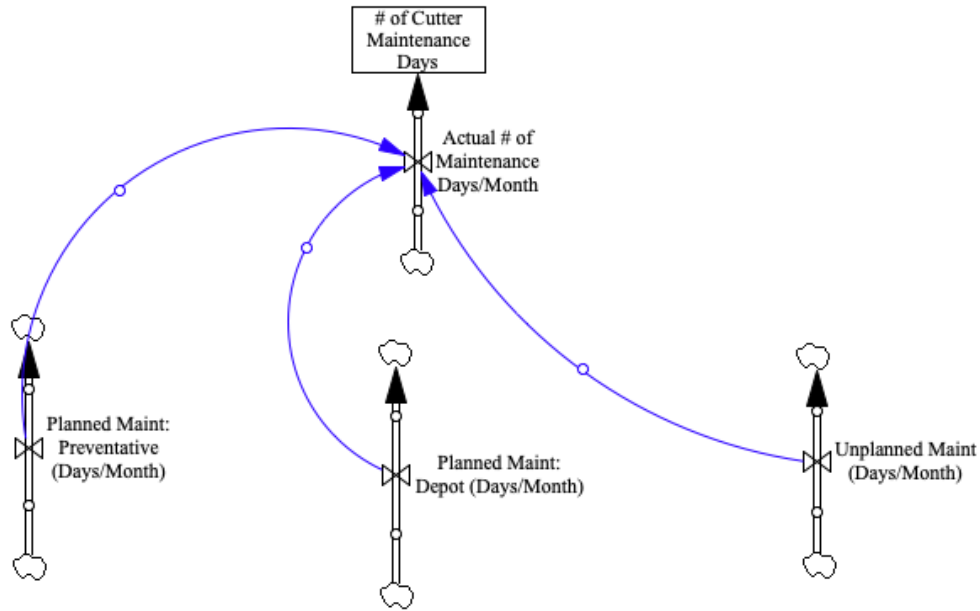
Figure 5: Rates impacting the stock of actual maintenance days for a cutter over a two-year period.
