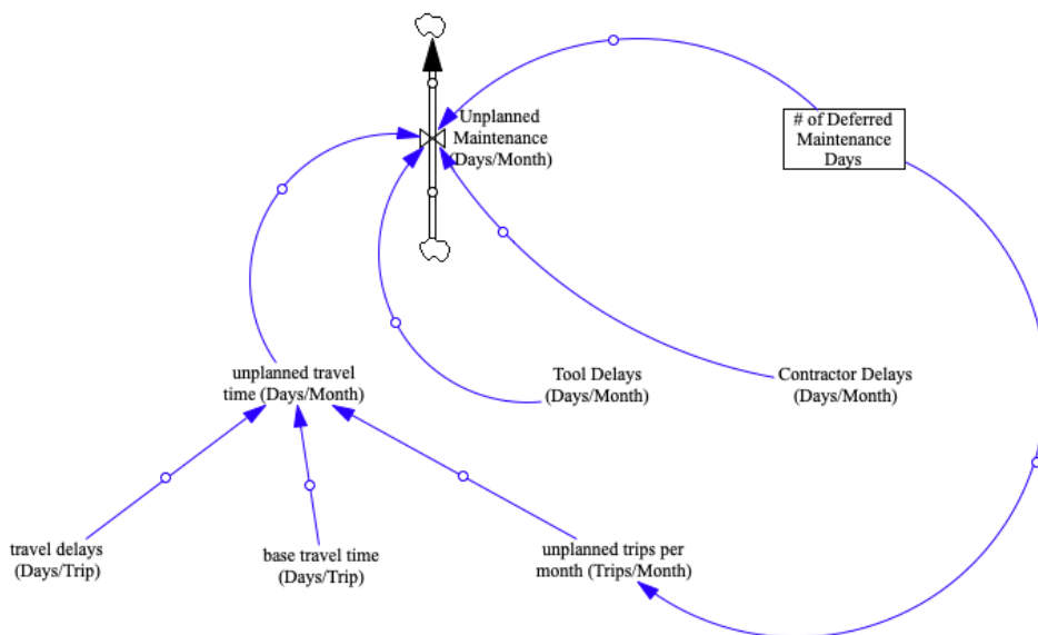
Figure 7: An expanded view of Figure 6, including the auxiliary variables that feed “unplanned travel time”. Note that the stock of deferred maintenance days again acts as a time delay, eventually increasing the number of unplanned maintenance trips needed every month.
