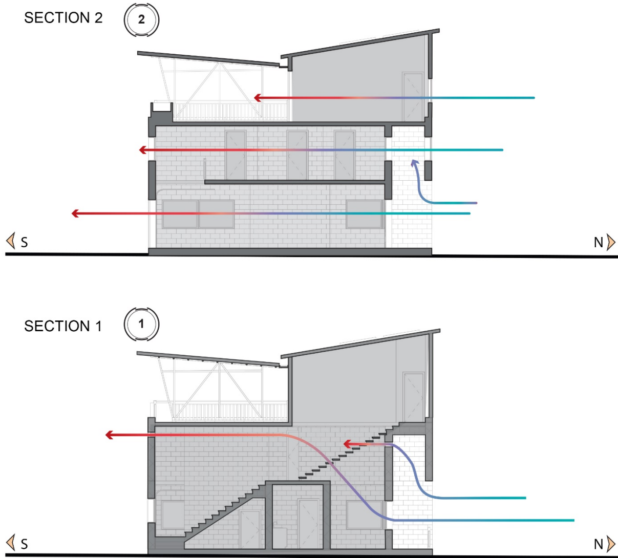
Fig. 5.9: Sections - Ventilation
