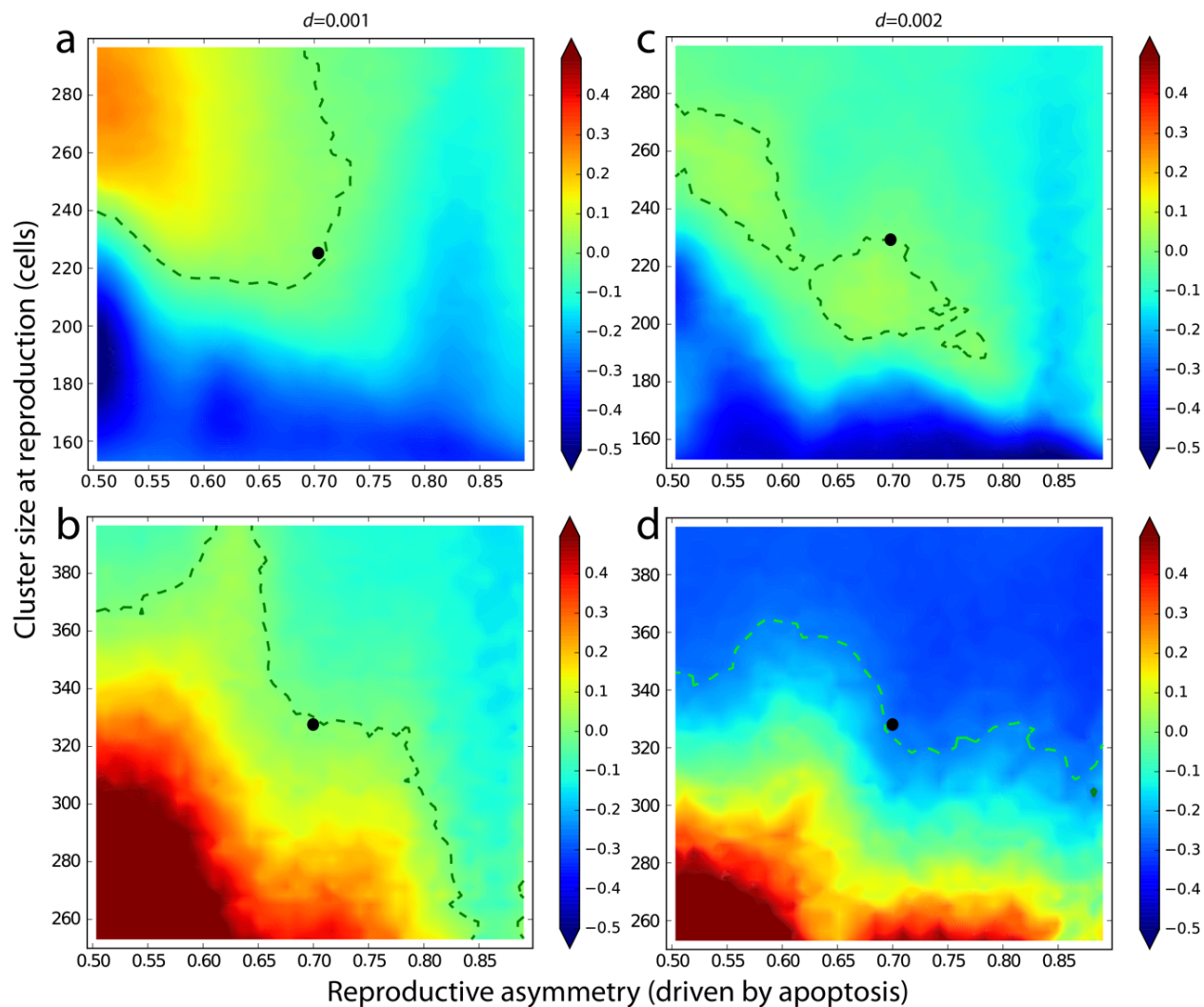
Figure 5.2: Fitness landscapes vary depending on the extent of resource diffusion and on cluster size. In each fitness landscape plotted above, a single strain (filled circle) competes against 1,554 competitor strains varying in cluster size at reproduction and apoptosis. Large size and low apoptosis are favored in small clusters with little diffusion limitation (A), while increasing the growth cost of diffusion favors smaller clusters with higher rates of apoptosis (C). Increasing cluster size at reproduction by 100 favors smaller cluster size (B, D). Apoptosis provides more of a benefit to larger clusters (lower region of B, D). Here s = 140 , d = 0.001 , and the growth phase contains sufficient resources for the production of 8 \times 10^6 cells. The dashed line demarcates a relative fitness of 0.
