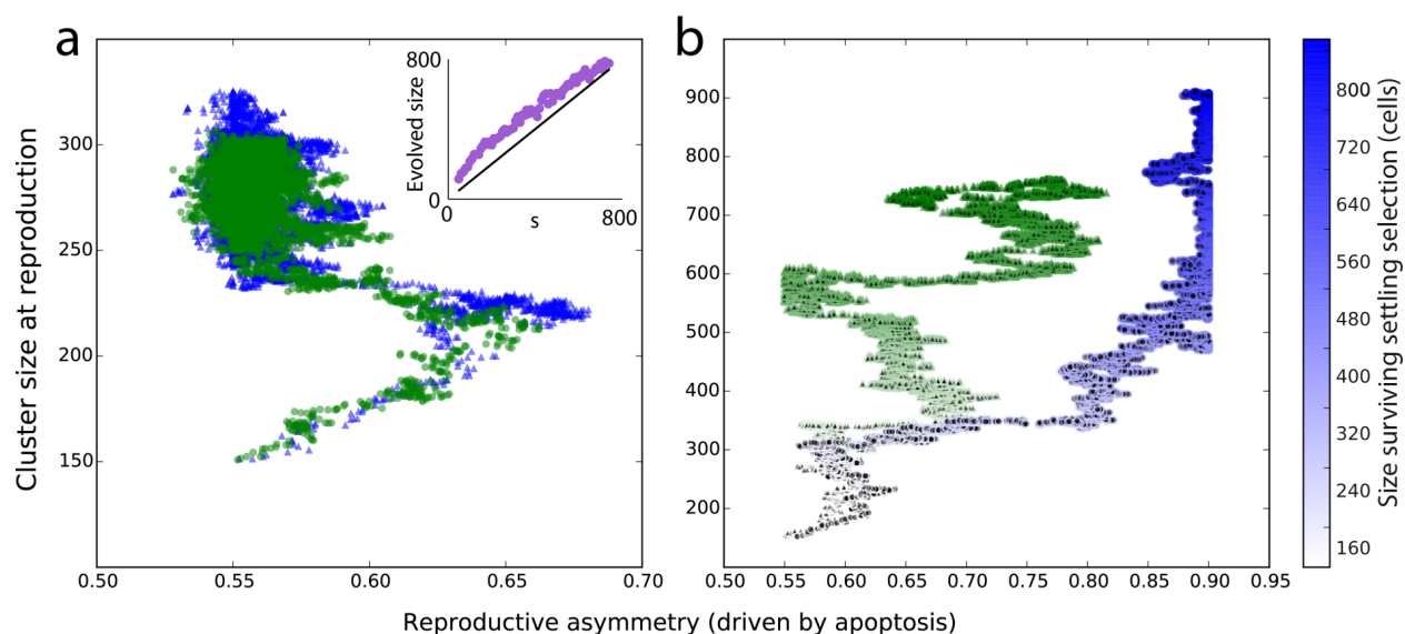
Figure 5.5: Pushing the envelope—the evolution of large clusters. (a) When the environment is constant ( s = 140 for all 7,600 transfers), equilibrium dynamics rapidly establish themselves with the evolution of modest cluster size and low apoptosis. For a range of s from 50–750, cluster size at equilibrium (1,000 transfers, purple circles in 5a inset) is only modestly larger than required for surviving settling selection (black line, inset). (b) Slowly ratcheting up the threshold for settling to the bottom of the tube ( s starts at 140 and increases by 1 every 10 transfers) results in the evolution of very large clusters with high rates of apoptosis. Filled circles and triangles refer to the two strains in competition. In these simulations the growth phase contains sufficient resources for the production of 2 \times 10^6 cells and d = 0.001 .
