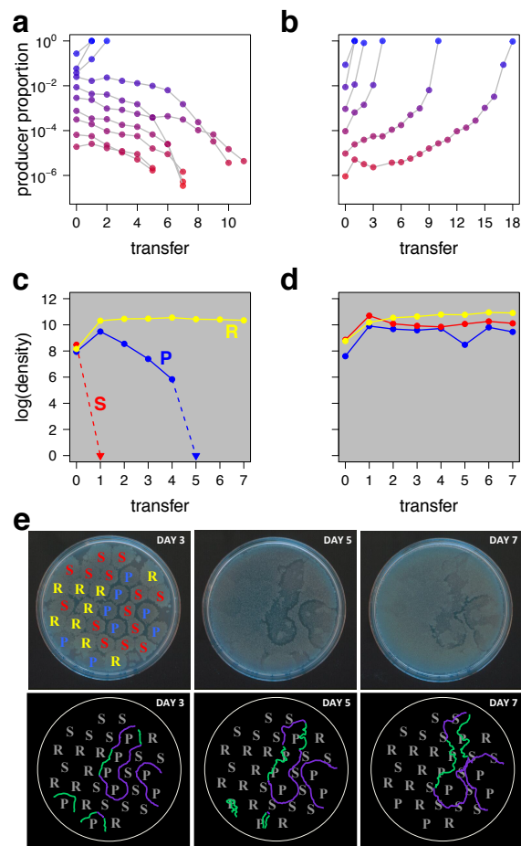
Figure 6.4: Spatial games. (a) An experiment tracking the proportion of colicin E3 producers in liquid culture. If the producers start above a critical fraction ( 0.02), then the producers drive the sensitive non-producers extinct. Otherwise, the producers go extinct (data reproduced with permission from Chao & Levin (1981)). (b) When the same community is propagated in a structured environment (soft agar), the producers increase despite initial proportion. (c) A second experiment tracking the density of three genotypes. In a well-mixed flask, the sensitive non-producer ( S ) quickly goes extinct (due to the ubiquitous toxin) and then the producer ( P ) is outcompeted by the resistant non-producer ( R ) (data reproduced with permission from Kerr et al. (2002)). (d) All three genotypes are maintained at high density when the community is propagated on the surface of an agar plate. (e) Time series photographs of a representative replicate of the RPS community propagated on agar. (Top row) The changing spatial configuration of the experimental community is shown in this first panel of photographs. Because borders could be identified where P interacted with R or S , the direction of clump movement over transfers could be inferred. (Bottom row) ‘Chasing’ between clumps is highlighted in this second panel. The borders where P chased S are colored in purple and the borders where R chased P are in green.
