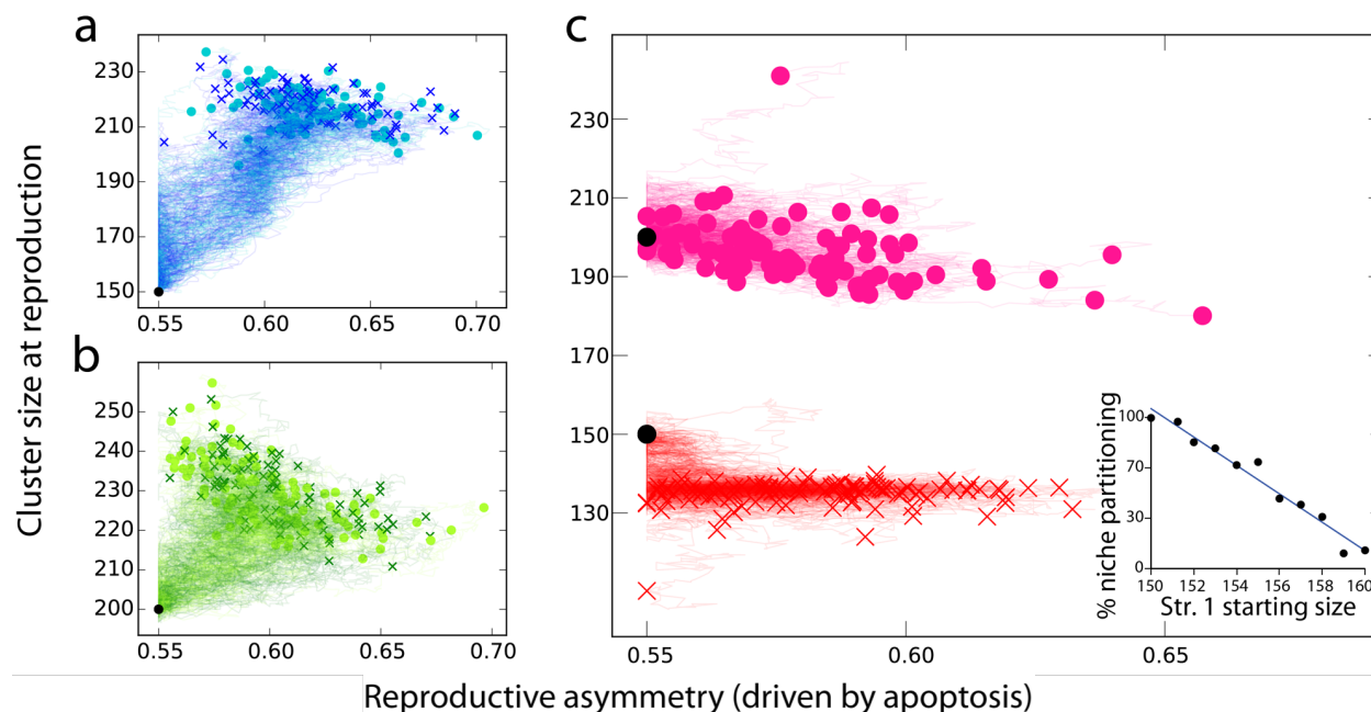
Figure 5.4: Arms races and niche partitioning. Larger clusters with higher rates of apoptosis evolve when both starting strains are similarly sized (a, b). If the initial size difference is substantial, arms-race dynamics are prevented, and instead the smaller strain evolves smaller size, becoming a growth specialist (c). The frequency of niche partitioning declines linearly as strain (Str.) 1's starting size increases from 150 to 160 (c, insert). Plotted are 100 simulations for each strain (strains 1 and 2 are demarcated by dark X's and light circles, respectively) over 150 transfers. Here s = 140 , d = 0.0015 , and the growth phase contains sufficient resources for the production of 2 \times 10^6 cells.
