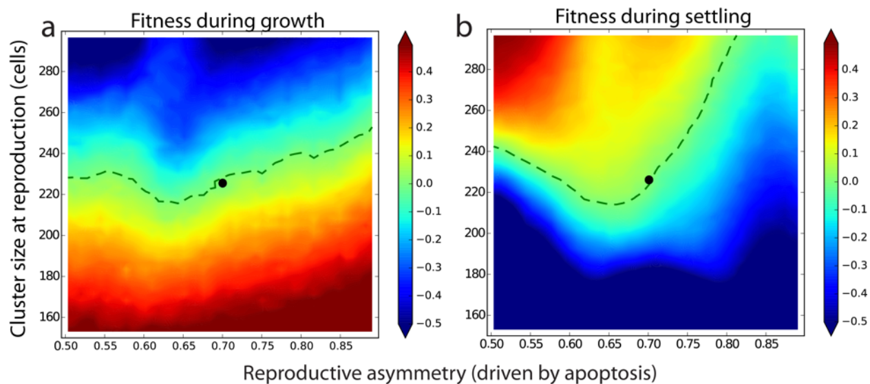
Figure 5.3: Disentangling fitness contributions from growth (a) and settling (b). We calculated the relative fitness consequences (as selection rate constants) during growth and settling for the landscape shown in figure 2c. Smaller cluster size at maturity and apoptosis increases fitness during growth at a cost to settling. Here s = 140 , d = 0.002 , and the growth phase contains sufficient resources for the production of 8 \times 10^6 cells. The dashed line demarcates a selection rate constant of 0.
