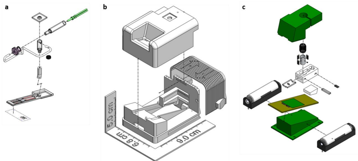
Figure 105: Exploded view of one of four identical MAD NAAT prototypes. (a) Fluid path components, including fluid storage and introduction syringe, sample chamber, and 2DPN. (b) Housing components: base, lid, and slider. (c) Supporting components, including electronics, valves, batteries, and insulation.
