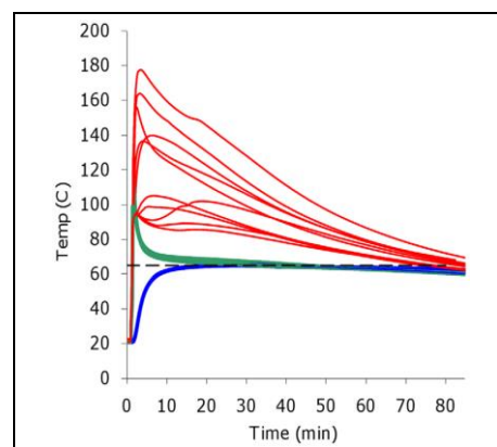
Figure 12. Temperature vs. time of multiple runs ( N=10 ) measured at the exothermic reaction (red), interface with the phase change material (green), and at the nucleic acid amplification reaction (blue) [66].
