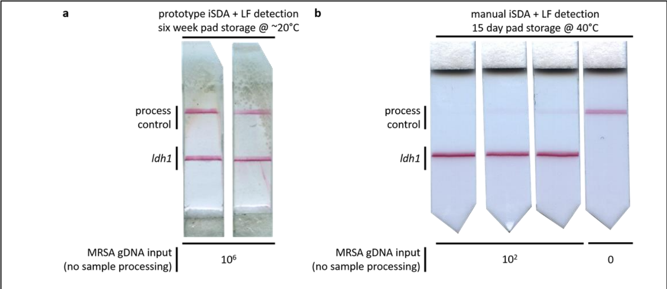
Figure 101: Detection results excerpted from dry storage study. (a) Prototype iSDA and LF detection on MRSA genomic DNA input using pads stored for six weeks at laboratory ambient temperature in desiccated conditions. Duplicate tests confirm dry reagent viability in these conditions through Idh1 amplification and detection functionality. (b) Manual assay tests on low input copy number MRSA genomic DNA using pads stored for 15 days at 40°C in desiccated conditions. Triplicate tests confirm dry reagent viability in these conditions through Idh1 amplification and detection functionality. Associated negative control indicates no contamination.
