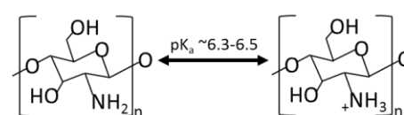
Figure 48. Chitosan structure in protonated and unprotonated forms.
