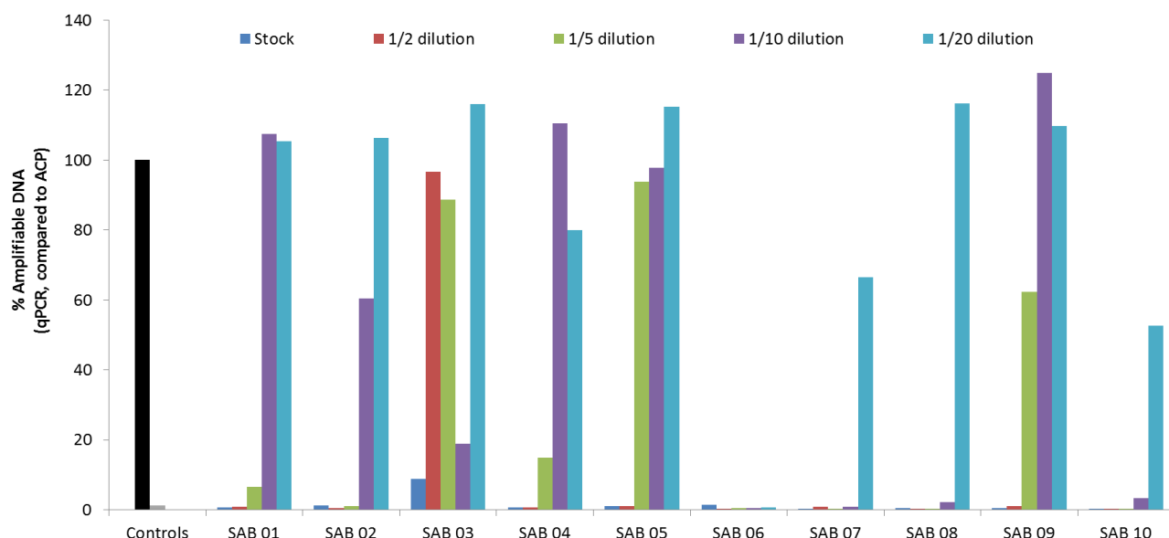
Figure 11. MSSA lysis with ACP in increasing dilutions of patient urine samples. Input \sim 10^5 bacteria/ \mu\text{L} , positive control was ACP treatment in 10 mM Tris (pH 8) followed by heat deactivation at 95^\circ\text{C} for 5 minutes, negative control was no lysis.
