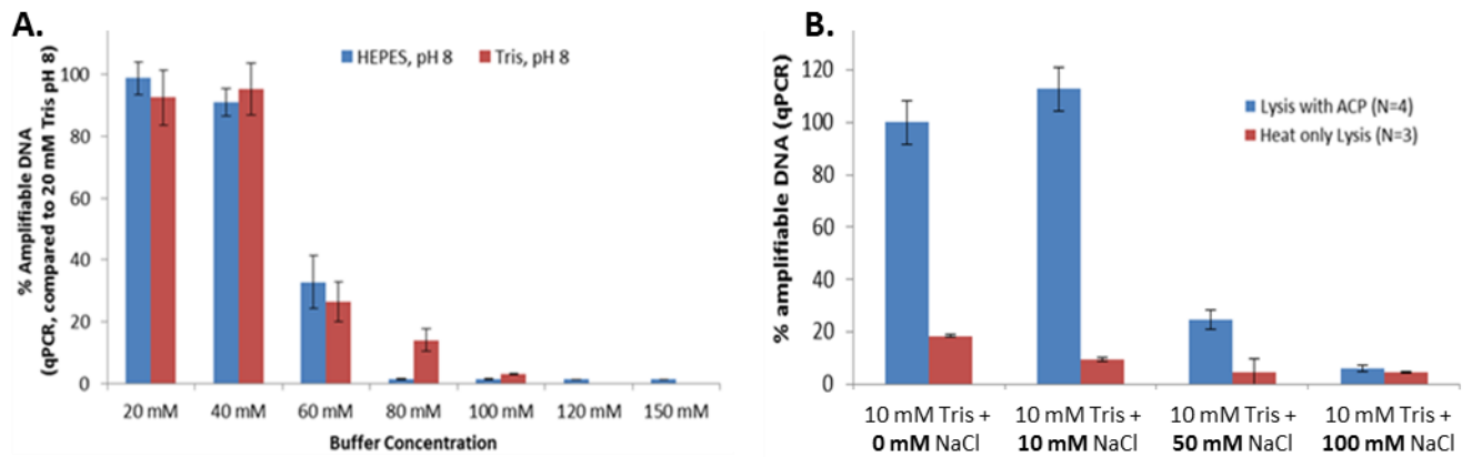
Figure 10. Effect of buffer composition and concentration on MSSA treatment with ACP. An average of at least N=3 +/- one standard deviation is reported for each condition. A. Increasing buffer concentration above 50 mM significantly impaired ACP function resulting in decreased availability of amplifiable DNA. B. Increasing NaCl concentration in the lysis buffer also significantly inhibited ACP function.
