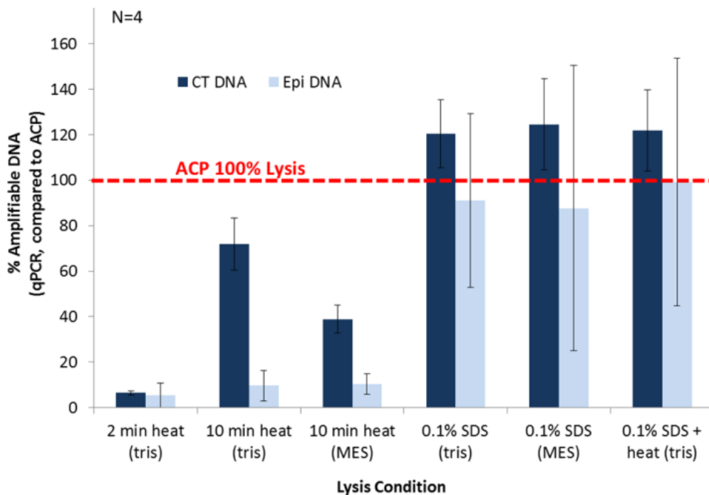
Figure 18. Comparing multiple lysis methods for CT+ cells. All samples were compared to lysis of CT+ epithelial cells in buffer with ACP for 2 minutes at room temperature followed by 10 minutes of heating to 95°C. Averages of at least N=4 are reported with error bars representing one standard deviation. Lysis of both the C. trachomatis and epithelial cells were quantified with separate qPCR assays. Lysis of the epithelial cells was highly variable.
