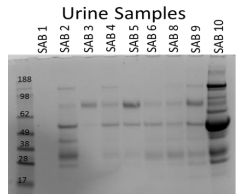
Figure 24. Protein gel of concentrated human urine samples.
