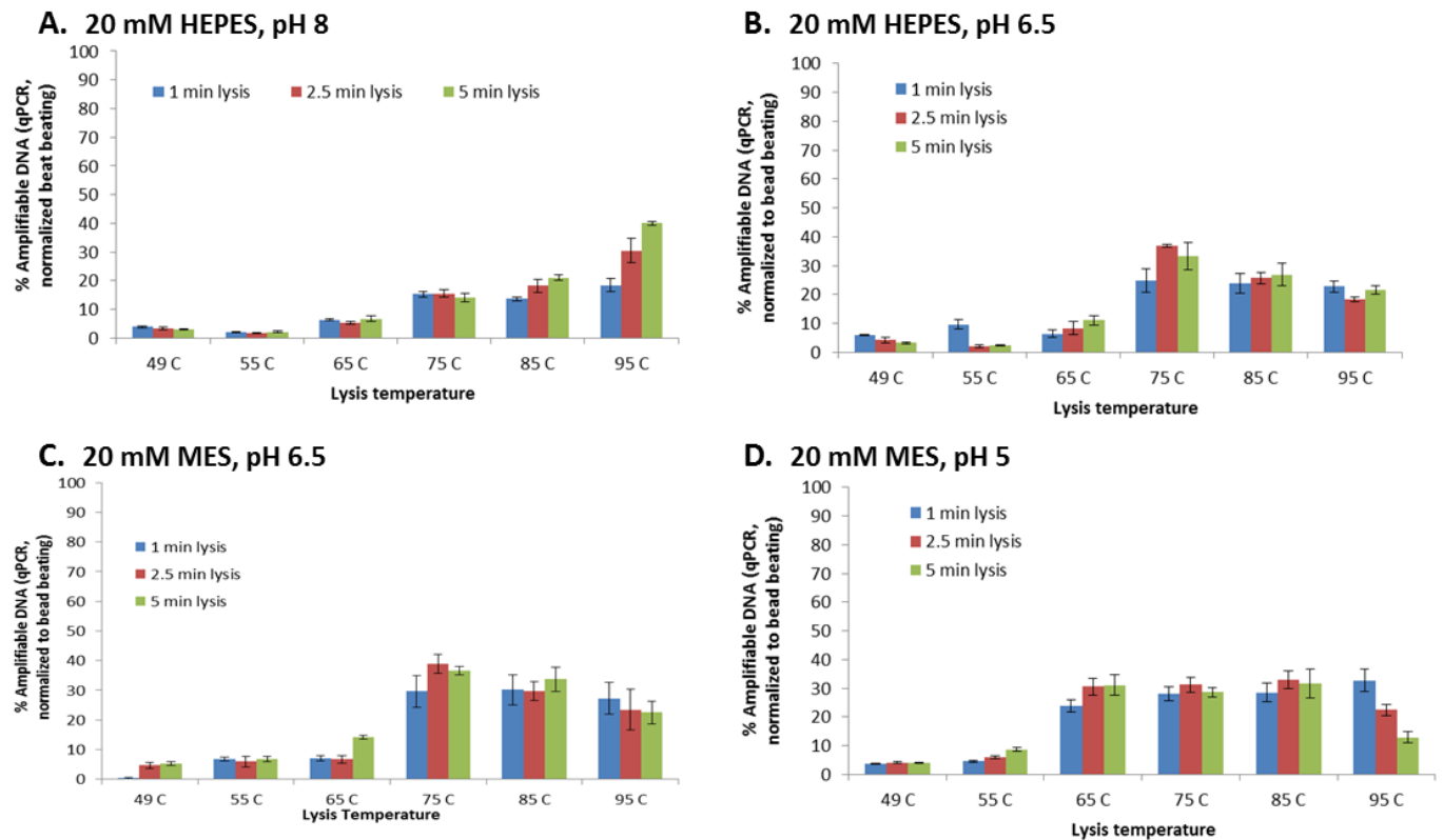
Figure 15. Comparing the effects of pH, temperature, and time on thermal lysis of E. coli . The average of N=3 \pm one standard deviation is reported for each condition. A. 20 mM HEPES at pH 8. B. 20 mM HEPES at pH 6.5. C. 20 mM MES at pH 6.5. D. 20 mM MES at pH 5.
