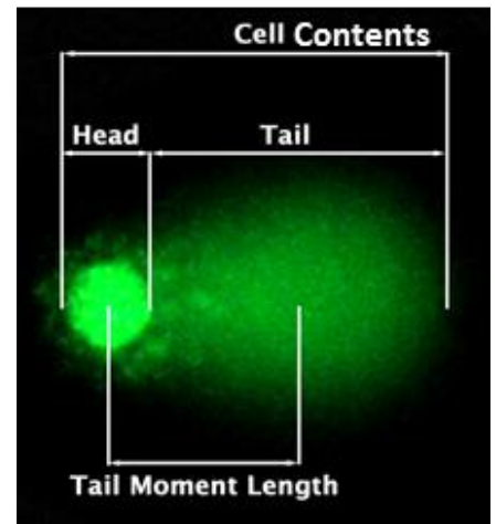
Figure 28. Example of the COMET assay for visualizing DNA fragmentation 193 .
