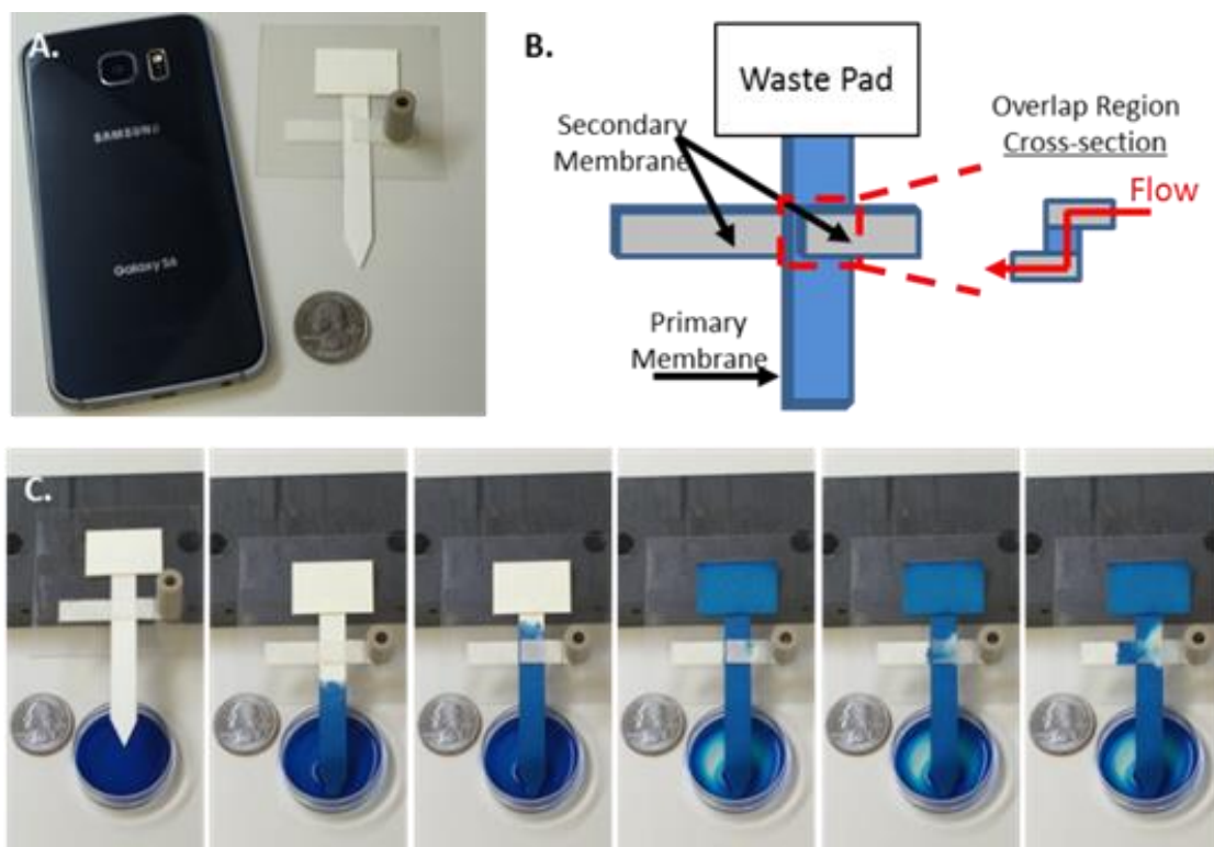
Figure 72. P-switch: pressure-controlled flow through multi-material networks. A. Device imaged next to a Samsung Galaxy S6 mobile phone and US quarter for scale. B. Schematic of the device using a multi-material network. The primary membrane is sandwiched and making contact with the two halves of the secondary membrane as shown in the cross-section. C.
