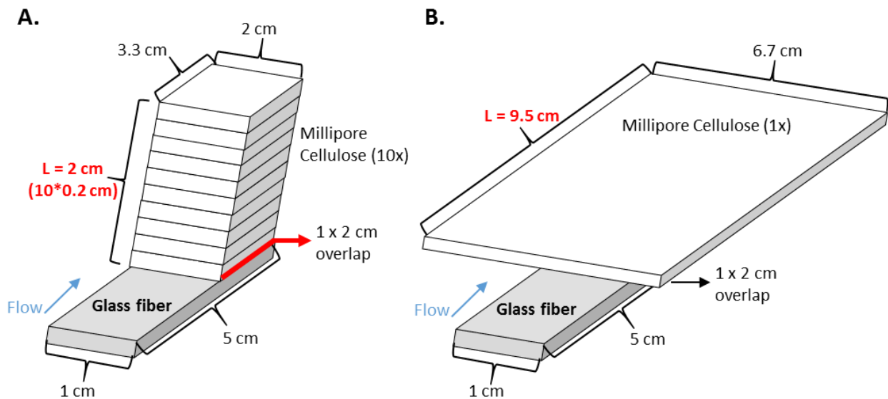
Figure 73. Schematic of waste pad configurations for large volume sample processing experiments. A. Stacked waste pads where L = 2\text{ cm} ( 10 \times 0.2\text{ cm} , thickness of the cellulose membranes). B. Large single waste pad where L = 9.5\text{ cm} .
