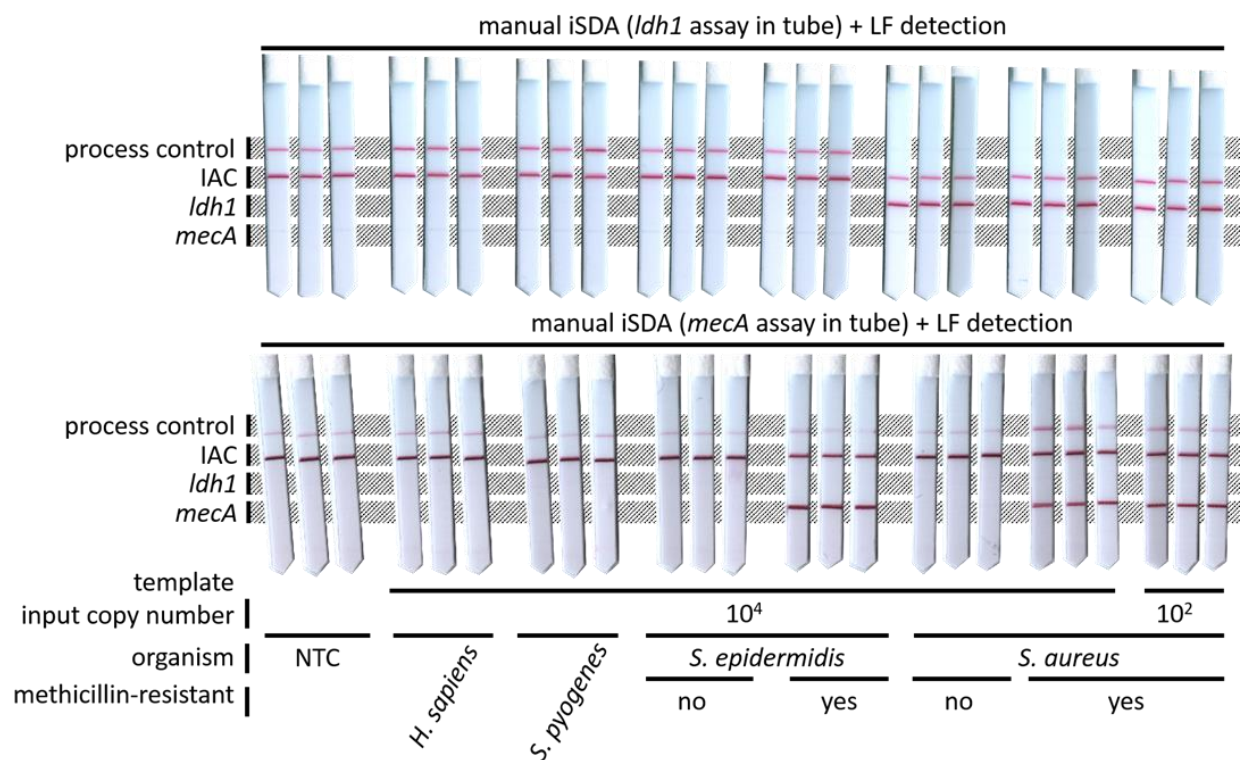
Figure 100: Manual iSDA and LF detection result for (a) Idh1 and (b) mecA assays using no template (NTC); and 10^4 copies of human, S. pyogenes , methicillin-sensitive S. epidermidis (MSSE), methicillin-resistant S. epidermidis (MRSE), methicillin-sensitive S. aureus (MSSA), and methicillin-resistant S. aureus (MRSA) gDNA templates (left-to-right). Amplifications were performed in tubes. The results were mixed with salt and Tween-20 in PBS to final concentrations of 600 mM and 1% w/v, respectively, then allowed to flow on LF strips. The strips shown are the last each of a set of two Idh1 and six mecA experiments. The previous experiments showed low-level signal on all nominally negative test lines, including in the NTC condition, and occasional IAC drop-outs in negative tests, which indicated invalid results. These errors were eliminated through use of new stocks of gold nanoparticles and IAC template, respectively. Across the 120 nominally negative conditions tested in the entire set of eight experiments, one NTC and one S. pyogenes template yielded a strong false positive, which may be indicative of contamination from five years of running these amplification assays in a single laboratory and open handling of amplicons for lateral flow detection and gel analysis.
