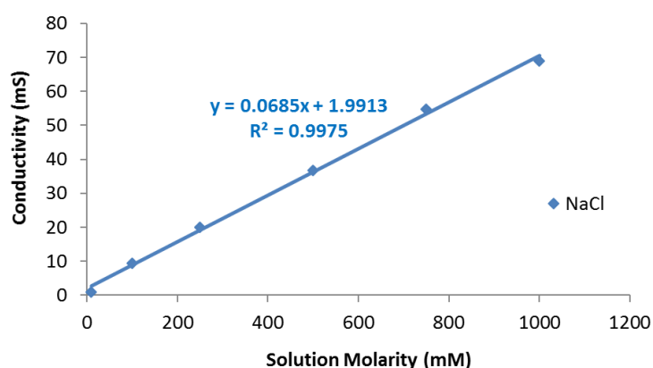
Figure 8. Standard curve to determine the salinity of patient urine samples.
