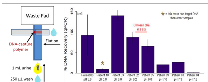
Figure 4. Application of the p-switch for in-membrane DNA purification and concentrated from 1 mL of discarded human urine samples. The primary membrane was patterned with a DNA-capture polymer. Flow of the 1 mL urine sample through primary the membrane resulted in DNA captured by the polymer in the at the membrane junction. After a wash step through the primary membrane, an elution buffer was introduced to the secondary membrane causing the DNA to flow through the junction and into the elution region. Sample recovery was quantified with qPCR. Averages of N=3 are reported with error bars representing +/- one standard deviation. Generally, as sample pH increased, recovery of target DNA decreased.
