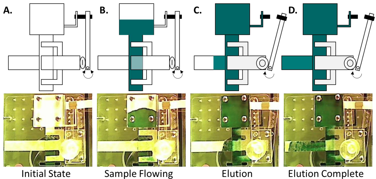
Figure 75. Automating the p-switch for the large volume sample concentration: schematic and image from a video of the device. A. Before sample has reached the waste pad. B. Initially, the elution buffer well is full, but the tubing connecting the well to the secondary network is pinched closed. The sample flows through the primary network into the waste pad. C. When the waste pad reaches a sufficient level of saturation, the activation leg wets a water-soluble membrane (black), which dissolves and breaks causing the pinch on the elution tube to be released. D. When the pinch is released, the elution buffer flows through the junction and fills the secondary network.
