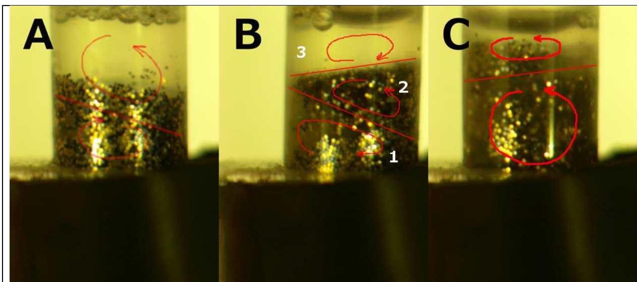
Figure 132: Comparing flow regimes with varied percent glycerol. Tube contains \frac{1}{4} " magnet, 250 mg of 0.1 mm glass beads, deionized H_2O , 0.1% micro 90, glitter, and a variable amount of glycerol. Glitter allows visualization of movement in the largely bead-free upper fluid zone. A: 0% glycerol. Bead slurry geometry and vortex regime in
