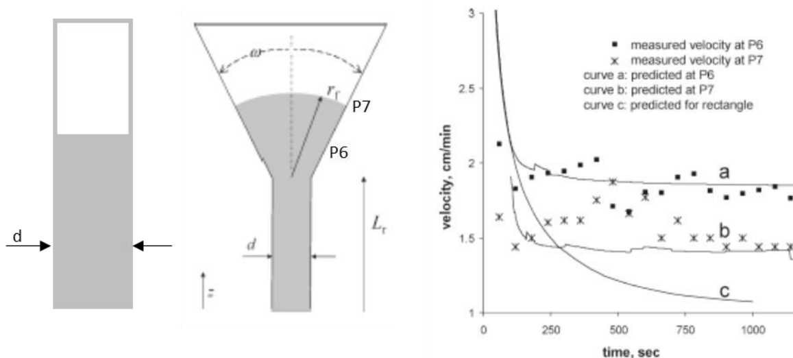
Figure 68. Models and experiments predicting flow through porous membranes. Wet-out of the standard rectangular membrane shows decreased velocity with increasing length and time. The modified geometry of the fan-shaped membrane increases the cross sectional area while decreasing the length required for fluid to travel leading to nearly constant flow rate through the rectangular section of the membrane. Modified from Mendez et al. 276
