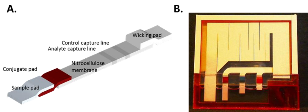
Figure 3. Examples of paper-based devices for POC diagnostics. A. One-dimensional lateral flow test, similar in format to the common pregnancy test. B. Two-dimensional paper network developed in the Yager laboratory for more sophisticated reactions 47 .
