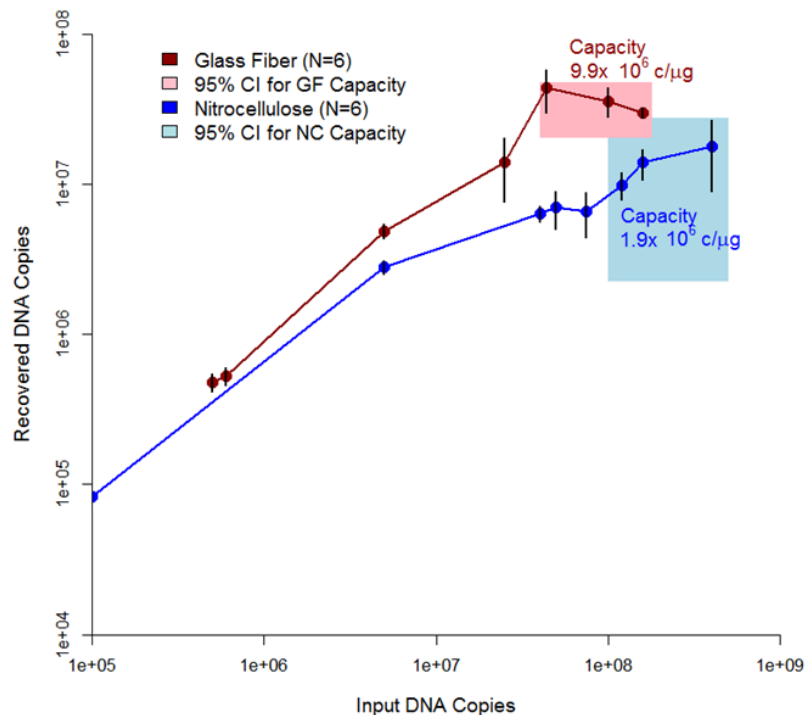
Figure 52. Capacity of chitosan for DNA in nitrocellulose and glass fiber over a range of input concentrations (N=6 for each point) after normalization for membrane surface area. The capacity of chitosan for DNA is 1.9 \times 10^6 \text{c}/\mu\text{g} (95% CI: 2.9 \times 10^5 to 3.5 \times 10^6 \text{c}/\mu\text{g} ) in nitrocellulose and 9.9 \times 10^6 \text{c}/\mu\text{g} (95% CI: 5.9 \times 10^6 to 1.4 \times 10^7 \text{c}/\mu\text{g} ) in glass fiber.
