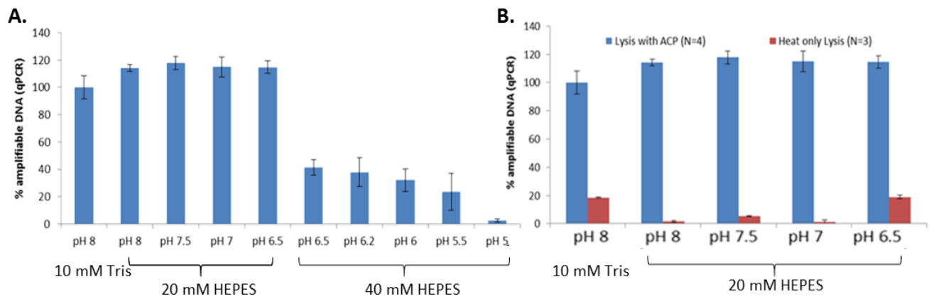
Figure 9. Effect of pH on ACP activity for bacterial lysis. Results were normalized to samples treated by bead beating. An average of at least N=3 \pm one standard deviation is reported for each condition. A. Testing a range of buffers and pH values. B. Samples lysed in the presence of ACP compared to samples lysed with only heat.
