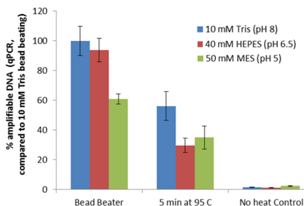
Figure 13. Effect of buffers on E. coli lysis methods. An average of N=4 \pm one standard deviation is presented for each condition.
