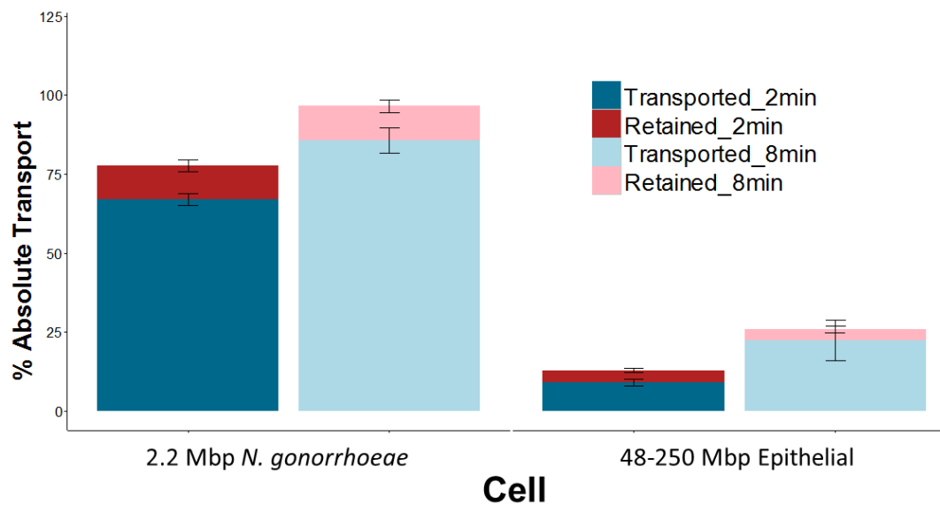
Figure 45. Fragmentation and transport of mixed samples through porous membranes. The epithelial cell does not lyse as effectively as the small bacterial cell in these conditions, therefore reducing the amount of DNA available for fragmentation. For both heating times tested, 4x more N. gonorrhoeae DNA successfully transported through the membrane compared to epithelial cell DNA. Averages of N=6 (N=3 from two independent cultures) are reported with error bars representing standard error. Samples were treated with ACP for 2 minutes at room temperature followed by heating to 95° for either 2 or 8 minutes.
