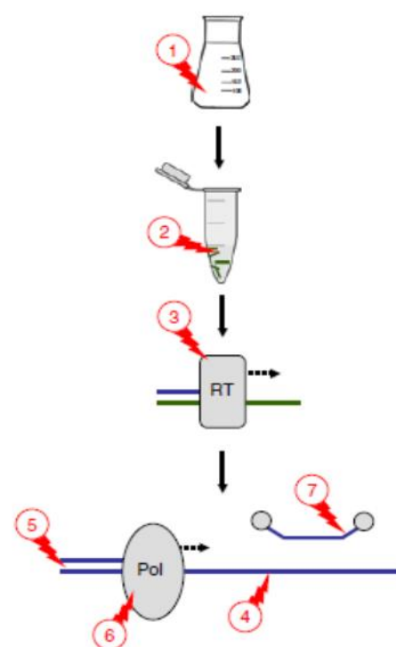
Figure 88. Methods of PCR inhibition. NA may react with the reaction vessel (1) or contaminants may be introduced during sample processing (2). Inhibitors may prevent reverse transcription (RT) for RNA-based assays (3) or degrade the NA template (4). Primer annealing (5) or polymerase (6) may be degraded or blocked. The probes for detection may also be inhibited (7) 266 .
