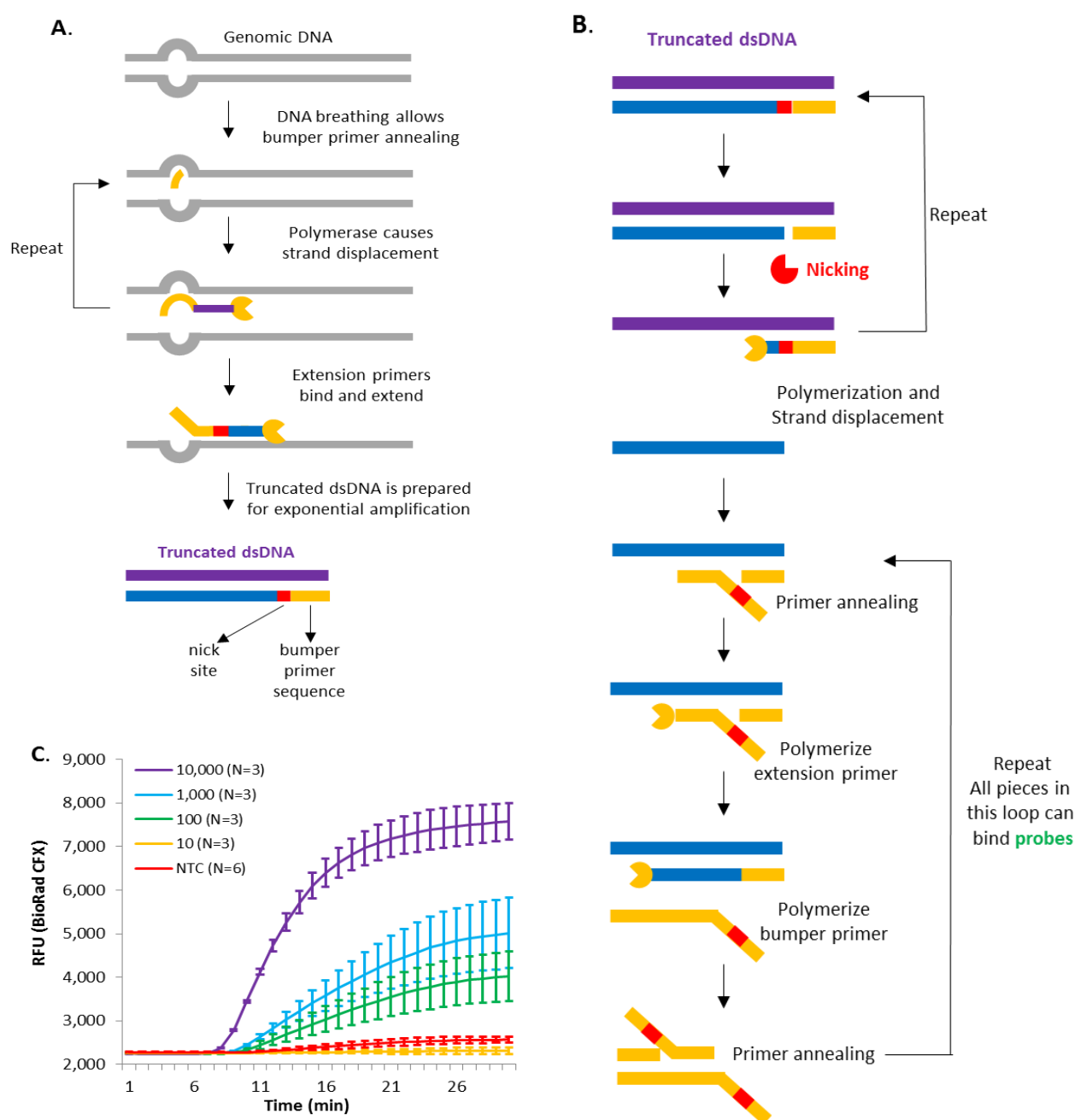
Figure 91. Summary of iSDA mechanism. A. Schematic of the linear phase of iSDA and the B. exponential phase, adapted from Dr. Joshua Bishop and Dr. Bhushan Toley. C. Example of real
