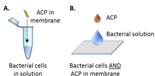
Figure 22. ACP treatment for bacterial lysis.
