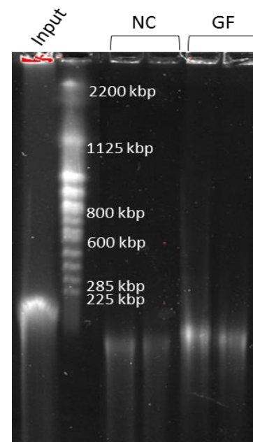
Figure 32. PFGE to determine range of fragment sizes that flowed through nitrocellulose (NC) and glass fiber (GF) membranes.
