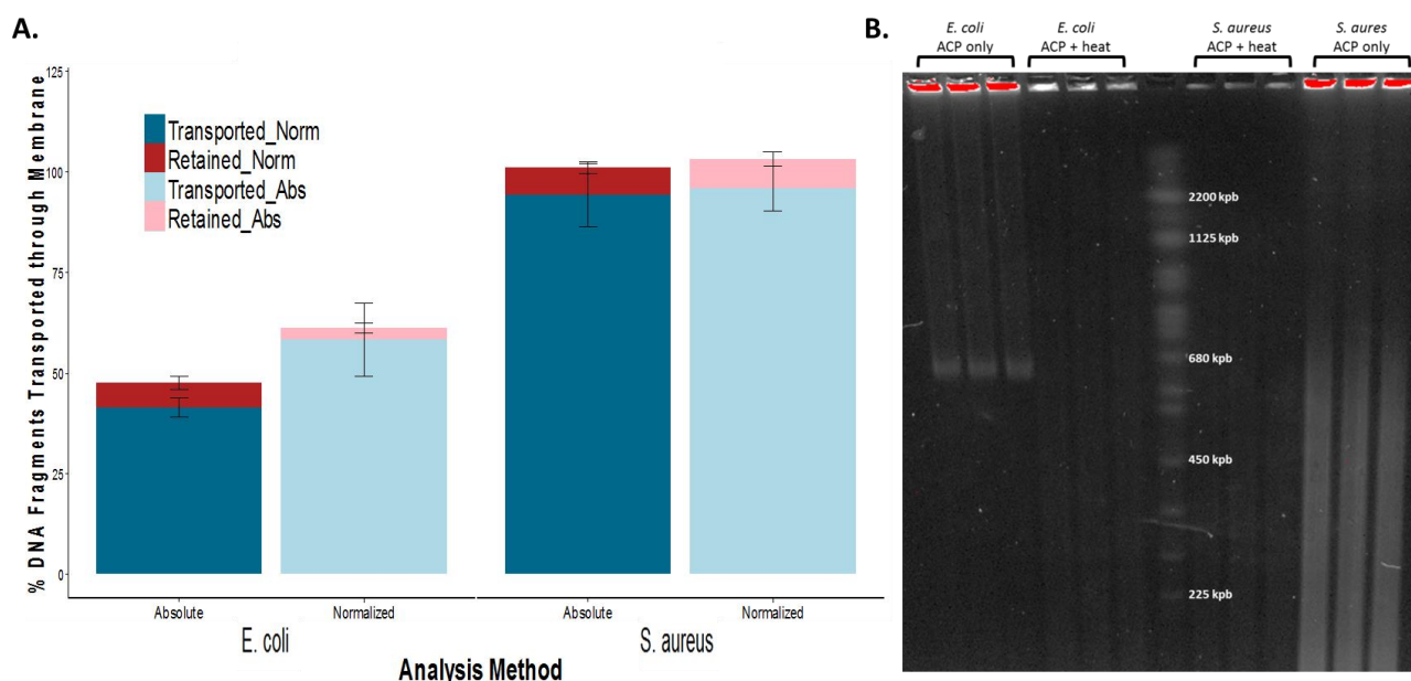
Figure 33. Methods for analyzing thermal gDNA fragmentation and transport through porous membranes using E. coli and S. aureus pathogens. A. Comparing two quantitative measurements of transport: Percent Absolute Transport (Absolute) and Percent Normalized Transport (Normalized). For this data, the lysis efficiencies for both pathogens were ~100% so the two transport quantification methods showed the same results. These data were collected using Fusion 5 membranes. Averages of N=6 (N=3 from two separate cultures) are reported with error bars representing standard error. B. PFGE comparing “ACP only” and “ACP + heat” lysis samples. Under these treatment conditions, the average size of S. aureus DNA fragments is smaller than the E. coli DNA fragments because some large fragment E. coli DNA remained in the wells while the S. aureus -containing “ACP + heat” wells had no visible DNA. Note that the red color of the wells in the upper part of the gel are saturated pixels, indicating the presence of very high concentrations of DNA.
