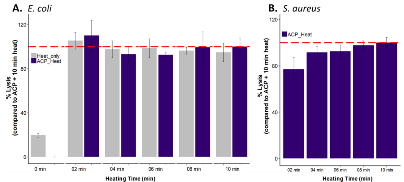
Figure 37. Lysis efficiencies for various methods and heating times at 95°C. Treatment with ACP + 10 minutes of heating was set to 100% (dashed red line) for each pathogen tested. In general, lysis efficiencies were similar for each condition. Samples treated with ACP could not have a 0 min heat condition because the non-denatured enzyme inhibits qPCR. The average of N=6 (N=3 from two independent cultures) is reported with the error bars representing standard error. A. E. coli treated with and without ACP, and B. MRSA treated with ACP.
