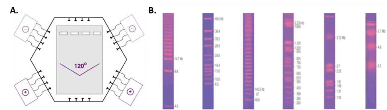
Figure 29. Pulsed field gel electrophoresis. A. Schematic 205 . B. Range of PFGE ladders 206 .
