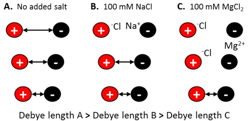
Figure 61. Effect of increasing ionic strength and ion valence on Debye length of electrostatic interactions. Charge species represented by "+" and "-" connected by arrows are successfully interacting. Increasing the quantity or valence of ions decreases the Debye length causing charged species that are further away to no longer interact as indicated by the loss of connecting arrows.
