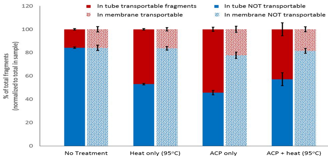
Figure 46. Comparing fragmentation methods of E. coli gDNA in tube and in membrane. Fragmentation is significantly reduced when cells are treated in a glass fiber membrane compared to in a tube. Averages of N=3 \pm one standard deviation are presented.
