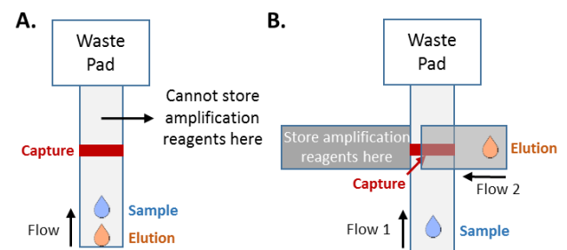
Figure 74. Schematic of A. linear purification and B. purification with controlled fluid flow.
