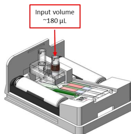
Figure 5. Current MAD NAAT device for small volumes (~180 \mu L).
