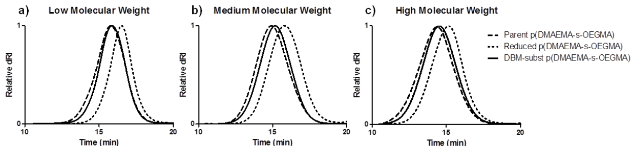
Figure 1.2 SEC traces of (a) low, (b) medium, and (c) high molecular weight parent, reduced, and DBM-substituted DMAEMA and OEGMA copolymers. Parent polymers were reduced with TCEP (right-shifted trace) and resulting thiolated polymer fragments were substituted to DBM-alkyne (overlapping trace with parent polymer).
