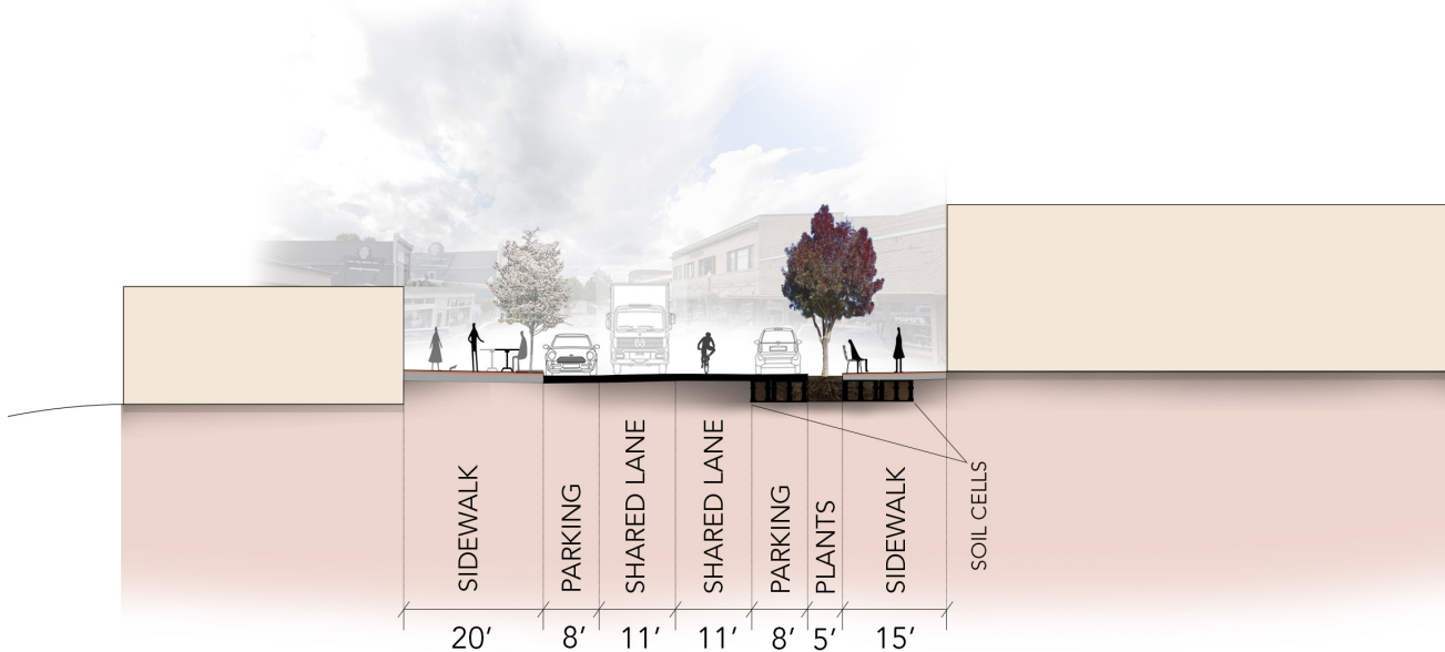
STREET SECTION: PROPOSED
