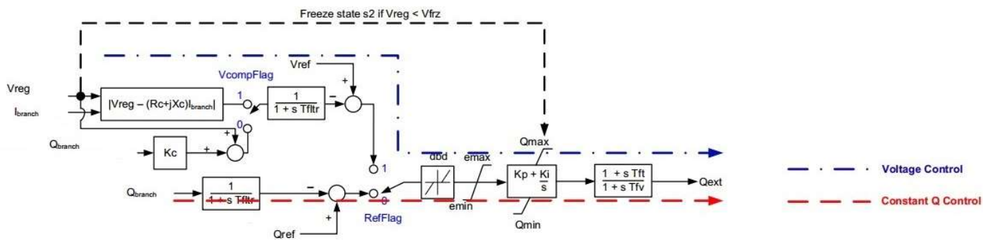
Figure A3: REPC_A reactive power control block diagram [28]
