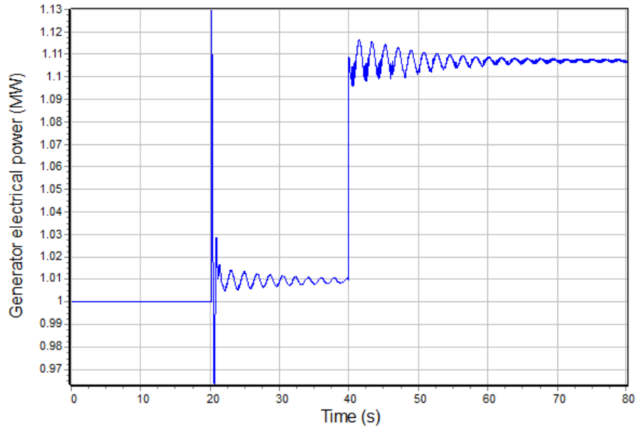
Figure 15: Existing system with default exciter settings & governor T_3 = 1 s
