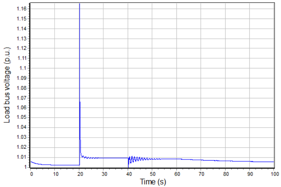
Figure 25: Load bus voltage, BESS internal voltage > 1.0 p.u. (simulation 3)
