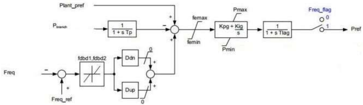
Figure 13: REPC_A active power control block diagram [20]
