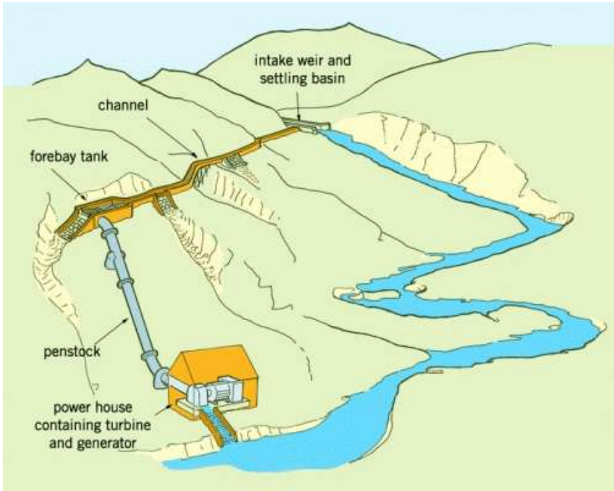
Figure 3: Example small-scale run-of-river hydroelectric system [5]
