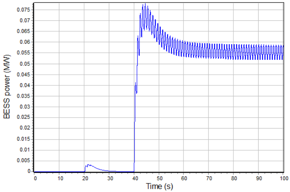
Figure B3: BESS output power with BESS K_{pg} = 3
