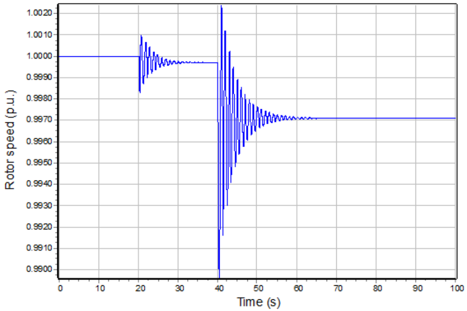
Figure 27: Generator rotor speed, 1.5 MW base load (simulation 5)
