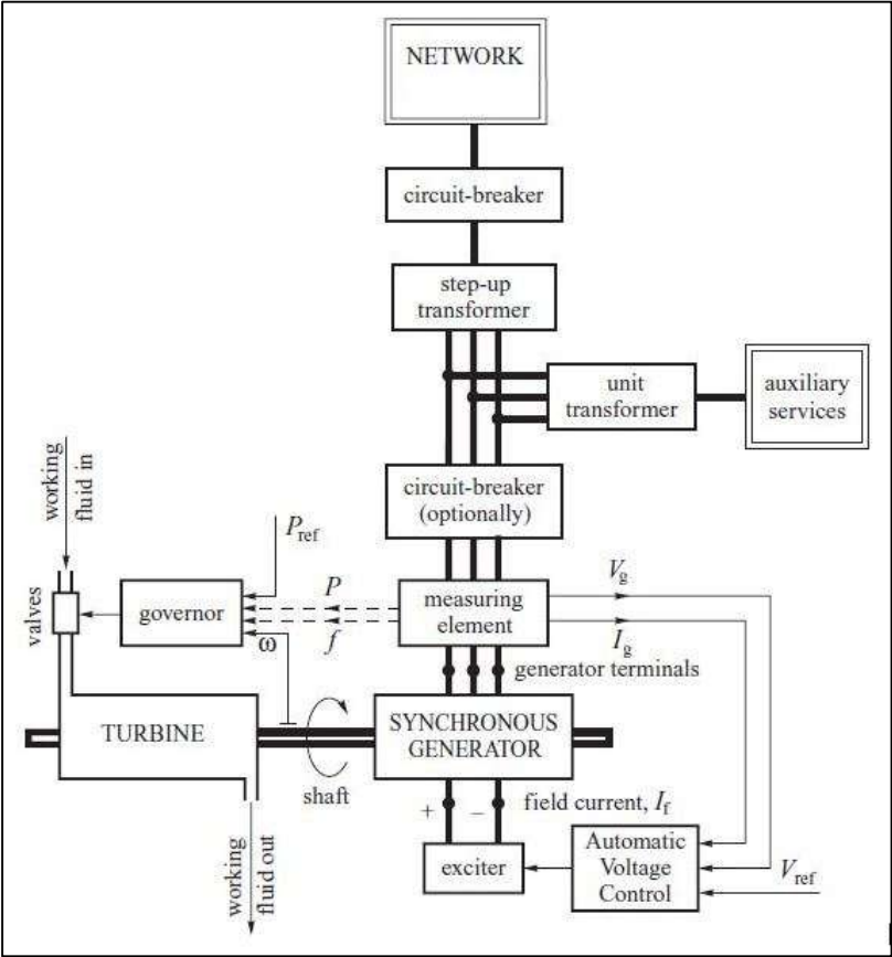
Figure 8: Power generation system block diagram [11]
