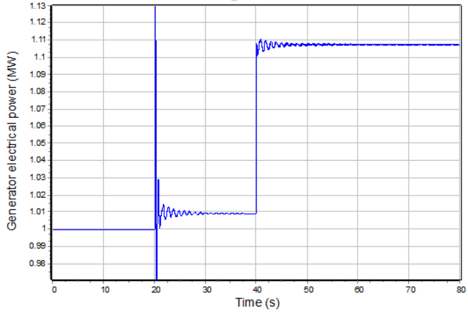
Figure 16: Existing system with default exciter settings & governor T_3 = 0.25 s
