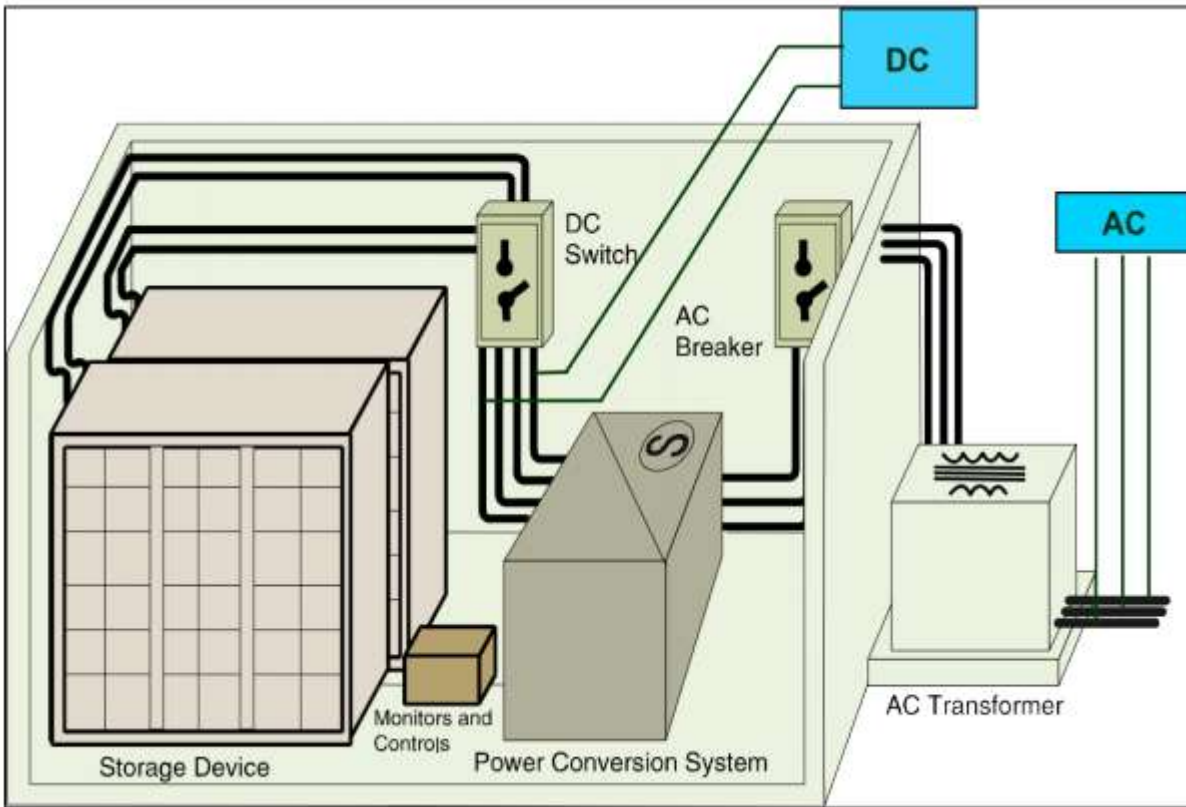
Figure 2: Battery energy storage system schematic [1]
