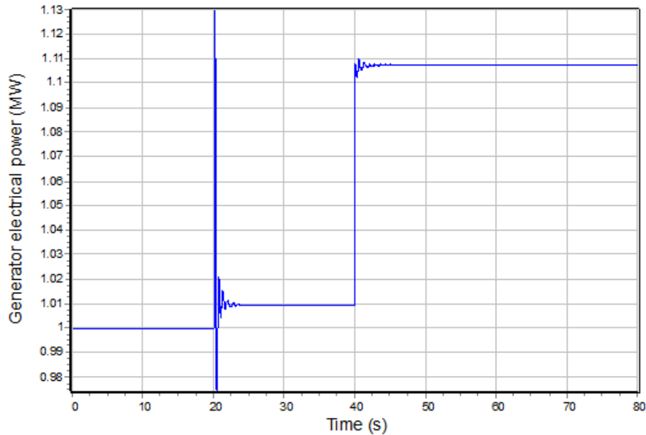
Figure 14: Existing system with default exciter & governor settings ( T_3 = 0.1 s)
