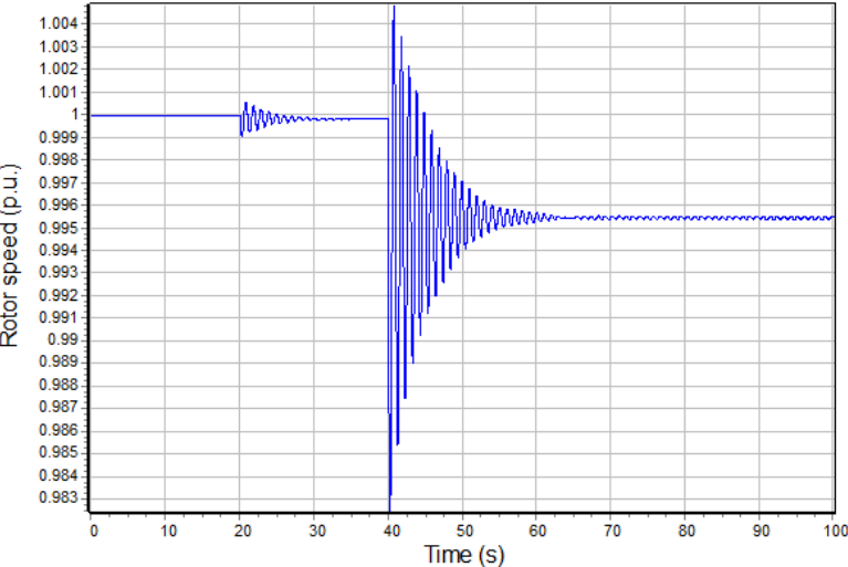
Figure 23: Generator rotor speed, 25% load increase (simulation 2)
