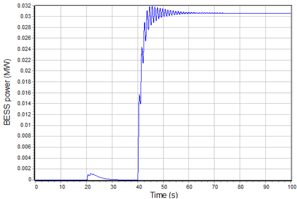
Figure 20: BESS output with BESS K_{pg} = 1
