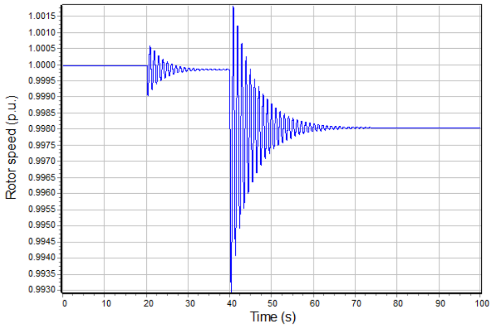
Figure 19: Generator rotor speed with BESS K_{pg} = 1
