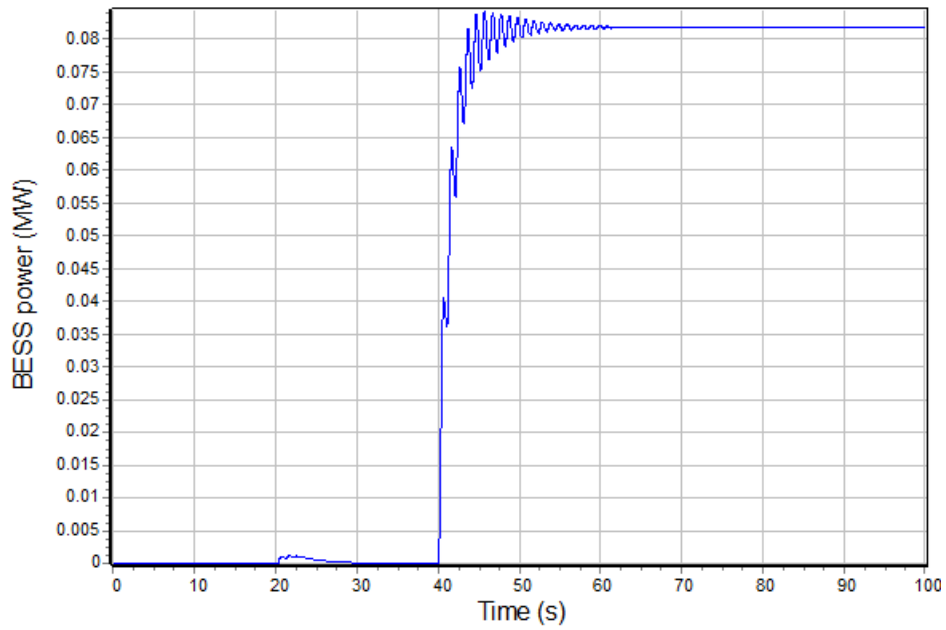
Figure B4: BESS power, 25% load increase (simulation 2)
