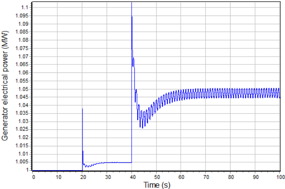
Figure B1: Generator electrical power output with BESS K_{pg} = 3
