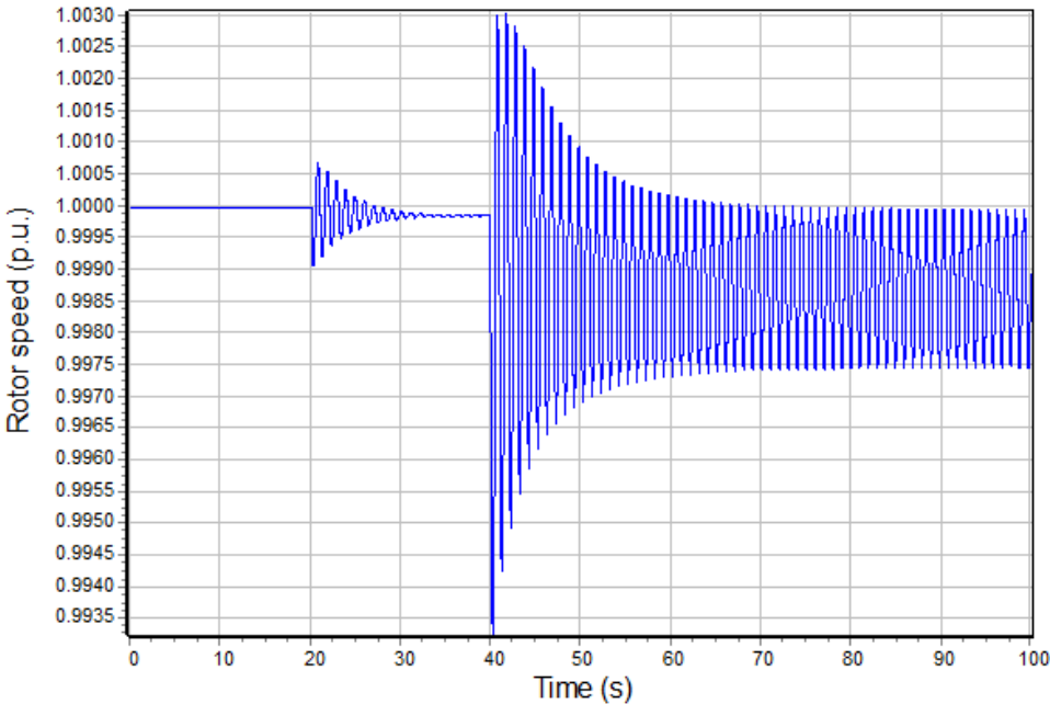
Figure B2: Generator rotor speed with BESS K_{pg} = 3
