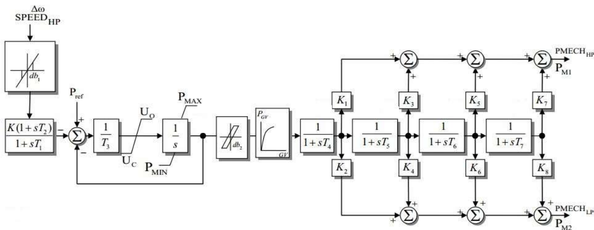
Figure 11: IEEE G1 block diagram [20]
