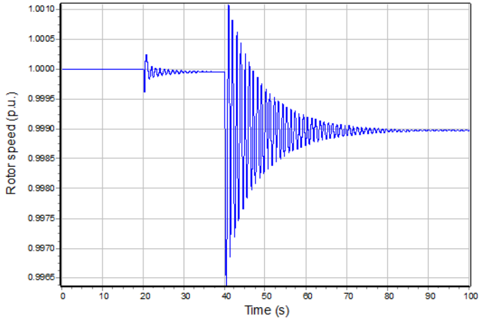
Figure 26: Generator rotor speed, 0.5 MW base load (simulation 4)
