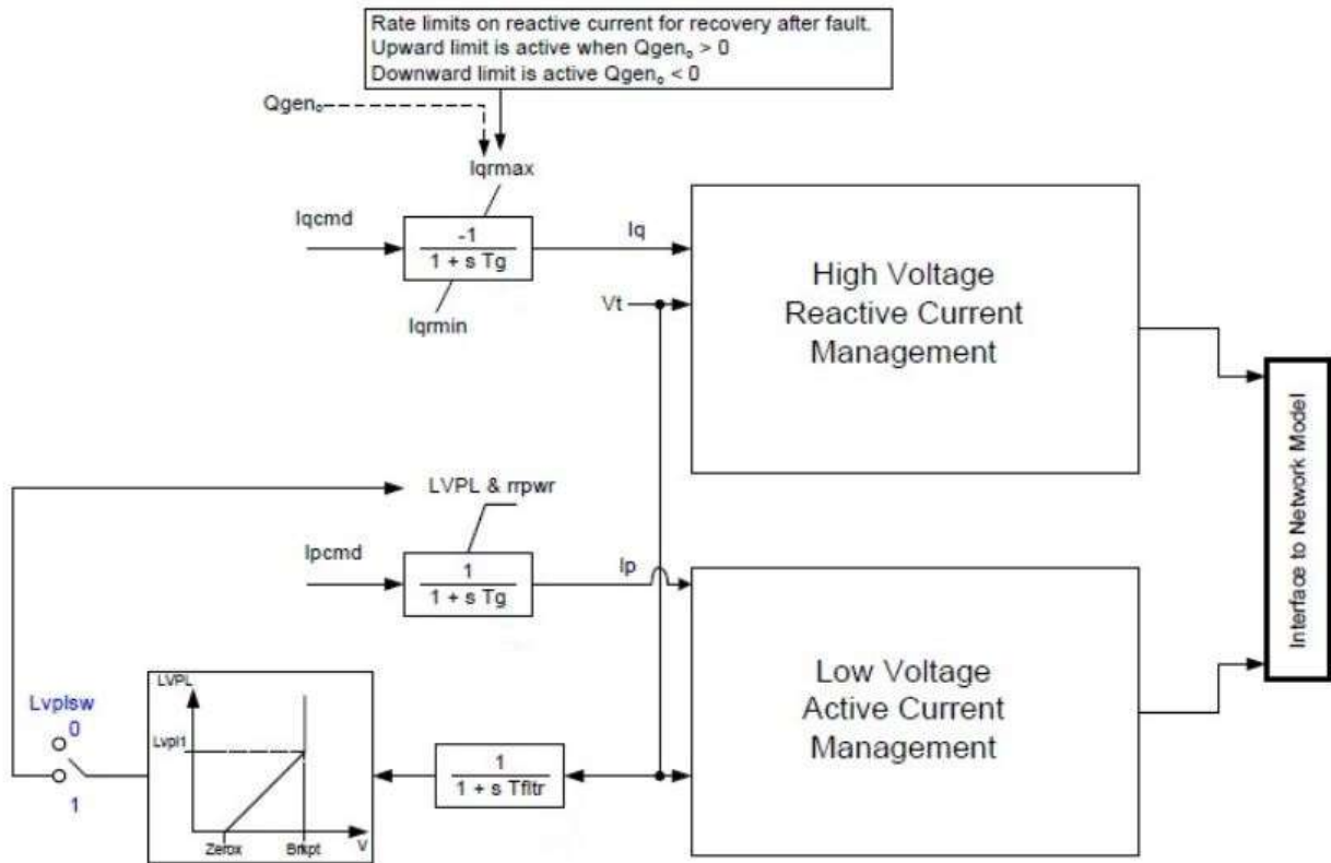
Figure A1: REGC_A block diagram [20]
