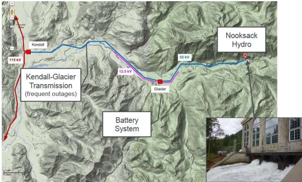
Figure 6: Map of proposed microgrid in Glacier, WA [17]
