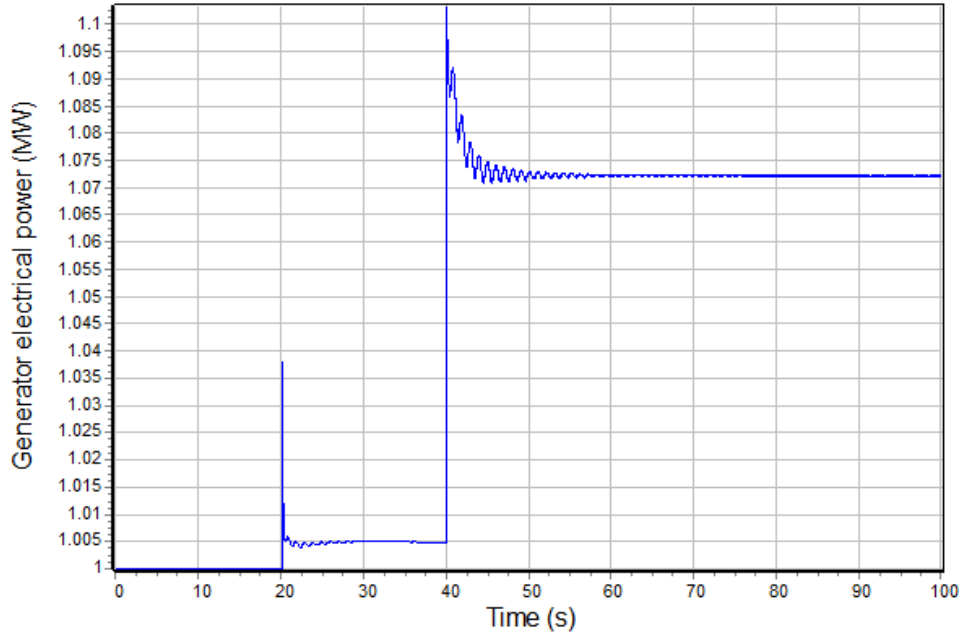
Figure 18: Generator electrical power output with BESS K_{pg} = 1
