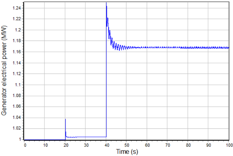
Figure 22: Generator electrical power output, 25% load increase (simulation 2)
