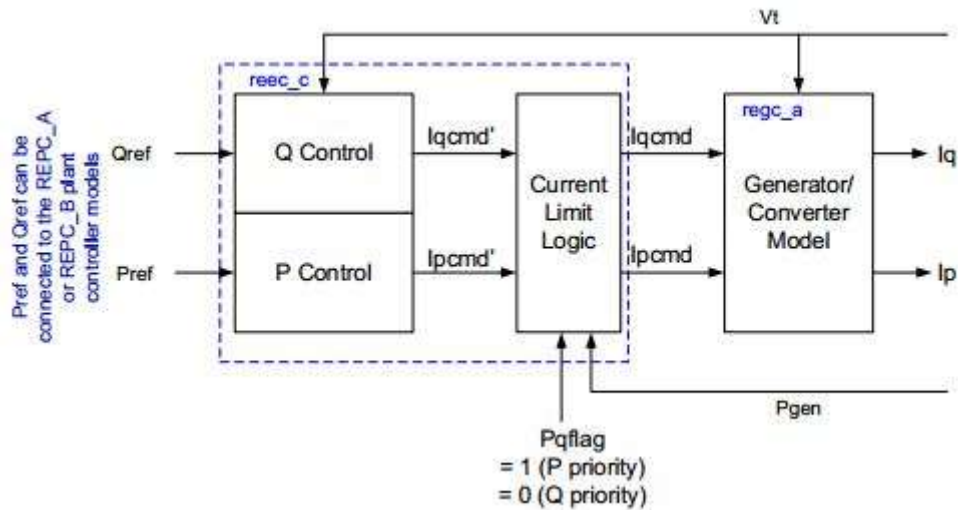
Figure 12: Simple BESS model [26]
