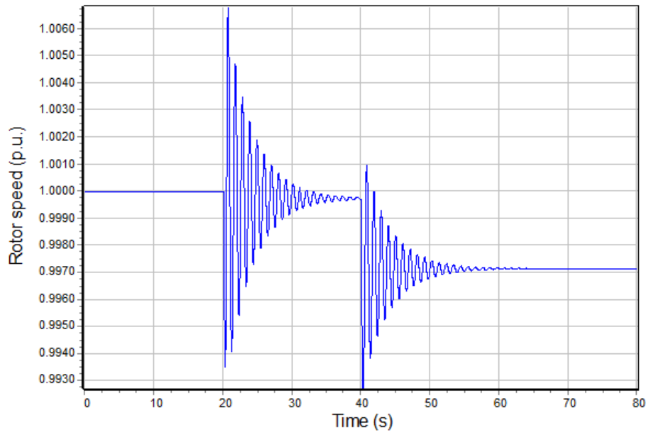
Figure 17: Generator speed with default exciter settings & governor T_3 = 0.25 s
