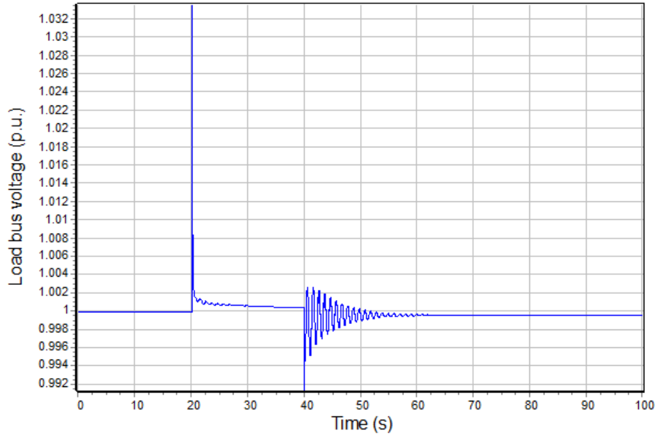
Figure 24: Load bus voltage, BESS internal voltage is 1.0 p.u. (simulation 2)
