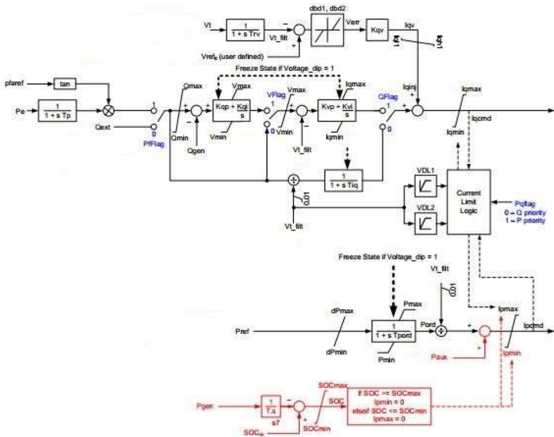
Figure A2: REEC_C block diagram [28]
