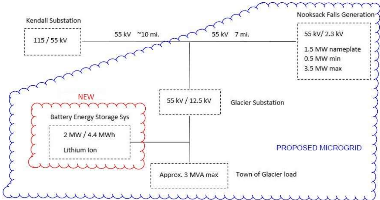
Figure 5: Proposed microgrid in Glacier, WA
