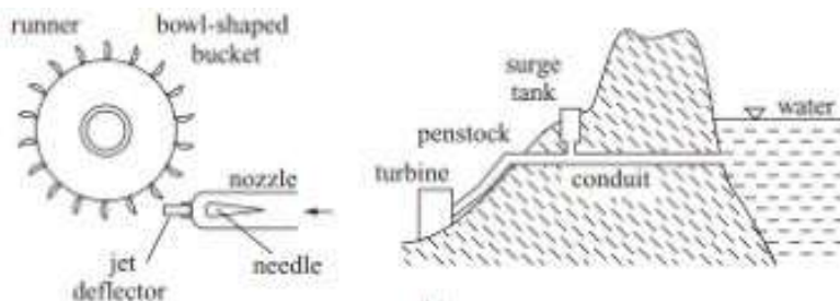
Figure 10: Pelton wheel high-head turbine [11]
