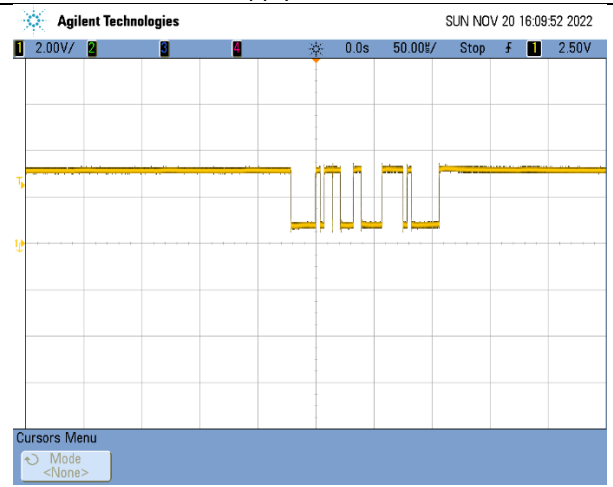
DB9 Connector Pin 6 (SLO+). Shows SLO+ Vhigh \approx 3.2 V, Vlow \approx 0.8 V. Idle state is high.
