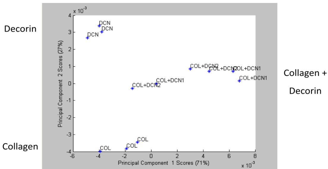
Figure 2.5. PCA Analysis of ToF-SIMS data from coated surfaces. Plot of principal component 1 (PC1) vs. principal component 2 (PC2) shows separation of decorin (DCN), collagen (COL) and collagen + decorin (COL+DCN) surfaces.
